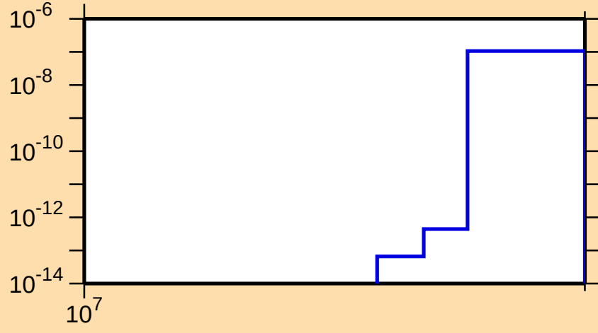
\sigma vs. E for ^{99}\text{Y}(n,\text{nd})
