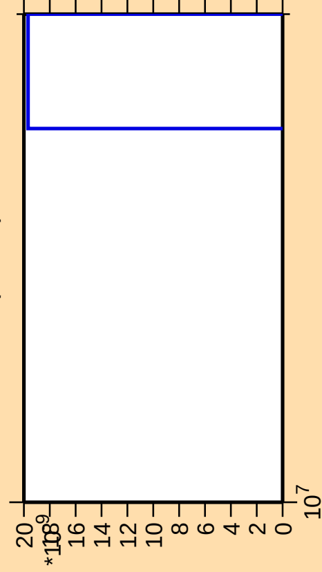
\Delta\sigma/\sigma vs. E for ^{99}\text{Y}(\text{mt } 11)
