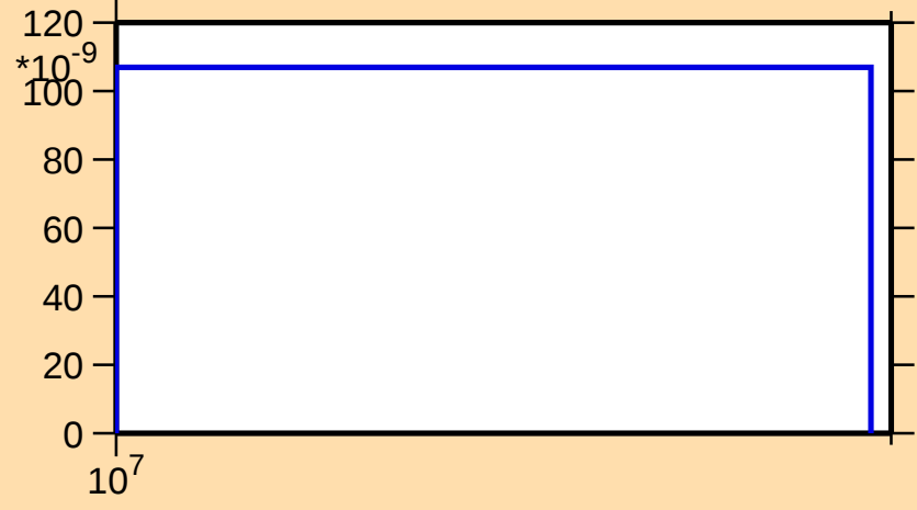
\sigma vs. E for ^{99}\text{Y}(n,nt)
