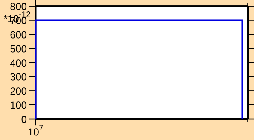
\sigma vs. E for ^{99}\text{Y}(\text{n},\text{nd})
