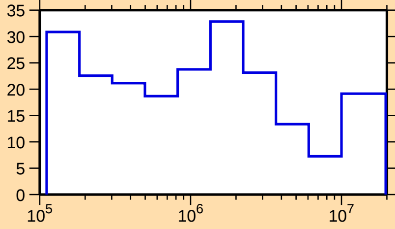
\Delta\sigma/\sigma vs. E for ^{99}\text{Y}(\text{n,el.})
