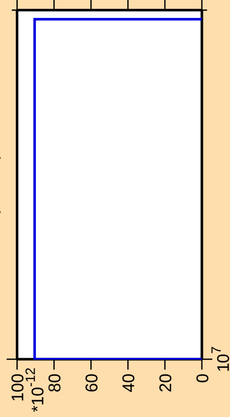
\Delta\sigma/\sigma vs. E for ^{99}\text{Y}(\text{mt } 11)
