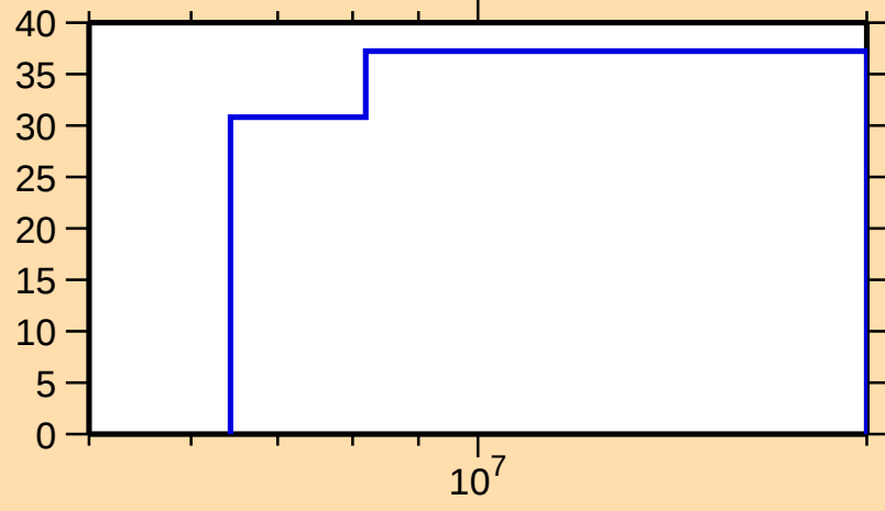
\Delta\sigma/\sigma vs. E for ^{99}\text{Y}(\text{n},\text{inel.})
