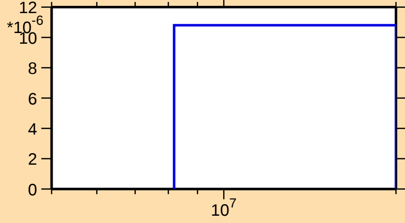
\sigma vs. E for ^{99}\text{Y}(n,np)
