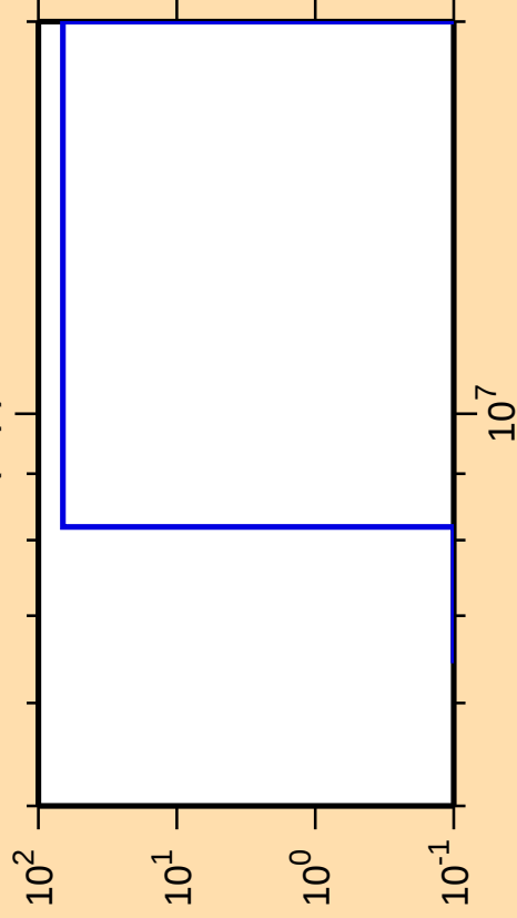
\Delta\sigma/\sigma vs. E for ^{99}\text{Y}(\text{n},\text{p})
