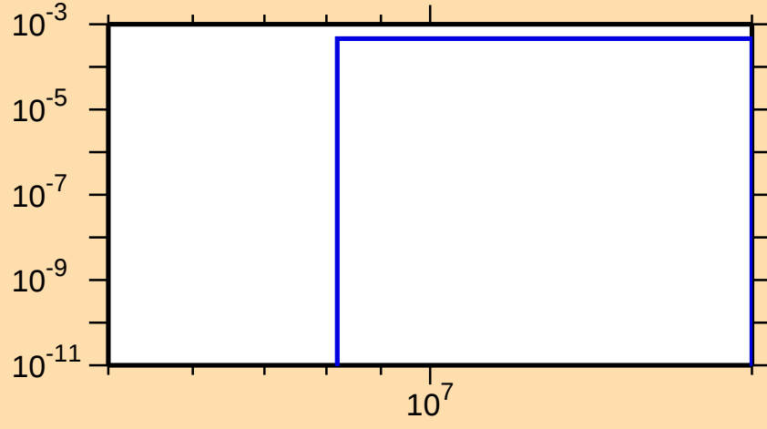
\sigma vs. E for ^{99}\text{Y}(n,p)
