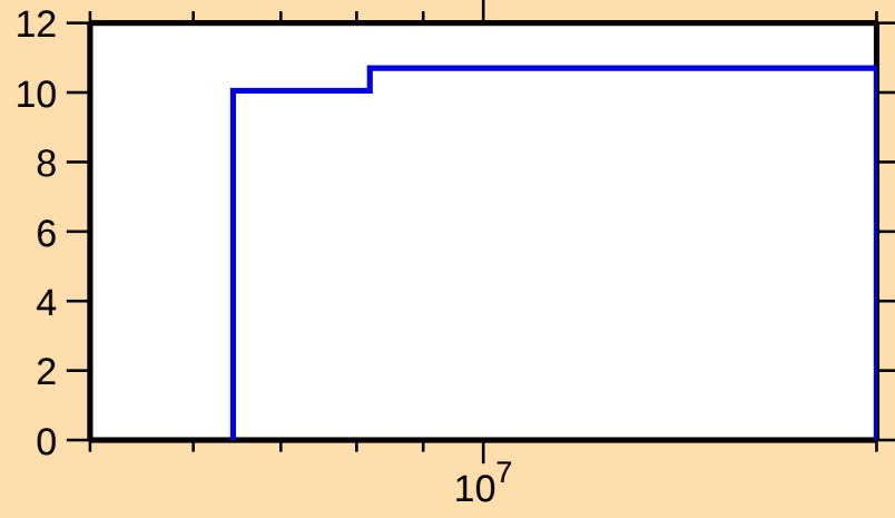
\Delta\sigma/\sigma vs. E for ^{99}\text{Y}(\text{n},\text{nonel.})
