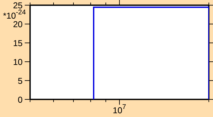
\sigma vs. E for ^{99}\text{Y}(\text{mt 11})
