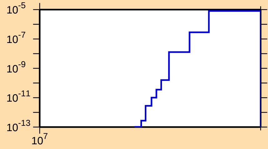
\sigma vs. E for ^{61}\text{Zn}(\text{mt 34})
