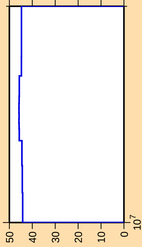
\Delta\sigma/\sigma vs. E for ^{61}\text{Zn}(n,n_1)
