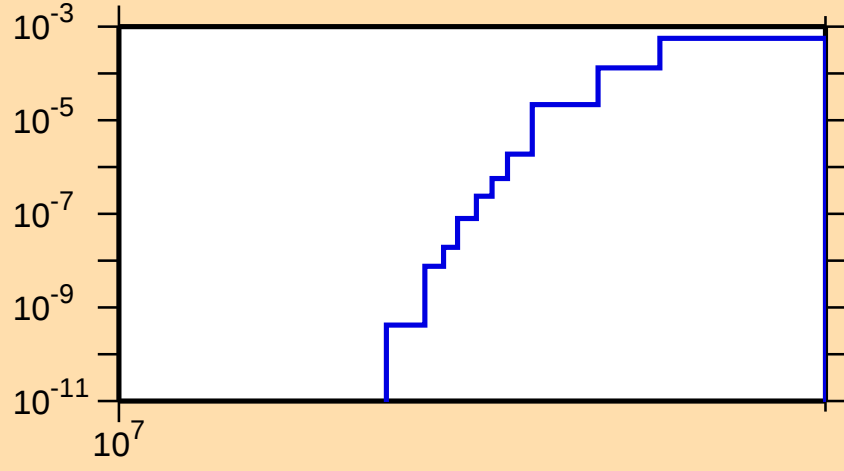
\sigma vs. E for ^{61}\text{Zn}(n,\text{pt})
