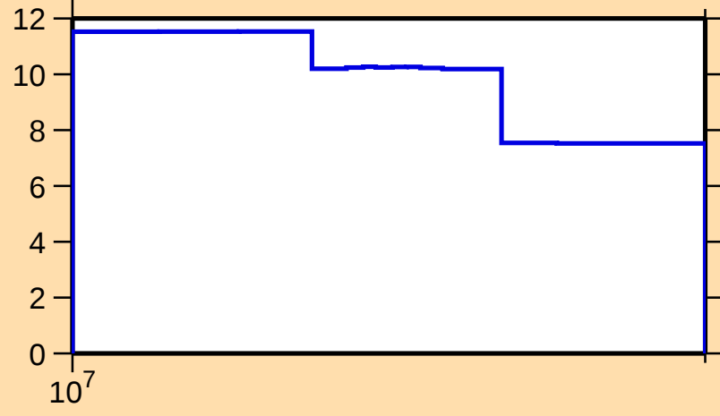
\Delta\sigma/\sigma vs. E for ^{61}\text{Zn}(n,\text{el.})
