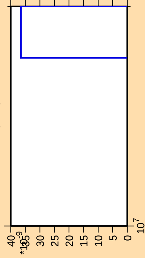
\Delta\sigma/\sigma vs. E for ^{61}\text{Zn}(n,nt)
