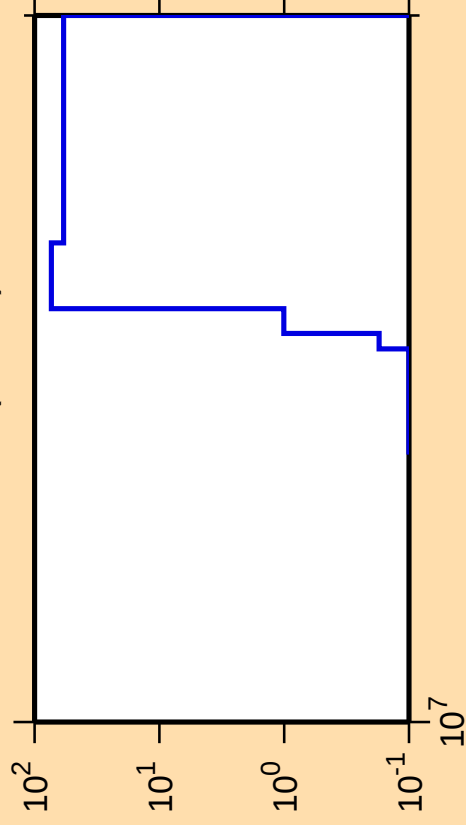
\Delta\sigma/\sigma vs. E for ^{61}\text{Zn}(\text{mt } 45)
