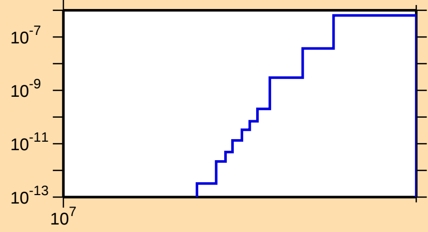
\sigma vs. E for ^{61}\text{Zn}(\text{mt117})
