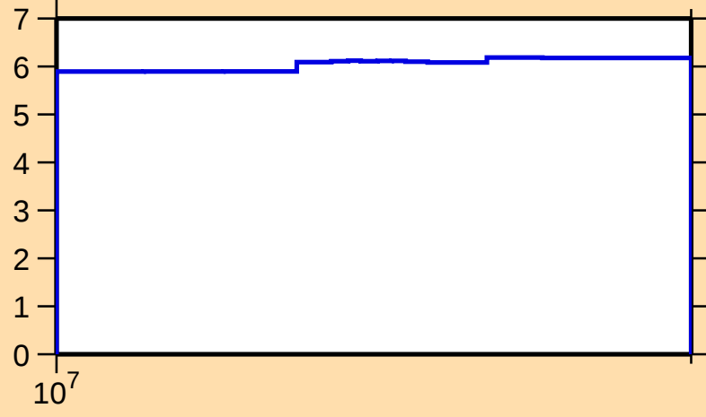
\Delta\sigma/\sigma vs. E for ^{61}\text{Zn}(n,\text{tot.})
