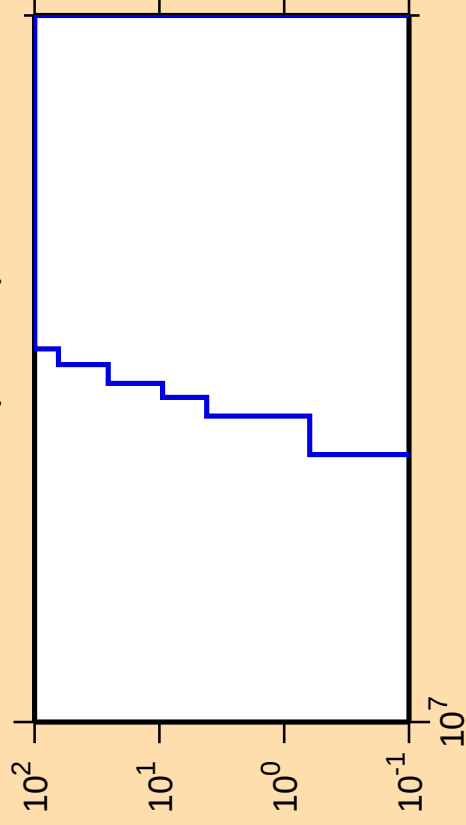
\Delta\sigma/\sigma vs. E for ^{61}\text{Zn}(\text{mt117})
