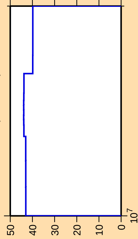
\Delta\sigma/\sigma vs. E for ^{61}\text{Zn}(n,n\text{cont.})
