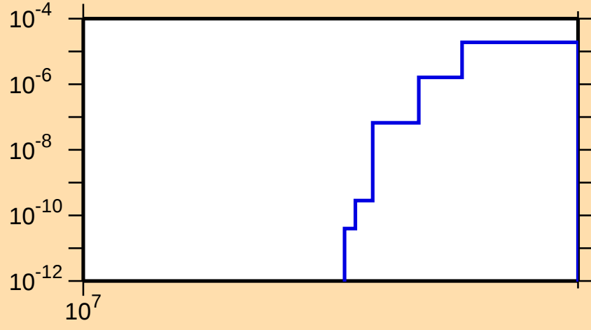
\sigma vs. E for ^{61}\text{Zn}(n,\text{nd})
