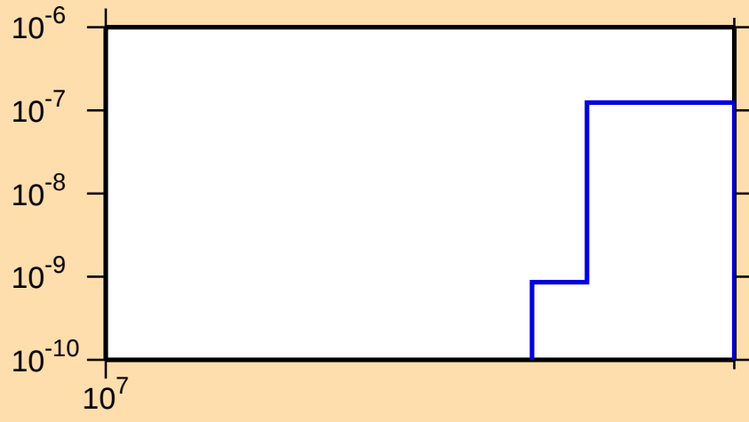
\sigma vs. E for ^{61}\text{Zn}(n,2n\alpha)
