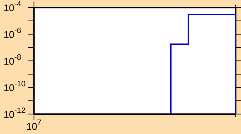
\sigma vs. E for ^{61}\text{Zn}(n,2np)
