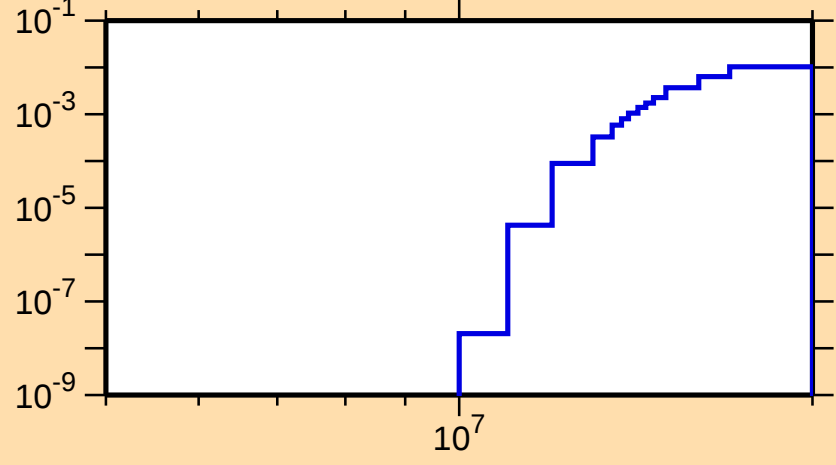
\sigma vs. E for ^{61}\text{Zn}(n,\text{pd})
