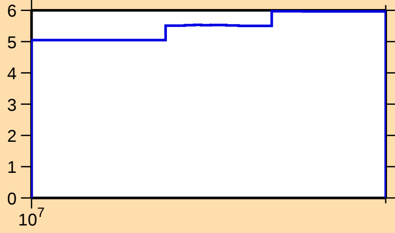
\Delta\sigma/\sigma vs. E for ^{61}\text{Zn}(n,\text{nonel.})
