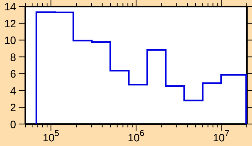
\Delta\sigma/\sigma vs. E for ^{61}\text{Zn}(n,\text{tot.})
