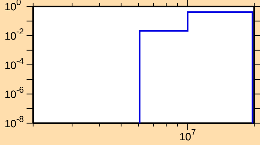
\sigma vs. E for ^{61}\text{Zn}(n,np)
