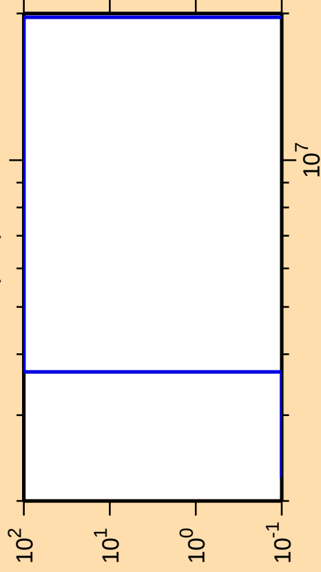
\Delta\sigma/\sigma vs. E for ^{61}\text{Zn}(n,d)
