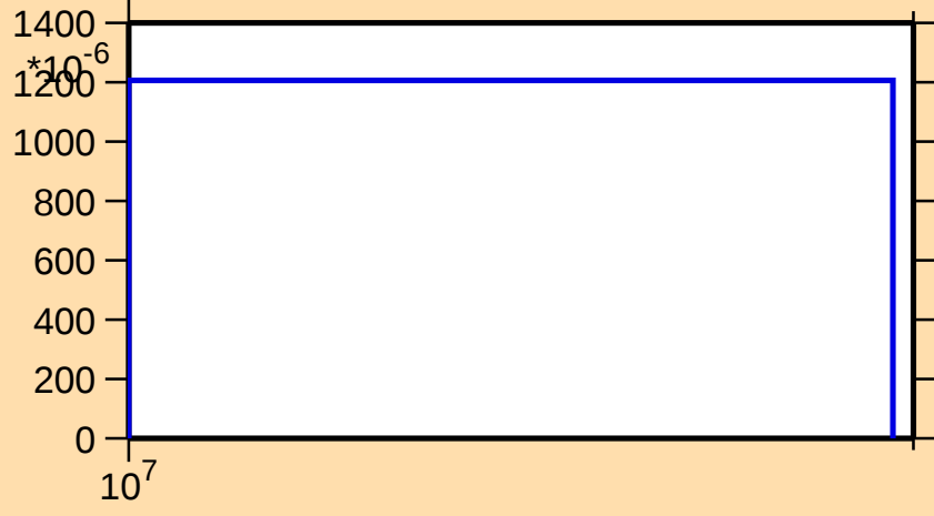
\sigma vs. E for ^{61}\text{Zn}(n,2n)
