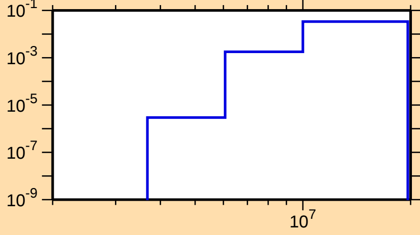
\sigma vs. E for ^{61}\text{Zn}(n,d)
