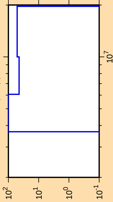
\Delta\sigma/\sigma vs. E for ^{61}\text{Zn}(n,np)
