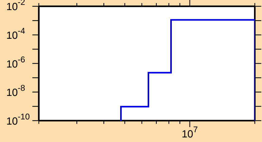
\sigma vs. E for ^{61}\text{Zn}(n,\text{He3})
