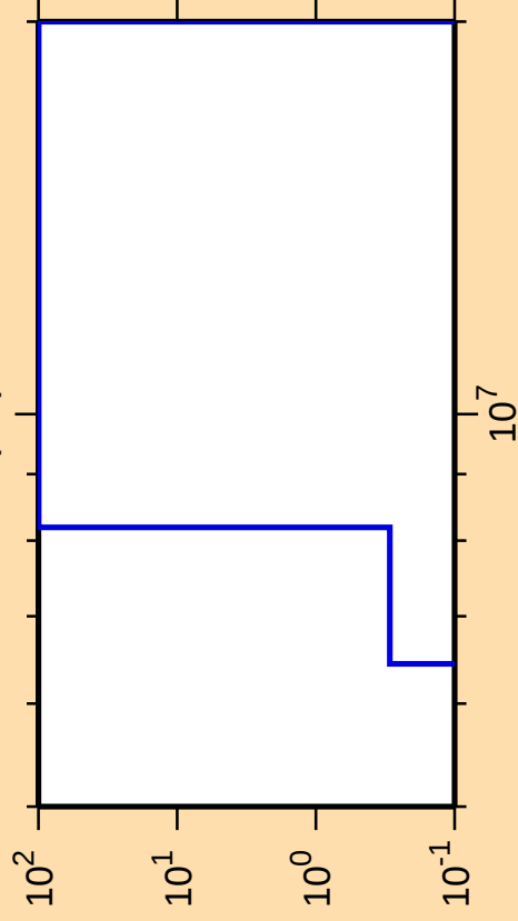
\Delta\sigma/\sigma vs. E for ^{61}\text{Zn}(n,t)
