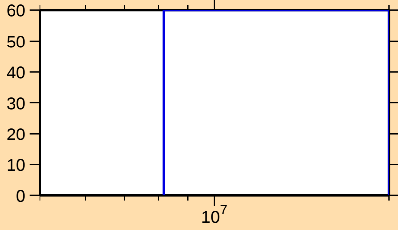
\Delta\sigma/\sigma vs. E for ^{61}\text{Zn}(n,2n)
