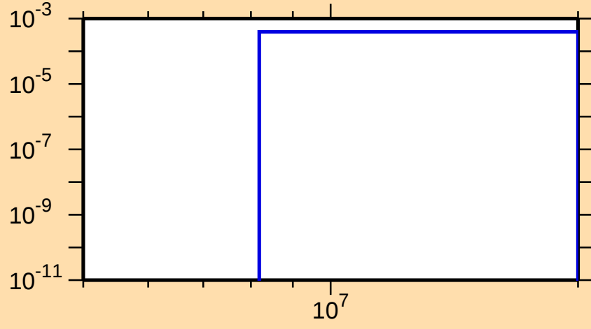
\sigma vs. E for ^{61}\text{Zn}(n,t)
