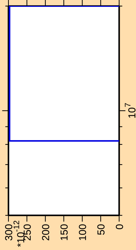
\Delta\sigma/\sigma vs. E for ^{61}\text{Zn}(n,nt)
