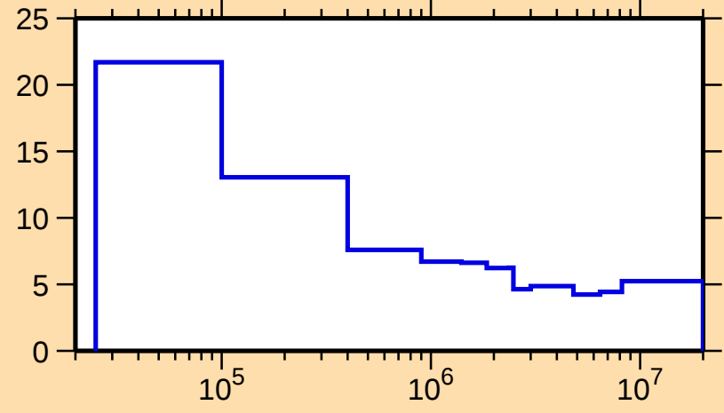
\Delta\sigma/\sigma vs. E for ^{61}\text{Zn}(n,\text{nonel.})
