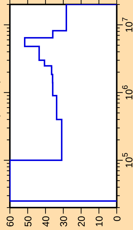
\Delta\sigma/\sigma vs. E for ^{61}\text{Zn}(n,\text{inel.})
