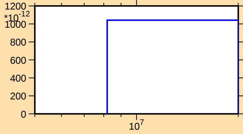
\sigma vs. E for ^{61}\text{Zn}(n,2n\alpha)
