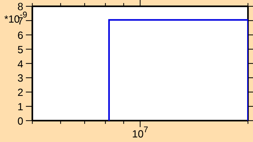
\sigma vs. E for ^{61}\text{Zn}(\text{mt117})
