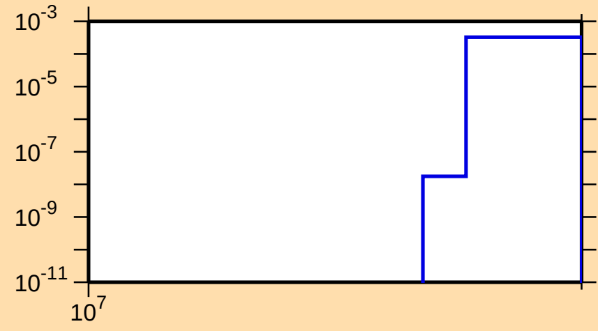
\sigma vs. E for ^{65}\text{Zn}(n,2np)
