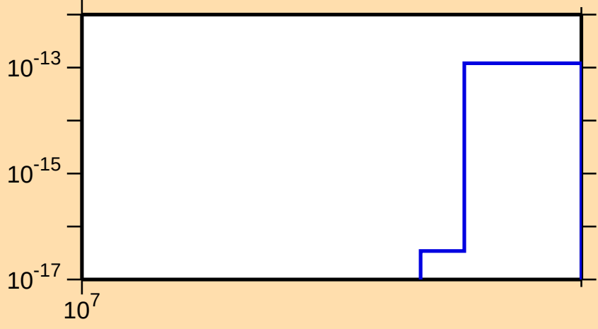
\sigma vs. E for ^{65}\text{Zn}(\text{mt 45})
