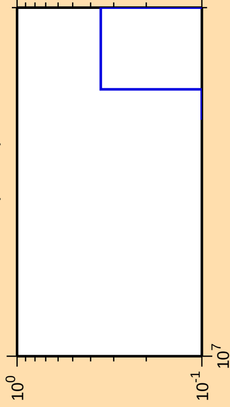
\Delta\sigma/\sigma vs. E for ^{65}\text{Zn}(\text{mt 45})
