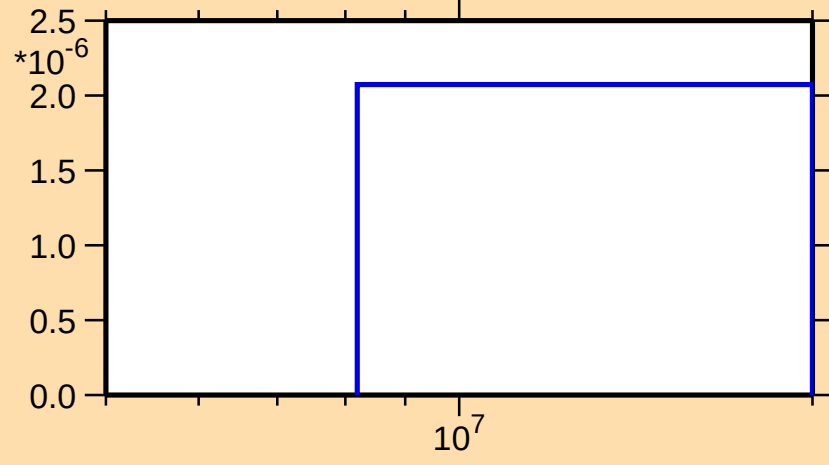
\sigma vs. E for ^{65}\text{Zn}(n,\text{nd})
