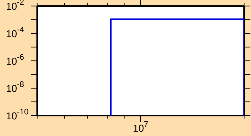
\sigma vs. E for ^{65}\text{Zn}(n,t)
