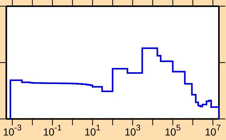
\sigma vs. E for ^{65}\text{Zn}(n,\text{el.})
