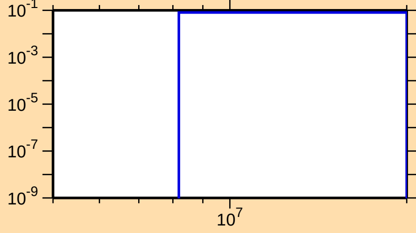
\sigma vs. E for ^{65}\text{Zn}(n,np)
