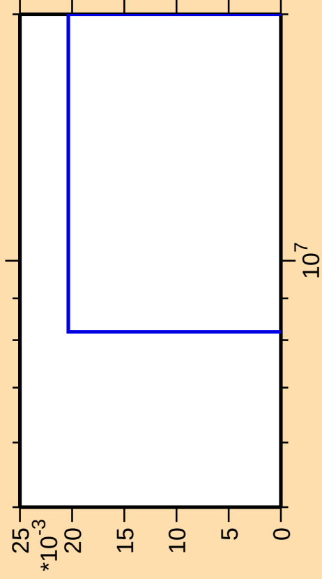
\Delta\sigma/\sigma vs. E for ^{65}\text{Zn}(n,nt)
