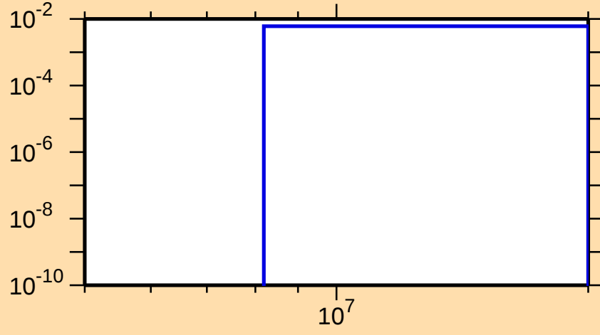
\sigma vs. E for ^{68}\text{Zn}(n,n\alpha)
