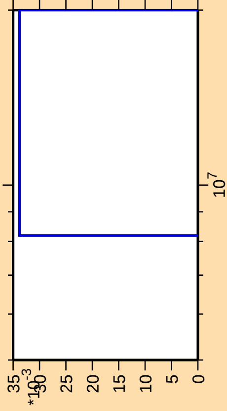
\Delta\sigma/\sigma vs. E for ^{68}\text{Zn}(n,p\alpha)
