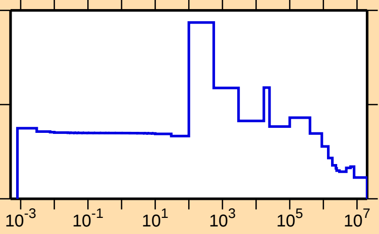
\sigma vs. E for ^{68}\text{Zn}(n,\text{el.})
