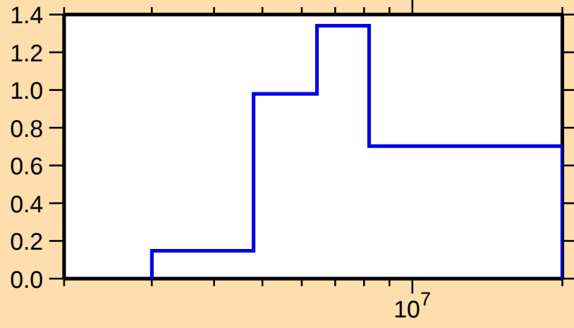
\sigma vs. E for ^{68}\text{Zn}(n,n\text{cont.})
