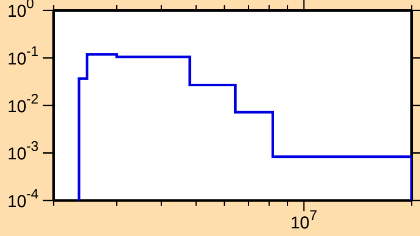
\sigma vs. E for ^{68}\text{Zn}(n,n_4)
