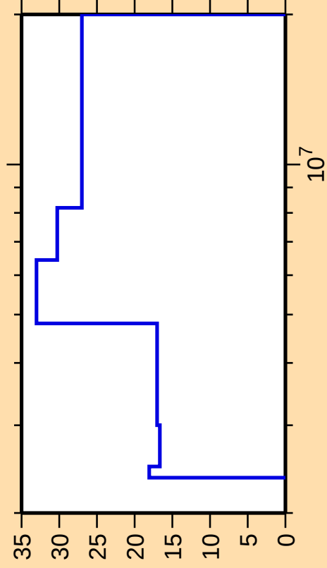
\Delta\sigma/\sigma vs. E for ^{68}\text{Zn}(n,n_4)
