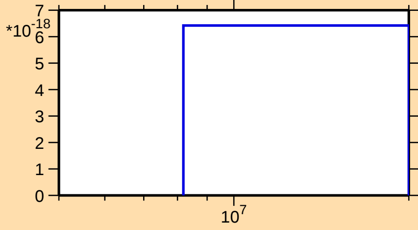
\sigma vs. E for ^{68}\text{Zn}(n,2np)
