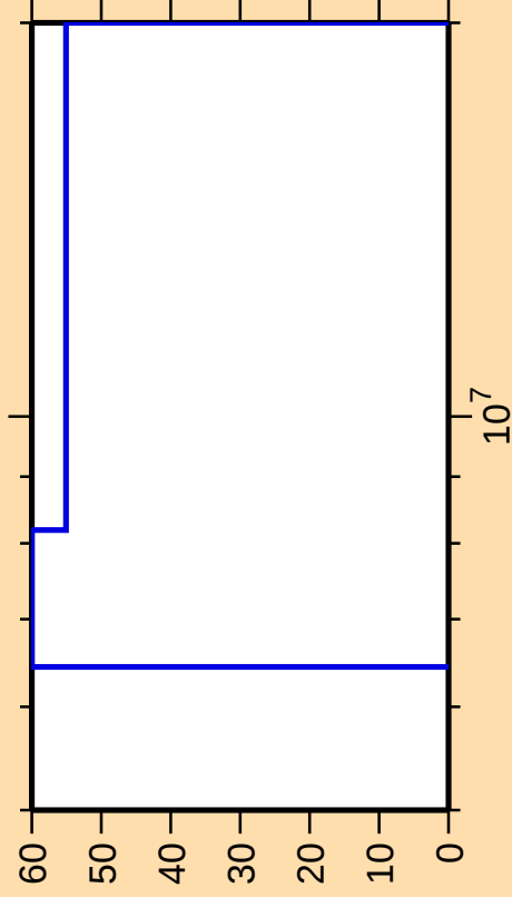
\Delta\sigma/\sigma vs. E for ^{81}\text{Zr}(n,n\alpha)
