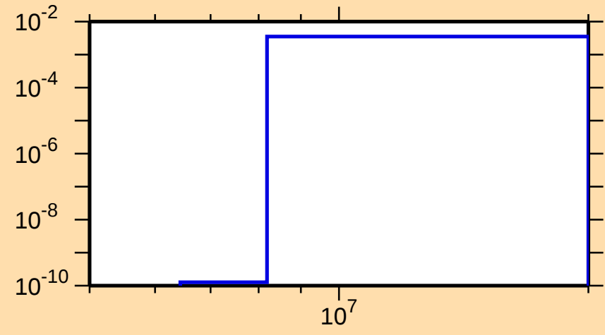
\sigma vs. E for ^{81}\text{Zr}(n,\text{pd})
