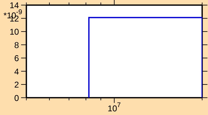
\sigma vs. E for ^{81}\text{Zr}(n,\text{nd})
