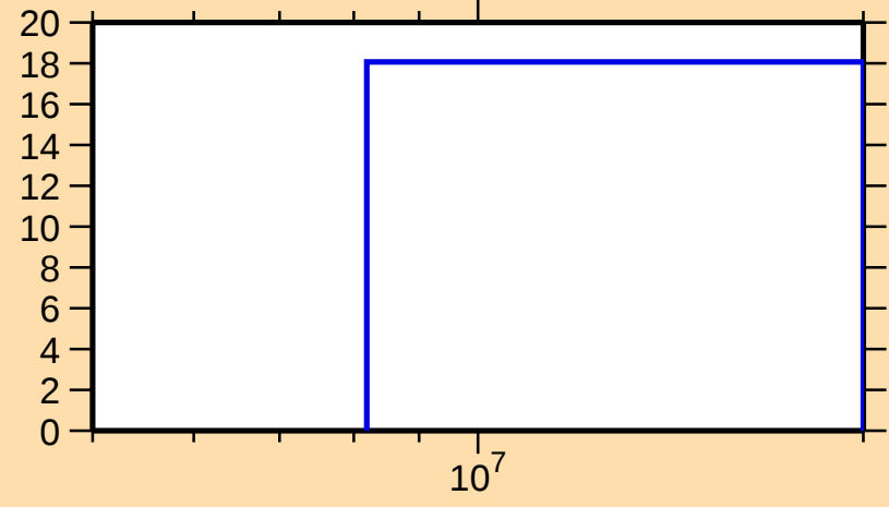
\Delta\sigma/\sigma vs. E for ^{81}\text{Zr}(n,\text{nonel.})
