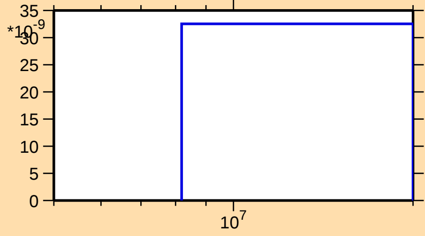
\sigma vs. E for ^{81}\text{Zr}(\text{mt } 45)
