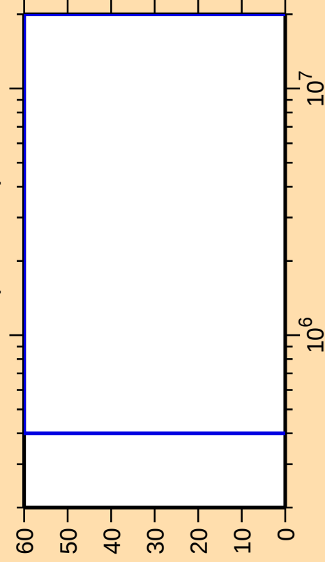
\Delta\sigma/\sigma vs. E for ^{81}\text{Zr}(\text{n},\text{ncont.})
