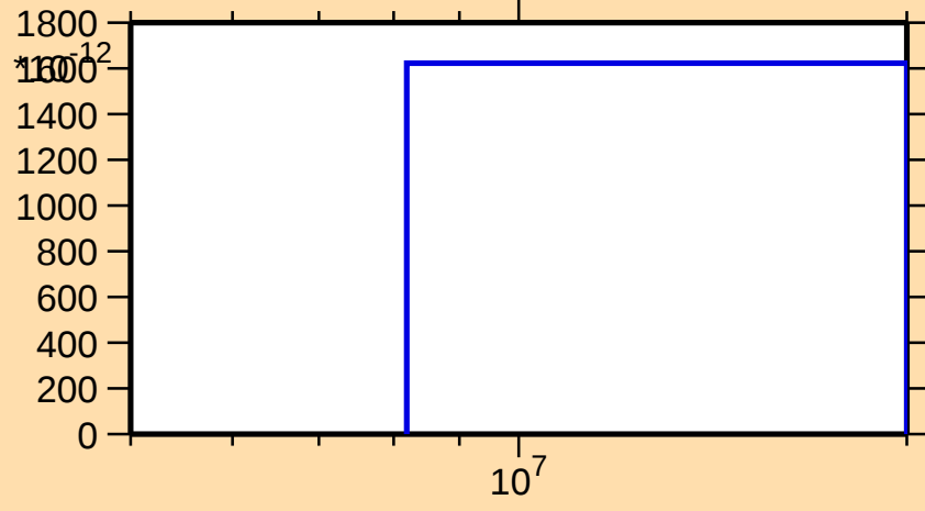
\sigma vs. E for ^{81}\text{Zr}(\text{mt117})
