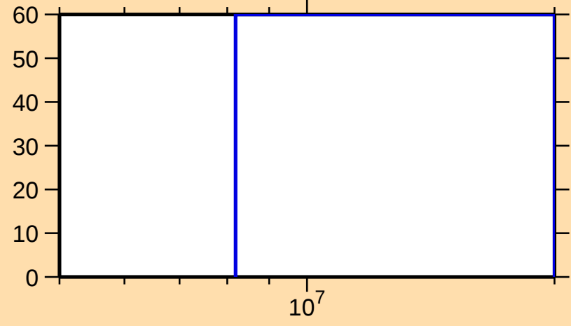
\Delta\sigma/\sigma vs. E for ^{81}\text{Zr}(n,\text{inel.})
