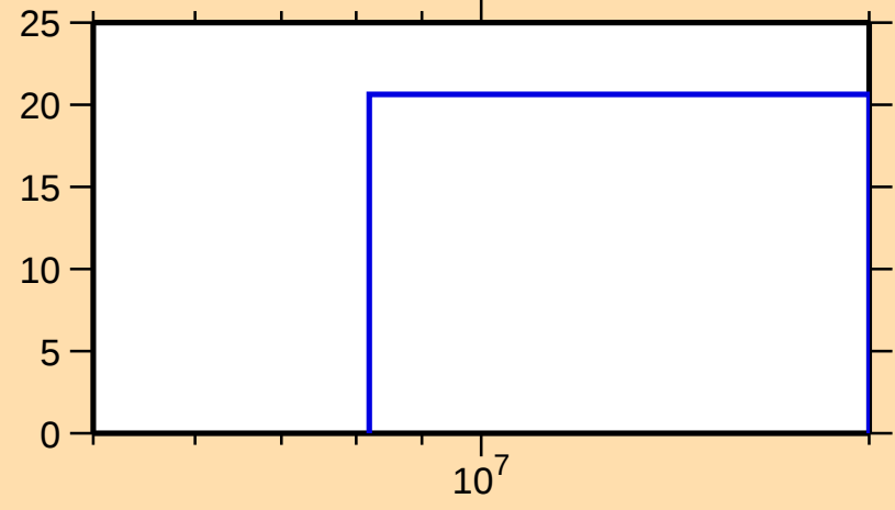
\Delta\sigma/\sigma vs. E for ^{81}\text{Zr}(n,\text{el.})
