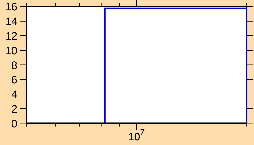
\Delta\sigma/\sigma vs. E for ^{81}\text{Zr}(n,\text{tot.})
