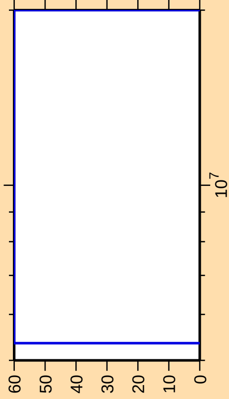
\Delta\sigma/\sigma vs. E for ^{233}\text{Ac}(n,f)
