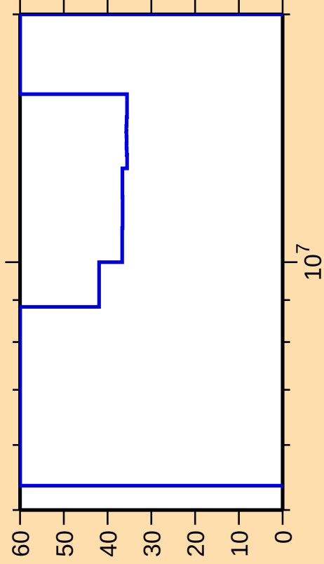
\Delta\sigma/\sigma vs. E for ^{233}\text{Ac}(n,\gamma)
