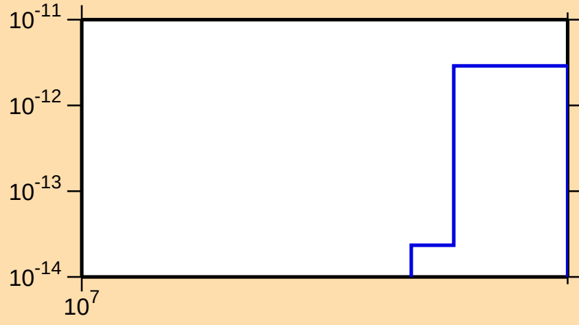
\sigma vs. E for ^{233}\text{Ac}(n,3n\alpha)
