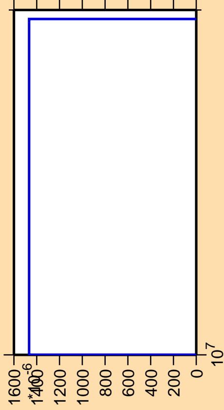
\Delta\sigma/\sigma vs. E for ^{233}\text{Ac}(\text{mt } 42)
