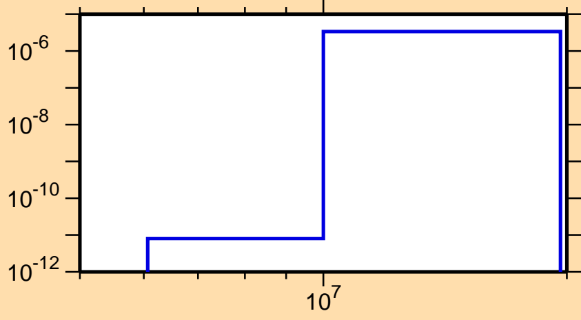
\sigma vs. E for ^{233}\text{Ac}(n,n\alpha)
