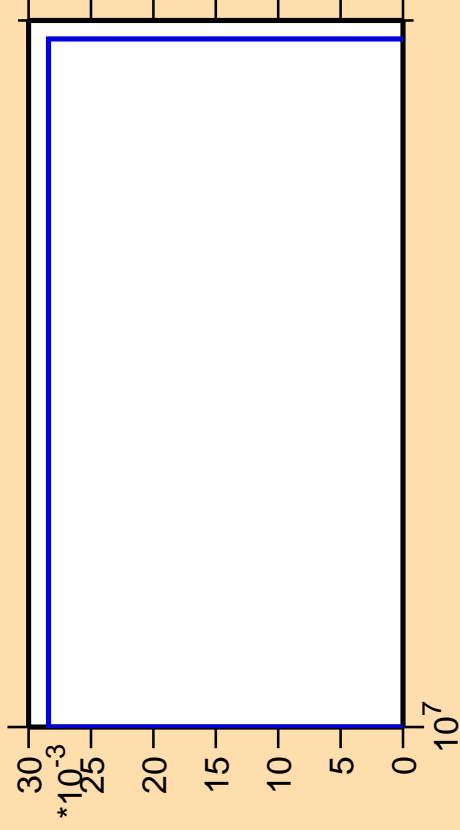
\Delta\sigma/\sigma vs. E for ^{233}\text{Ac} (mt 11)
