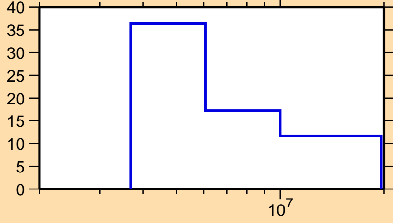
\Delta\sigma/\sigma vs. E for ^{233}\text{Ac}(n,ncont.)
