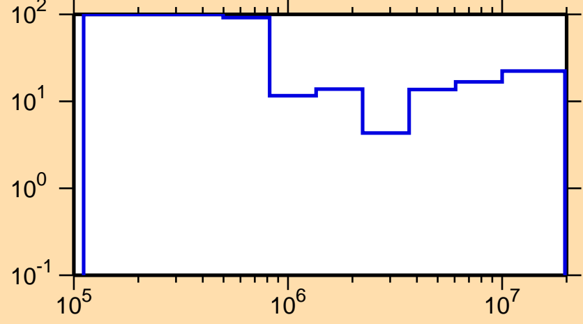
\Delta\sigma/\sigma vs. E for ^{233}\text{Ac}(n,\text{nonel.})
