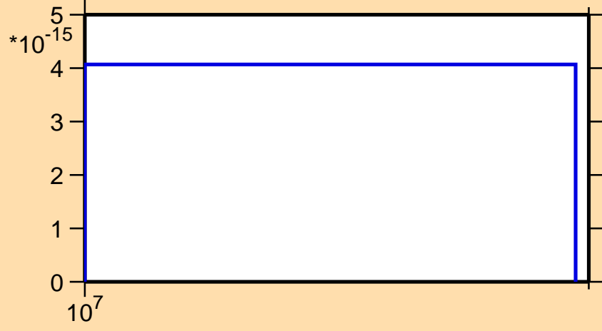
\sigma vs. E for ^{233}\text{Ac} (mt 11)
