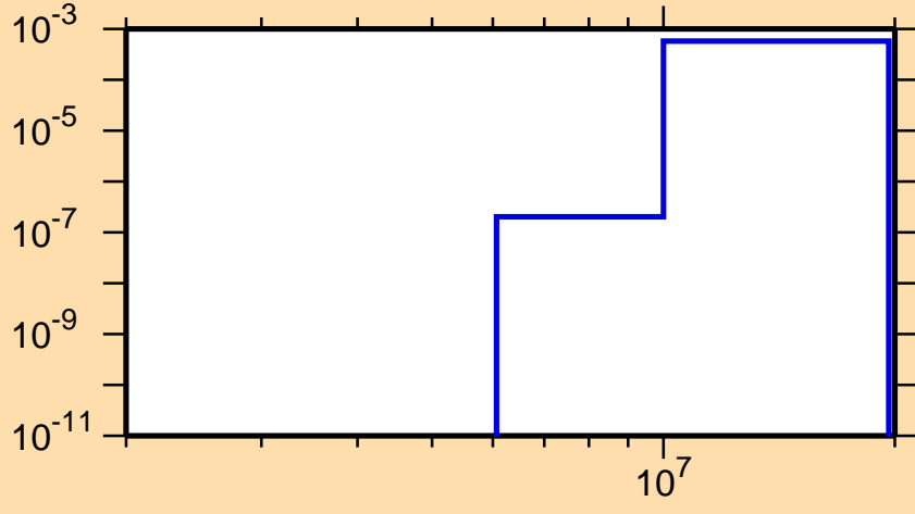
\sigma vs. E for ^{233}\text{Ac}(n,p)
