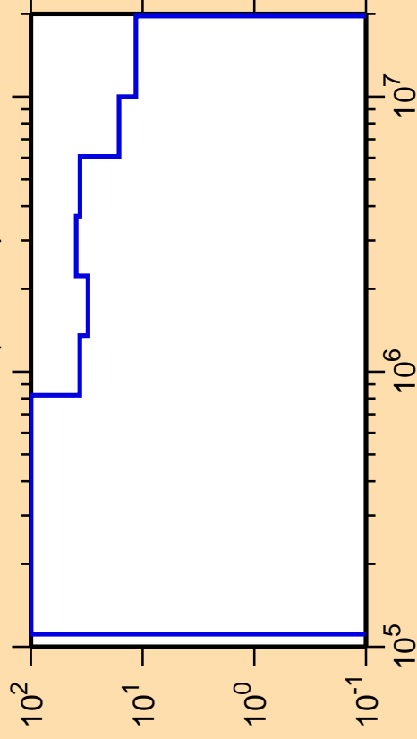
\Delta\sigma/\sigma vs. E for ^{233}\text{Ac}(n,\text{inel.})
