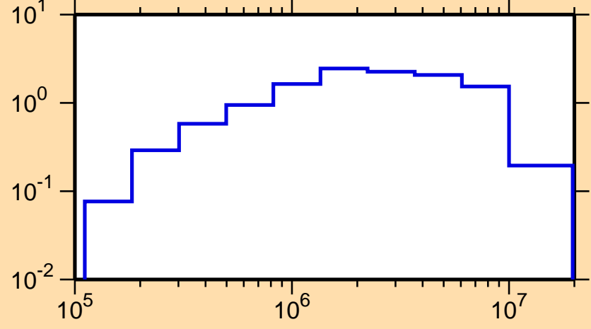
\sigma vs. E for ^{233}\text{Ac}(n,\text{inel.})
