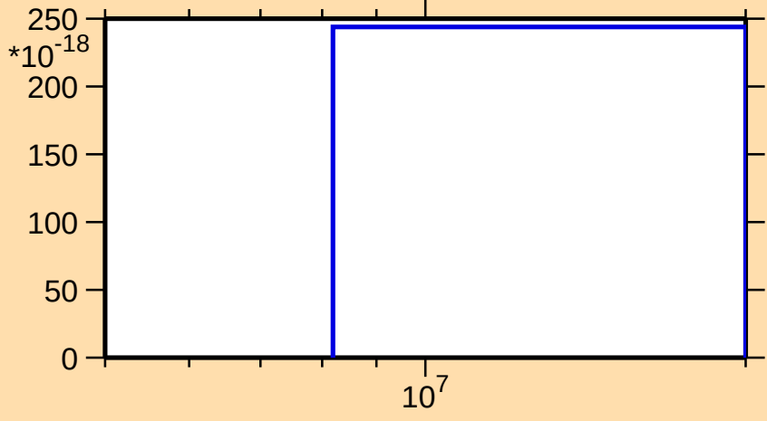
\sigma vs. E for ^{233}\text{Ac}(\text{mt } 42)
