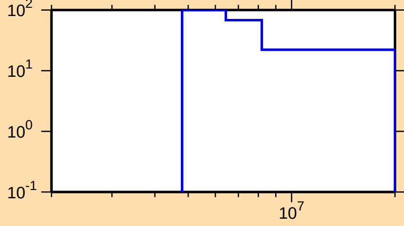
\Delta\sigma/\sigma vs. E for ^{233}\text{Ac}(n,2n)
