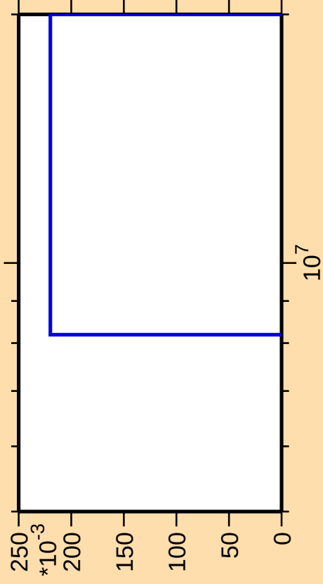
\Delta\sigma/\sigma vs. E for ^{233}\text{Ac}(n,3n\alpha)
