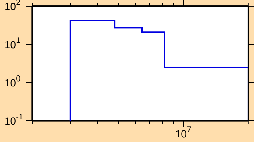
\Delta\sigma/\sigma vs. E for ^{233}\text{Ac}(n,n\text{cont.})
