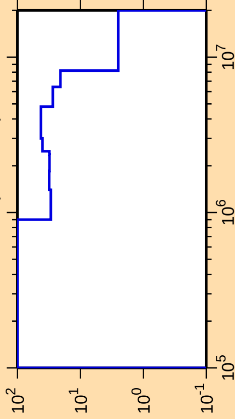
\Delta\sigma/\sigma vs. E for ^{233}\text{Ac}(n,\text{ncont.})
