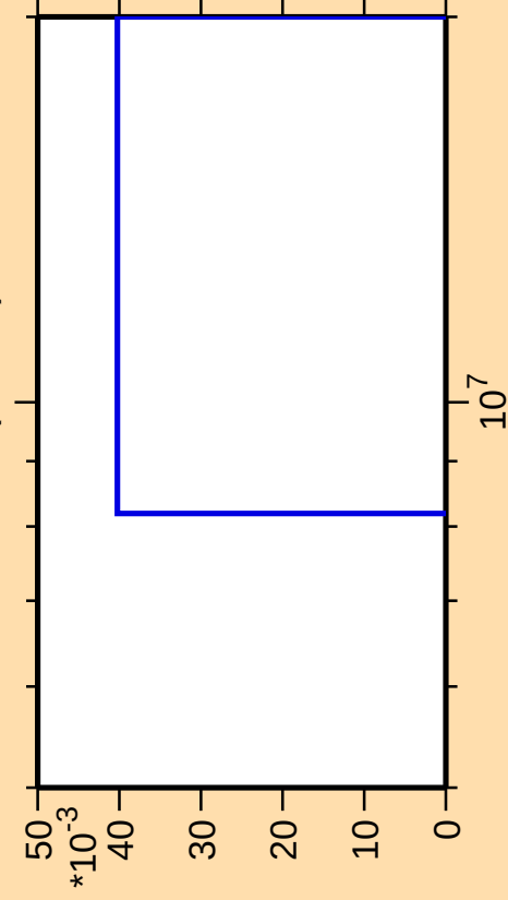
\Delta\sigma/\sigma vs. E for ^{233}\text{Ac}(\text{mt 11})
