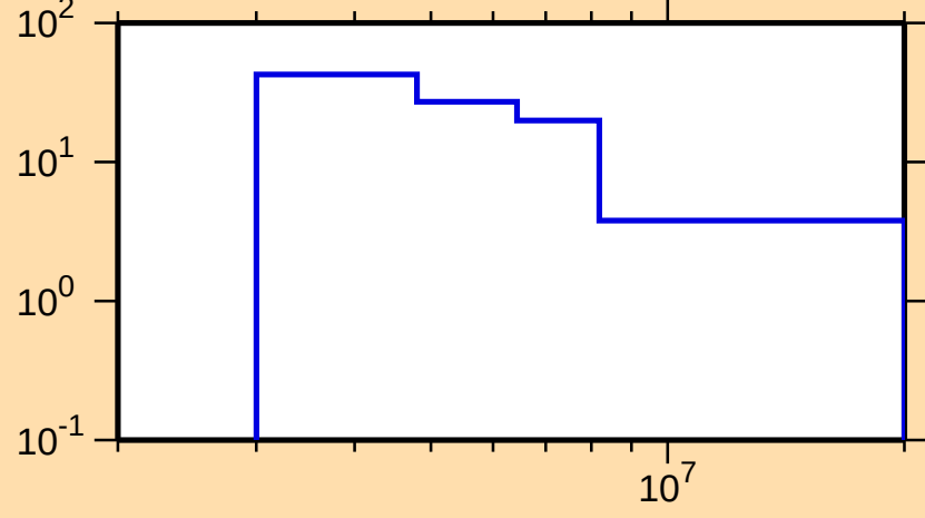
\Delta\sigma/\sigma vs. E for ^{233}\text{Ac}(n,\text{inel.})
