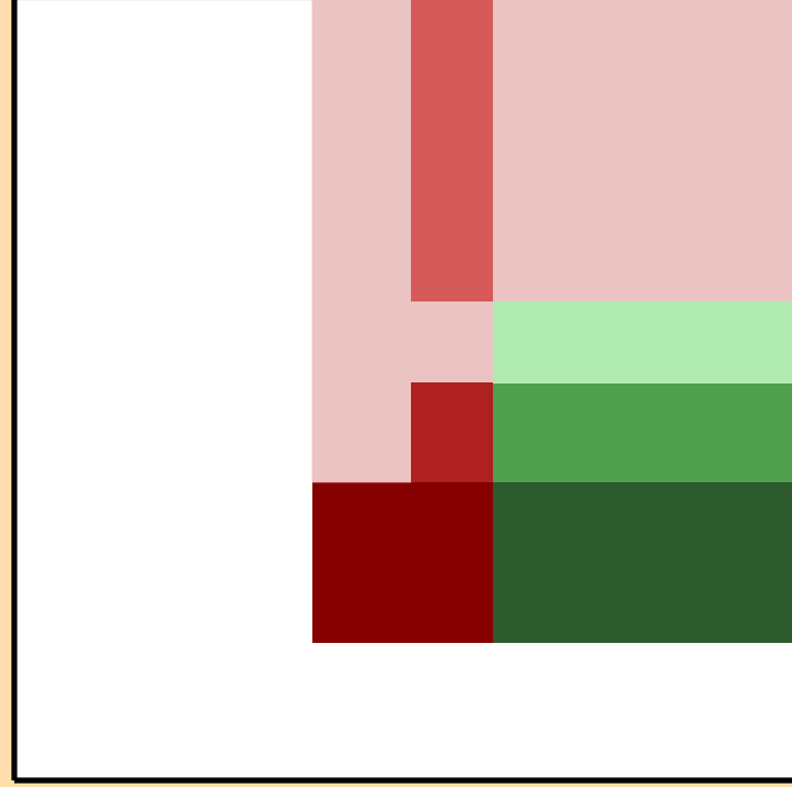
\Delta\sigma/\sigma vs. E for ^{233}\text{Ac}(n,2n)
