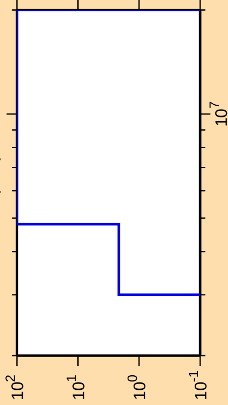
\Delta\sigma/\sigma vs. E for ^{233}\text{Ac}(n,\alpha)
