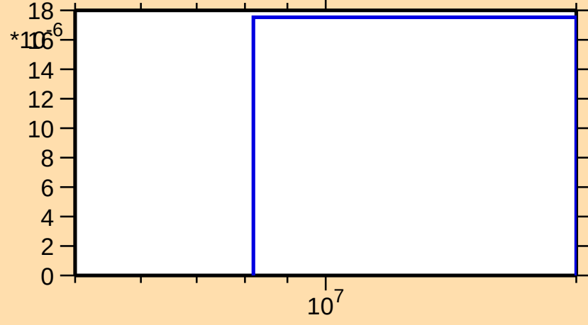
\sigma vs. E for ^{233}\text{Ac}(n,t)
