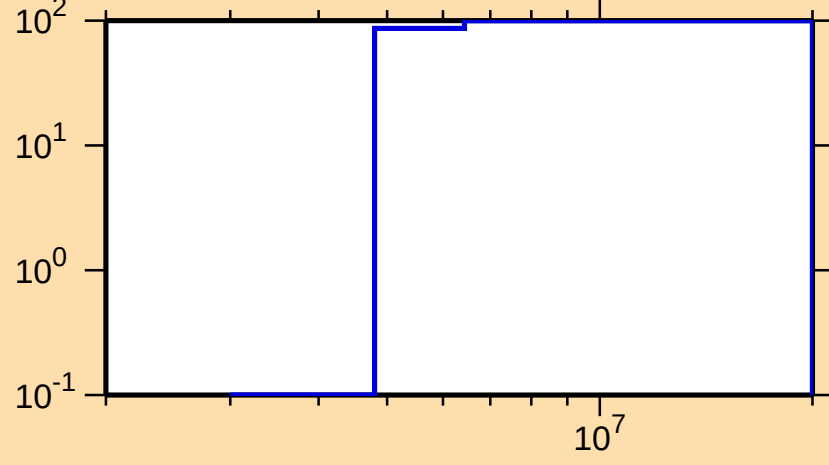
\Delta\sigma/\sigma vs. E for ^{233}\text{Ac}(n,p)
