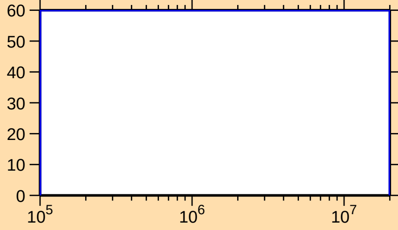
\Delta\sigma/\sigma vs. E for ^{233}\text{Ac}(n,\text{f})
