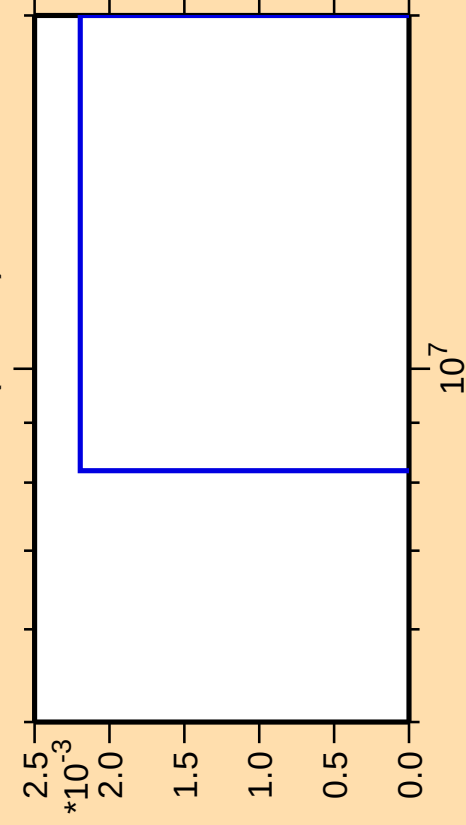
\Delta\sigma/\sigma vs. E for ^{233}\text{Ac}(\text{mt } 42)
