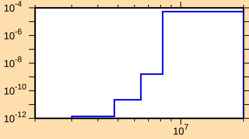
\sigma vs. E for ^{233}\text{Ac}(n,\alpha)
