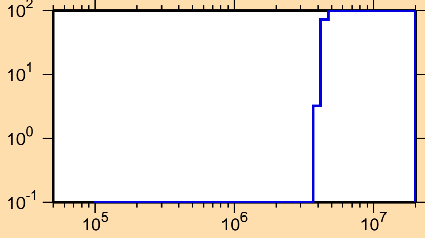
\Delta\sigma/\sigma vs. E for ^{237}\text{Ac}(n,\text{f})
