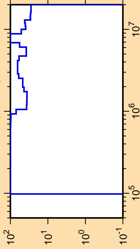
\Delta\sigma/\sigma vs. E for ^{237}\text{Ac}(n,\text{inel.})
