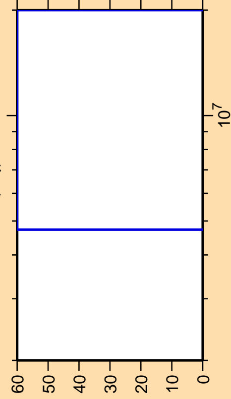
\Delta\sigma/\sigma vs. E for ^{237}\text{Ac}(n,\gamma)
