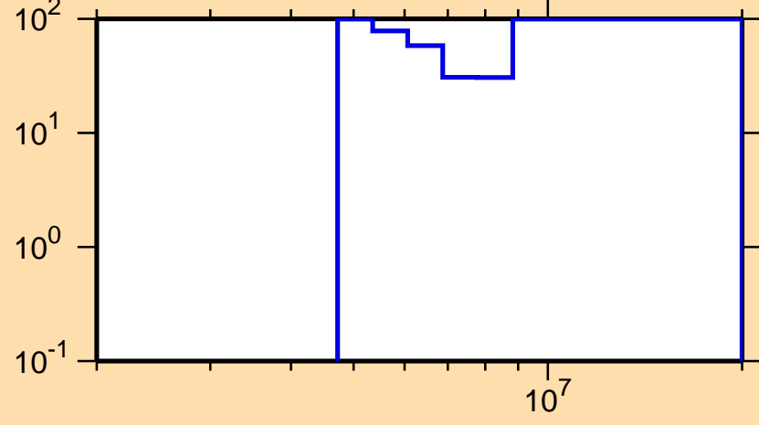
\Delta\sigma/\sigma vs. E for ^{237}\text{Ac}(n,2n)
