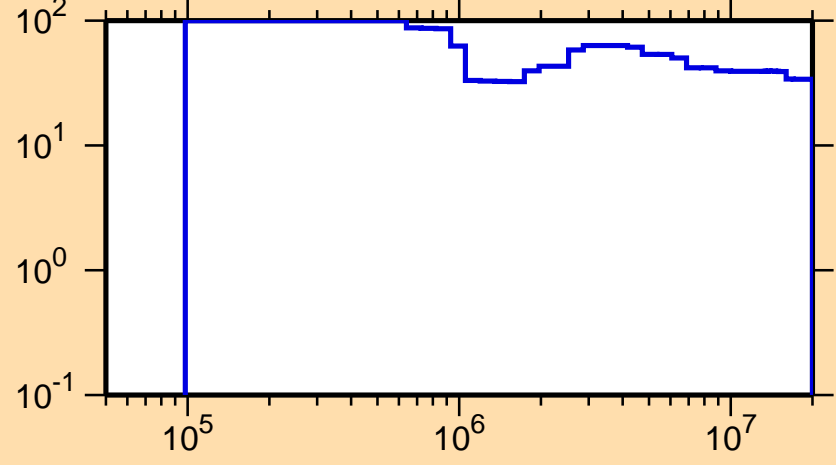
\Delta\sigma/\sigma vs. E for ^{237}\text{Ac}(n,\text{nonel.})
