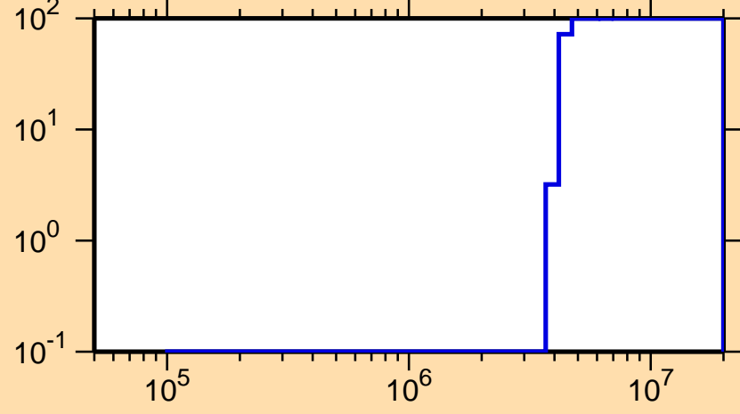
\Delta\sigma/\sigma vs. E for ^{237}\text{Ac}(n,f)
