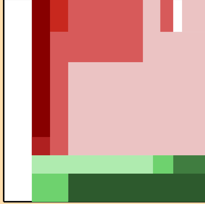
\Delta\sigma/\sigma vs. E for ^{237}\text{Ac}(n,p)
