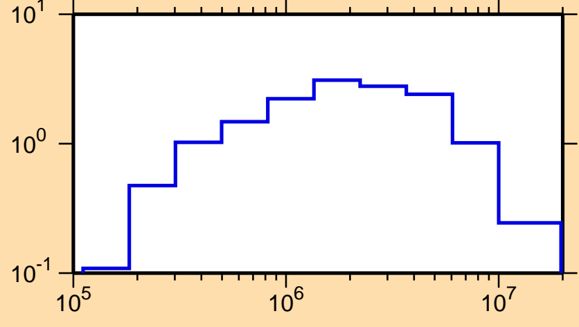
\sigma vs. E for ^{237}\text{Ac}(n,\text{inel.})
