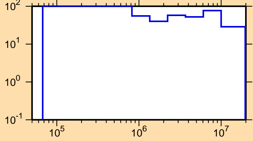
\Delta\sigma/\sigma vs. E for ^{237}\text{Ac}(n,\text{inel.})
