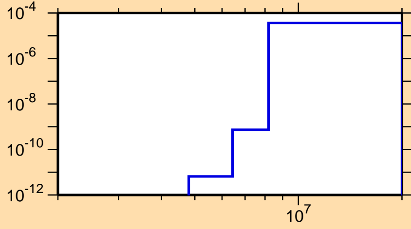
\sigma vs. E for ^{237}\text{Ac}(n,\alpha)
