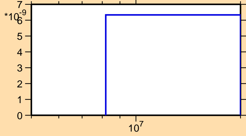
\sigma vs. E for ^{237}\text{Ac}(n,\text{nd})
