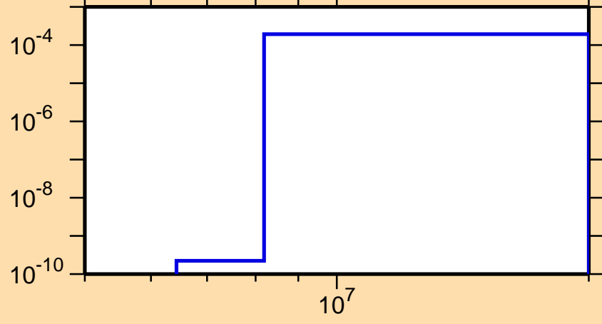
\sigma vs. E for ^{237}\text{Ac}(n,p)
