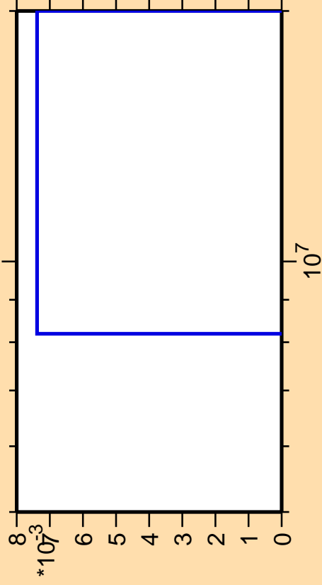
\Delta\sigma/\sigma vs. E for ^{237}\text{Ac}(\text{mt } 42)
