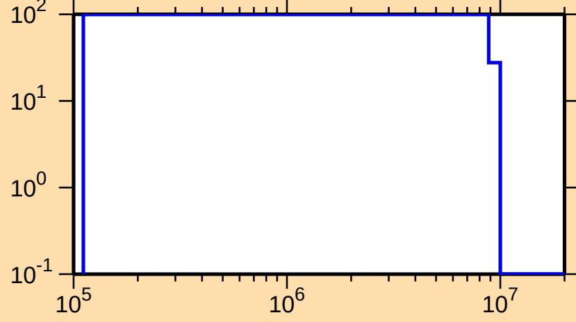
\Delta\sigma/\sigma vs. E for ^{230}\text{Am}(n,n_1)
