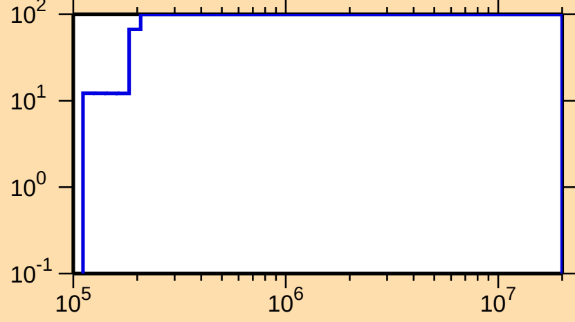
\Delta\sigma/\sigma vs. E for ^{230}\text{Am}(n,\text{tot.})
