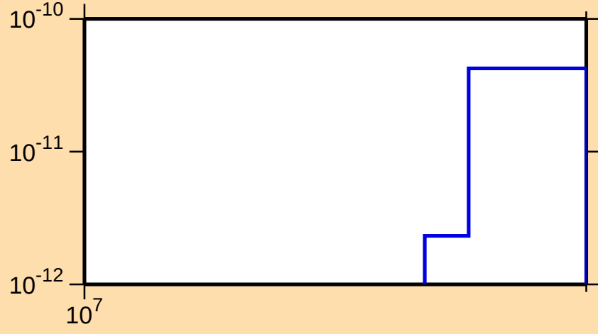
\sigma vs. E for ^{230}\text{Am}(\text{mt } 34)
