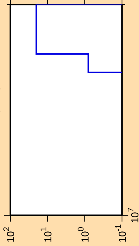
\Delta\sigma/\sigma vs. E for ^{230}\text{Am}(n,\text{nt})
