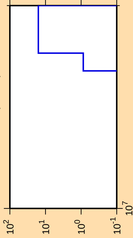
\Delta\sigma/\sigma vs. E for ^{230}\text{Am}(\text{mt } 34)
