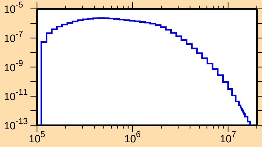
\sigma vs. E for ^{230}\text{Am}(n,n_1)
