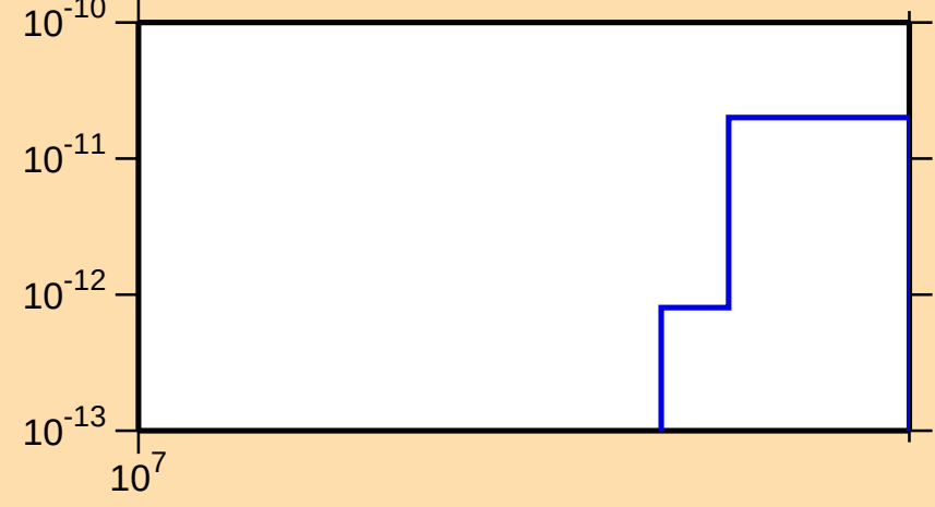
\sigma vs. E for ^{230}\text{Am}(n,\text{nt})
