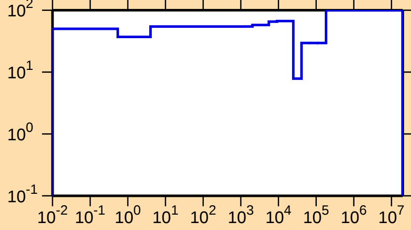
\Delta\sigma/\sigma vs. E for ^{230}\text{Am}(n,\text{el.})
