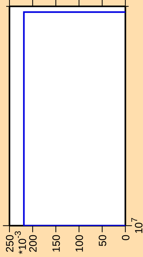
\Delta\sigma/\sigma vs. E for ^{230}\text{Am}(n,\text{nt})
