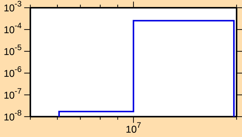
\sigma vs. E for ^{230}\text{Am}(n,np)
