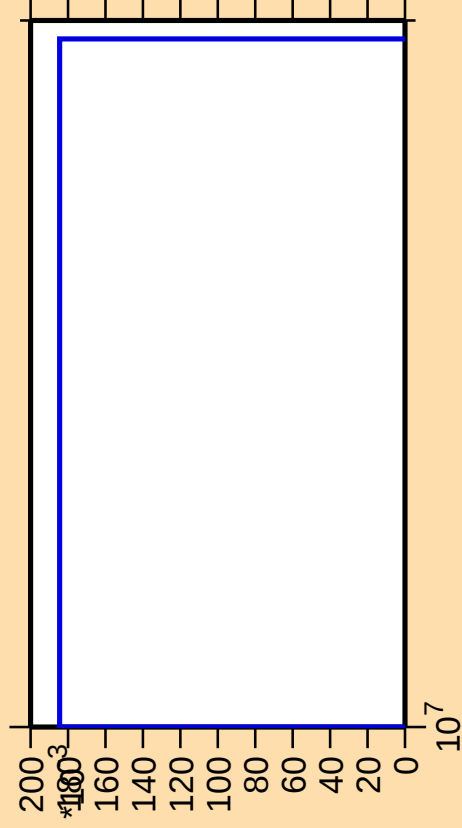
\Delta\sigma/\sigma vs. E for ^{230}\text{Am}(\text{mt } 34)
