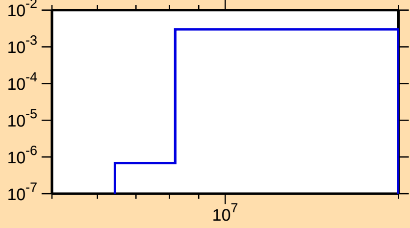
\sigma vs. E for ^{230}\text{Am}(n,2n)
