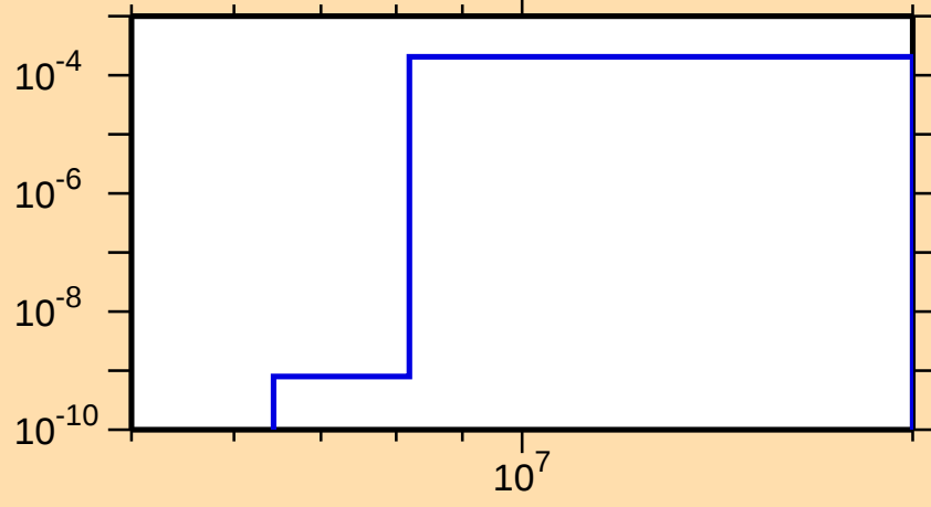
\sigma vs. E for ^{230}\text{Am}(n,np)
