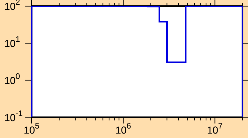
\Delta\sigma/\sigma vs. E for ^{230}\text{Am}(n,\text{inel.})
