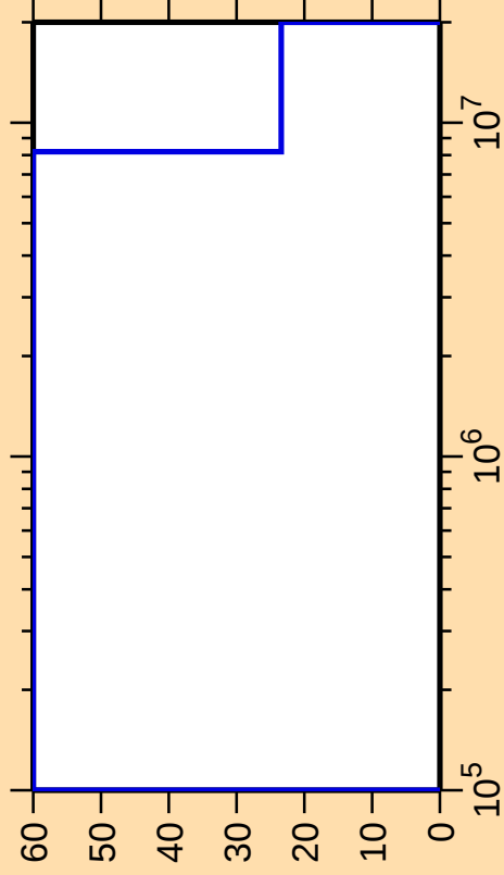
\Delta\sigma/\sigma vs. E for ^{230}\text{Am}(n,n_1)
