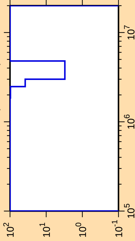
\Delta\sigma/\sigma vs. E for ^{230}\text{Am}(n,\text{ncont.})
