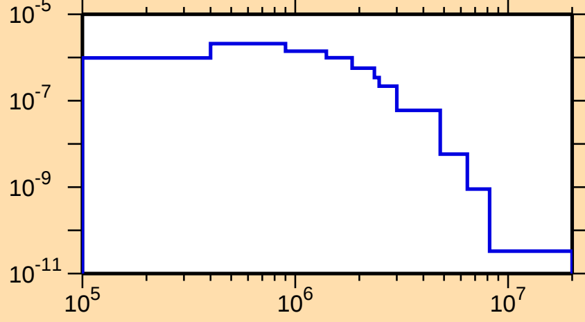
\sigma vs. E for ^{230}\text{Am}(n,n_1)
