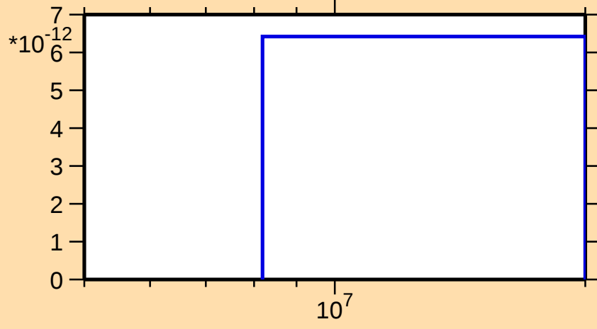
\sigma vs. E for ^{230}\text{Am}(\text{mt } 45)
