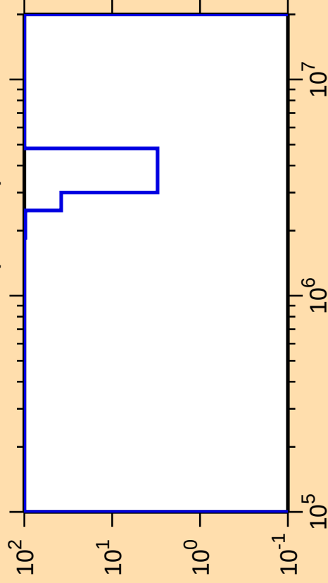
\Delta\sigma/\sigma vs. E for ^{230}\text{Am}(n,\text{inel.})
