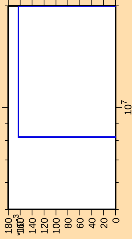
\Delta\sigma/\sigma vs. E for ^{230}\text{Am} (mt 34)
