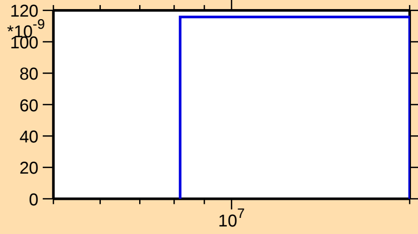
\sigma vs. E for ^{230}\text{Am}(n,\text{He3})
