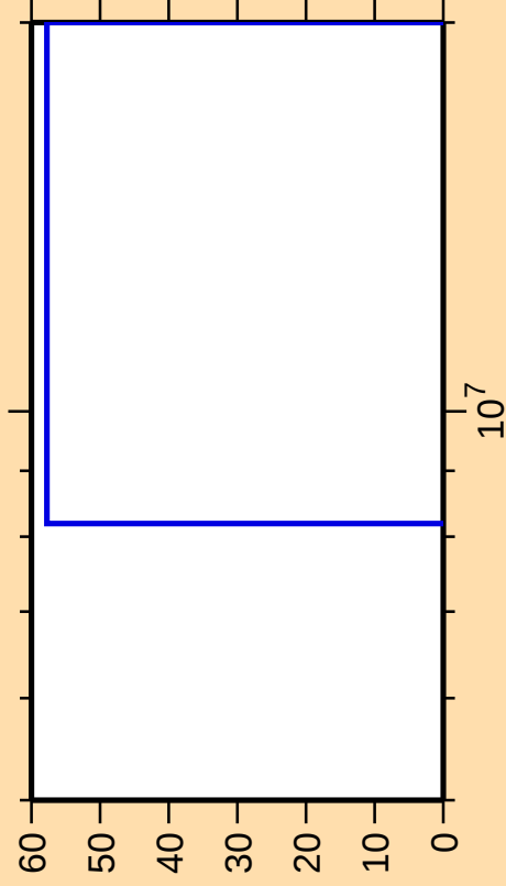
\Delta\sigma/\sigma vs. E for ^{230}\text{Am}(\text{mt } 45)
