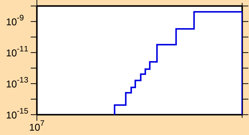
\sigma vs. E for ^{235}\text{Am}(n,\text{nd})
