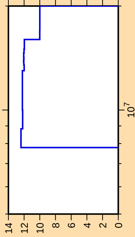
\Delta\sigma/\sigma vs. E for ^{235}\text{Am}(n,f)
