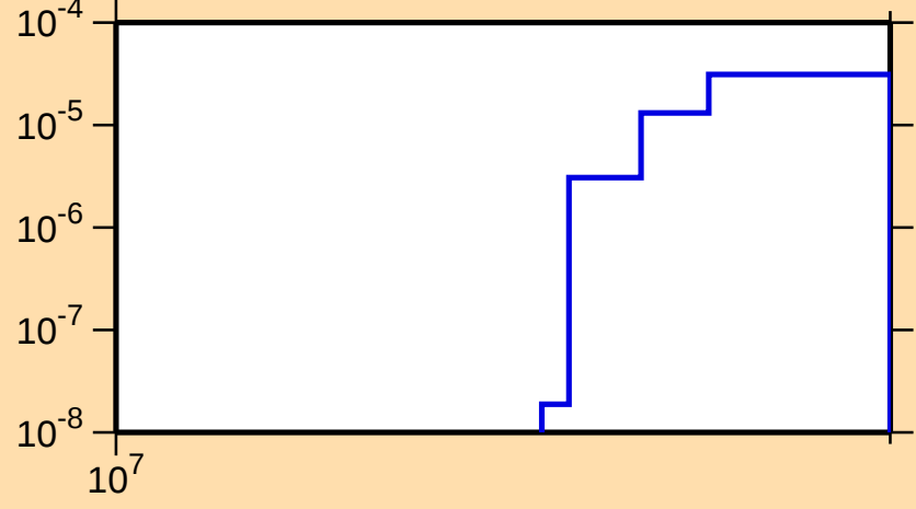
\sigma vs. E for ^{235}\text{Am}(n,3n)
