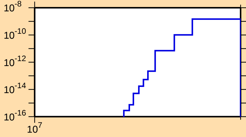
\sigma vs. E for ^{235}\text{Am}(n,2np)
