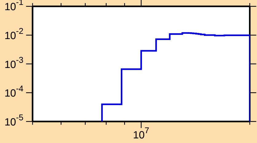
\sigma vs. E for ^{235}\text{Am}(n,2n)
