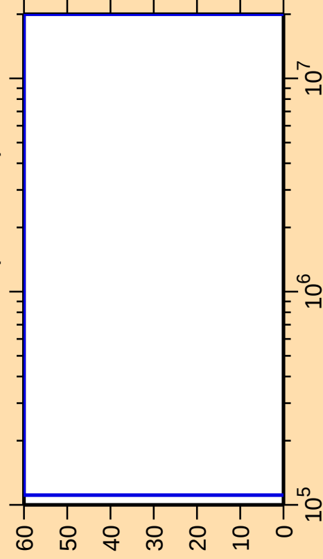
\Delta\sigma/\sigma vs. E for ^{235}\text{Am}(n,\text{ncont.})
