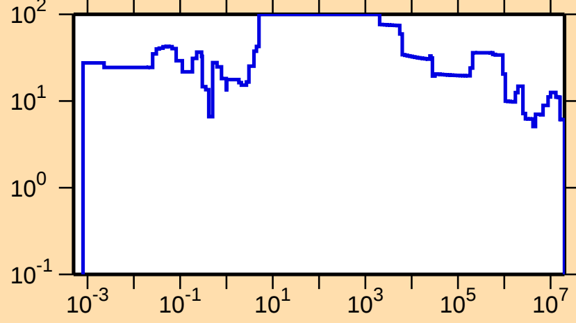
\Delta\sigma/\sigma vs. E for ^{235}\text{Am}(n,\text{tot.})
