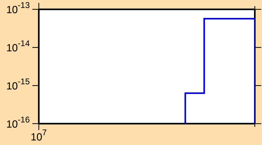
\sigma vs. E for ^{235}\text{Am}(n,3n\alpha)
