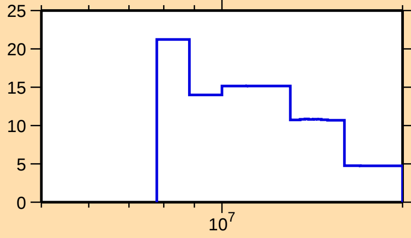
\Delta\sigma/\sigma vs. E for ^{235}\text{Am}(n,\text{el.})
