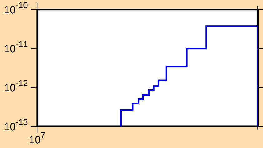
\sigma vs. E for ^{235}\text{Am}(n,p\alpha)
