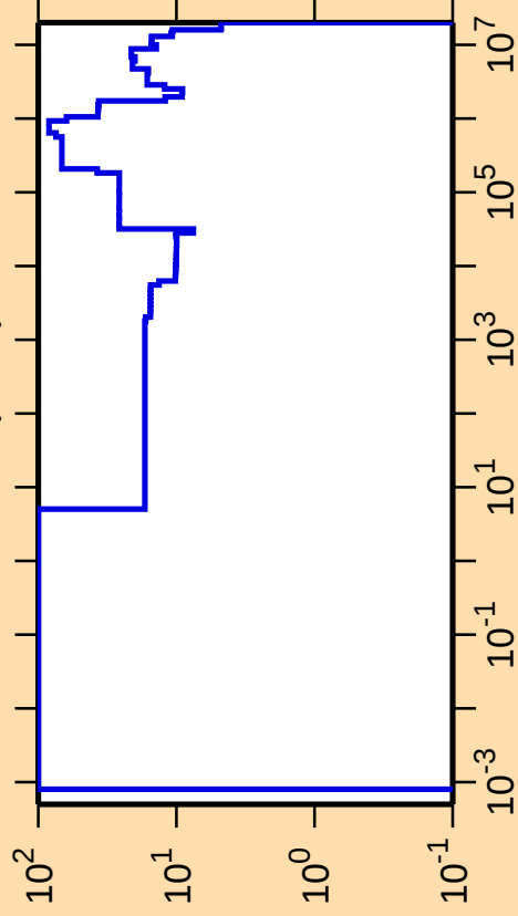
\Delta\sigma/\sigma vs. E for ^{235}\text{Am}(n,\text{el.})
