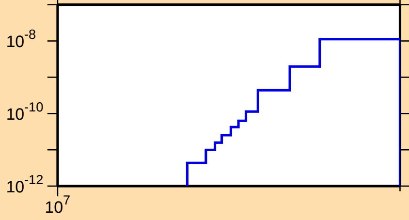
\sigma vs. E for ^{235}\text{Am}(n,\text{He3})
