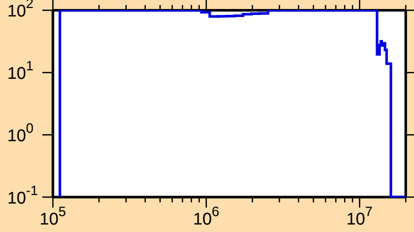
\Delta\sigma/\sigma vs. E for ^{235}\text{Am}(n,n_1)
