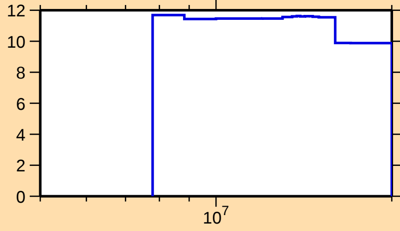
\Delta\sigma/\sigma vs. E for ^{235}\text{Am}(n,\text{nonel.})
