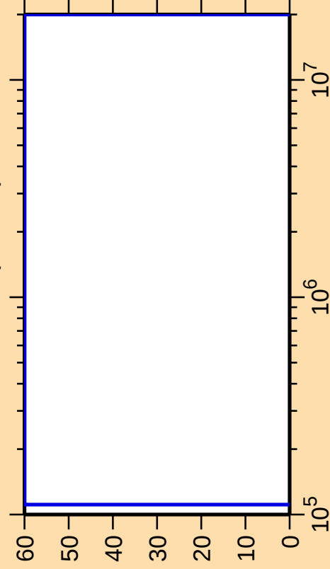
\Delta\sigma/\sigma vs. E for ^{235}\text{Am}(n,\text{inel.})
