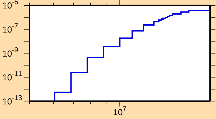
\sigma vs. E for ^{235}\text{Am}(n,np)
