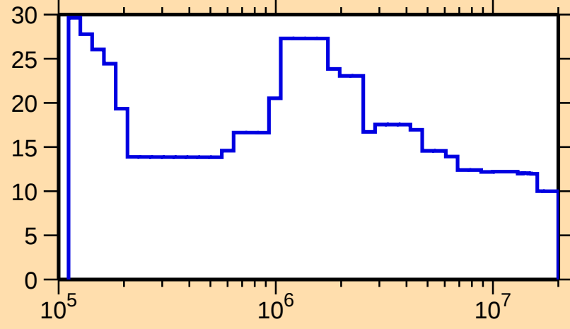
\Delta\sigma/\sigma vs. E for ^{235}\text{Am}(n,f)
