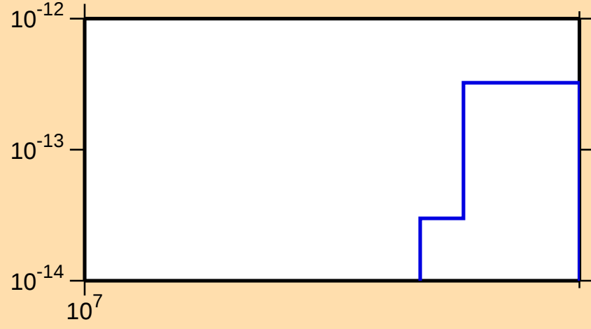
\sigma vs. E for ^{235}\text{Am}(\text{mt } 45)
