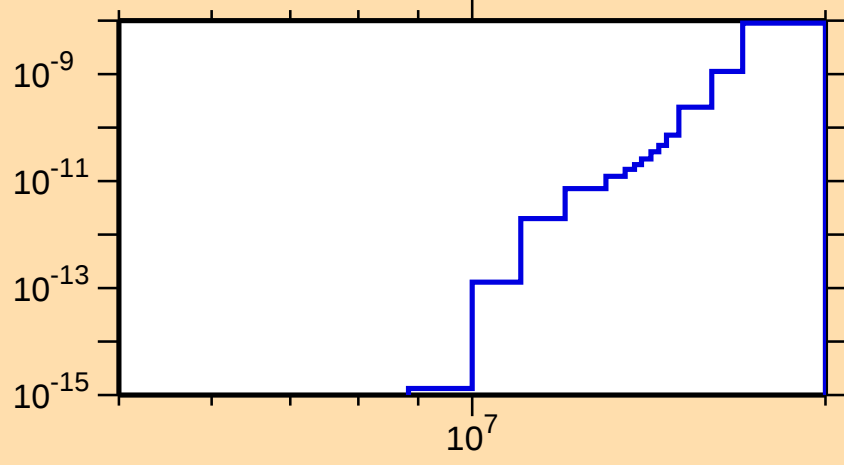
\sigma vs. E for ^{235}\text{Am}(n,2n\alpha)
