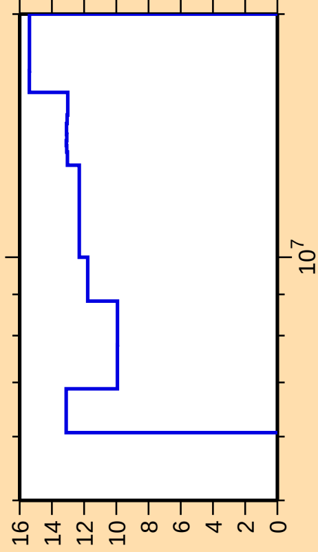
\Delta\sigma/\sigma vs. E for ^{238}\text{Am}(n,f)
