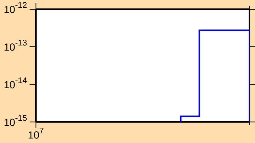
\sigma vs. E for ^{238}\text{Am}(\text{mt } 34)
