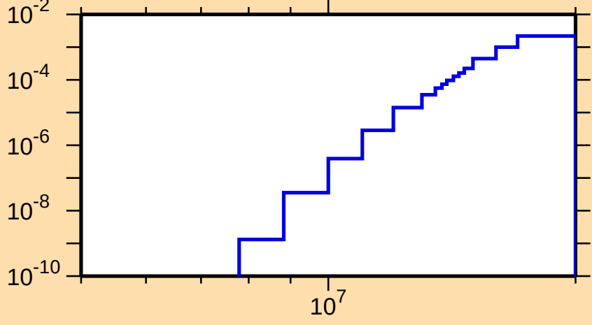
\sigma vs. E for ^{238}\text{Am}(n,np)
