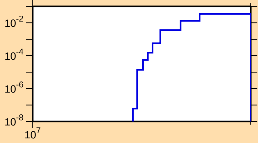
\sigma vs. E for ^{238}\text{Am}(n,3n)
