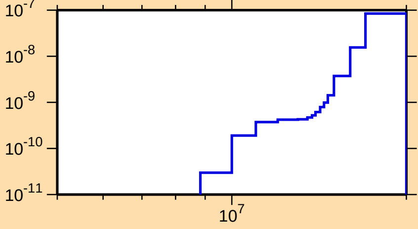
\sigma vs. E for ^{238}\text{Am}(n,2n\alpha)
