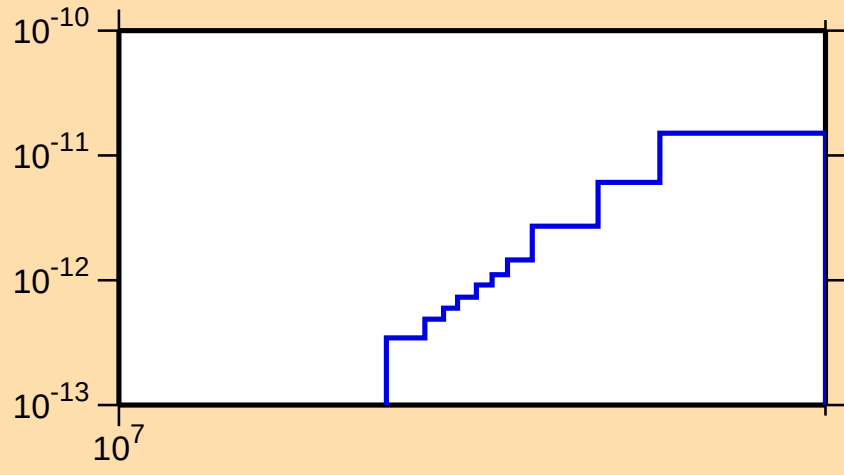
\sigma vs. E for ^{238}\text{Am}(n,p\alpha)
