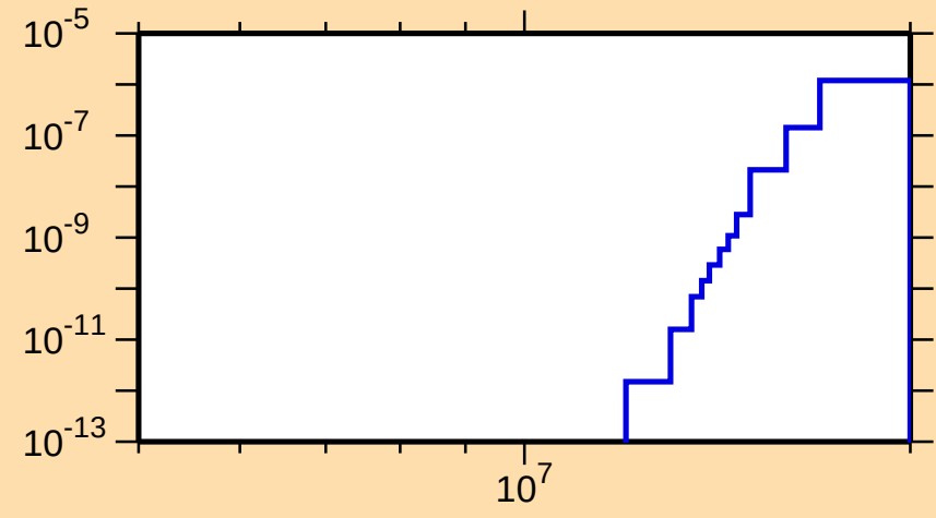
\sigma vs. E for ^{238}\text{Am}(n,\text{nd})
