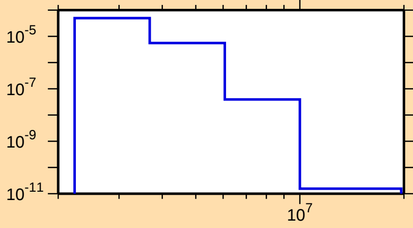
\sigma vs. E for ^{238}\text{Am}(n,n_1)
