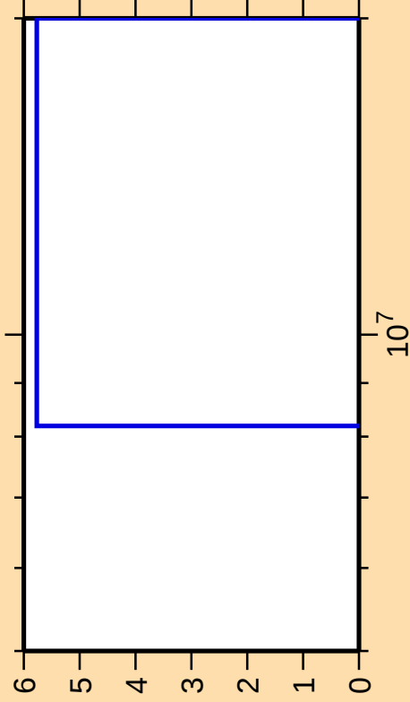
\Delta\sigma/\sigma vs. E for ^{238}\text{Am}(n,p\alpha)
