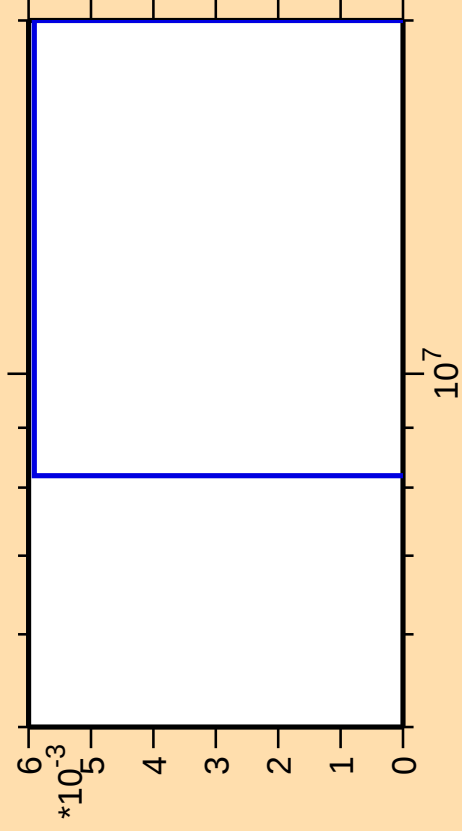
\Delta\sigma/\sigma vs. E for ^{238}\text{Am}(\text{mt } 34)
