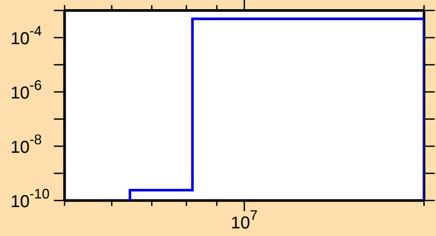
\sigma vs. E for ^{238}\text{Am}(n,d)
