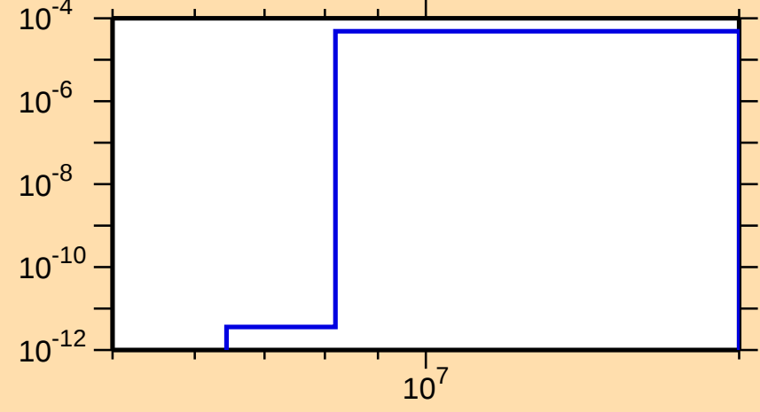
\sigma vs. E for ^{238}\text{Am}(n,t)
