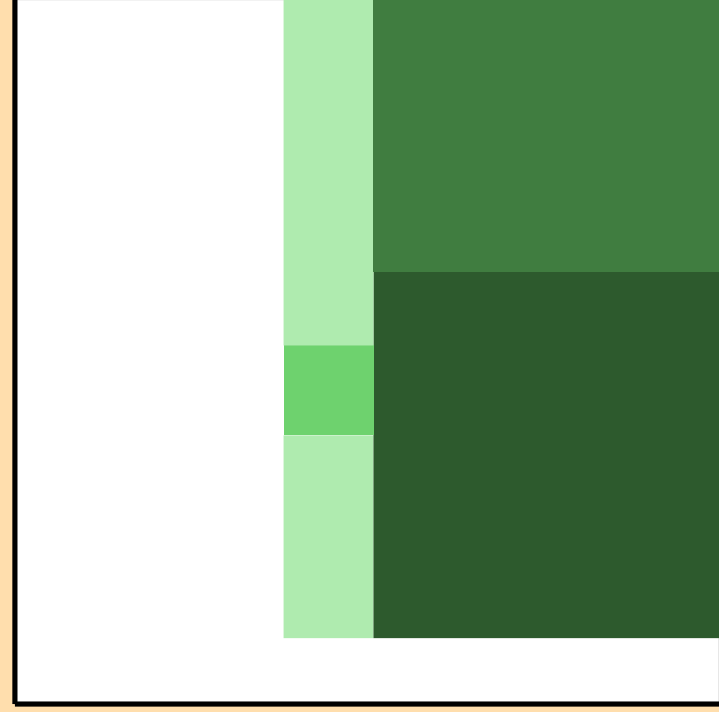
\Delta\sigma/\sigma vs. E for ^{238}\text{Am}(n,2n)
