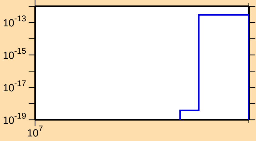
\sigma vs. E for ^{244}\text{Bk}(\text{mt 11})
