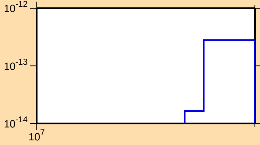
\sigma vs. E for ^{244}\text{Bk}(n,3n\alpha)
