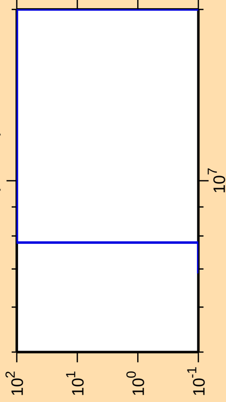
\Delta\sigma/\sigma vs. E for ^{244}\text{Bk}(n,2n\alpha)
