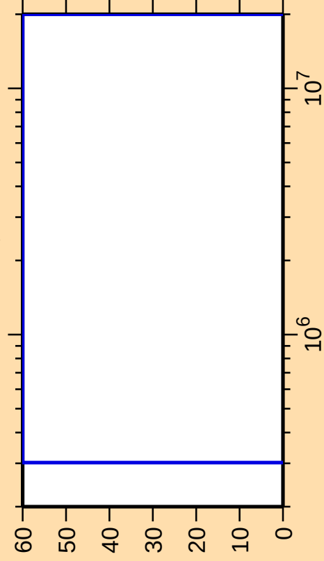
\Delta\sigma/\sigma vs. E for ^{244}\text{Bk}(n,\gamma)
