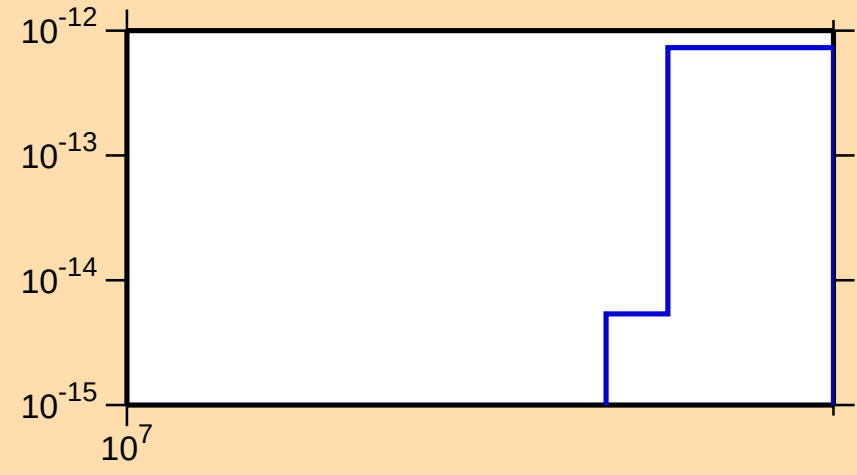
\sigma vs. E for ^{244}\text{Bk}(\text{mt } 34)
