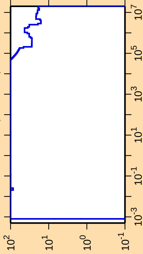
\Delta\sigma/\sigma vs. E for ^{244}\text{Bk}(n,\text{nonel.})
