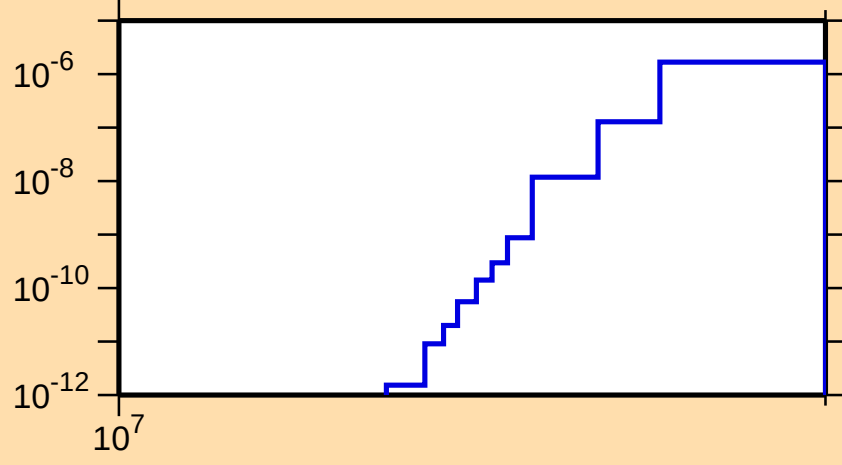
\sigma vs. E for ^{244}\text{Bk}(n,nt)
