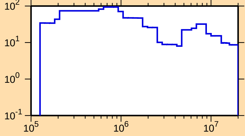
\Delta\sigma/\sigma vs. E for ^{244}\text{Bk}(n,\text{el.})
