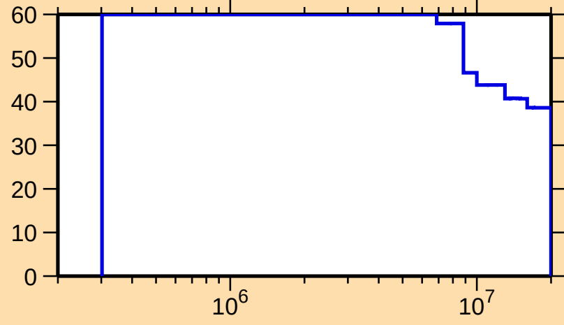
\Delta\sigma/\sigma vs. E for ^{244}\text{Bk}(n,n\text{cont.})
