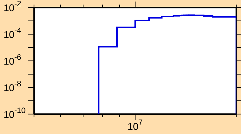
\sigma vs. E for ^{244}\text{Bk}(n,2n\alpha)
