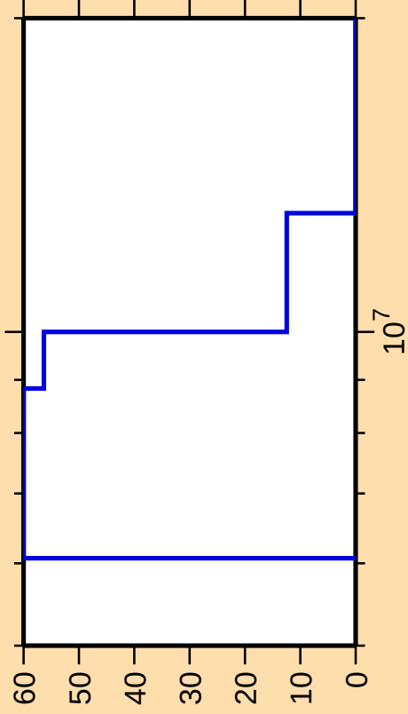
\Delta\sigma/\sigma vs. E for ^{244}\text{Bk}(n,n_1)
