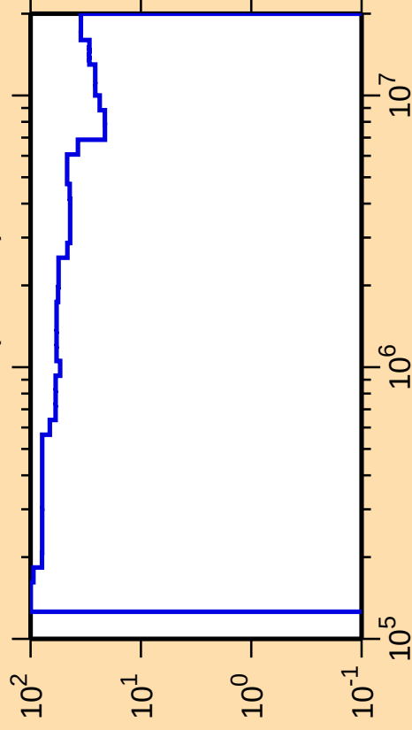
\Delta\sigma/\sigma vs. E for ^{244}\text{Bk}(n,\text{inel.})
