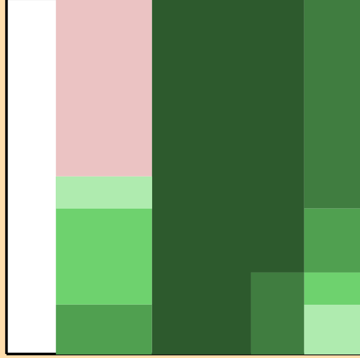
\Delta\sigma/\sigma vs. E for ^{244}\text{Bk}(n,2n)
