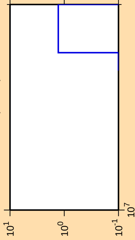
\Delta\sigma/\sigma vs. E for ^{244}\text{Bk}(\text{mt 11})
