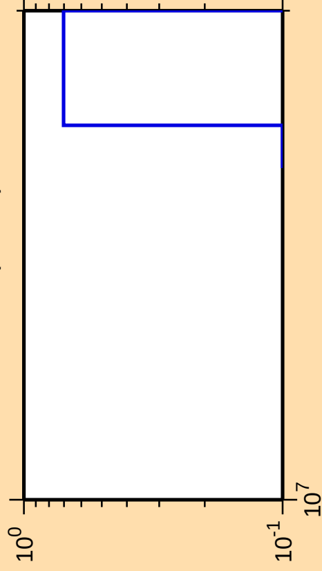
\Delta\sigma/\sigma vs. E for ^{244}\text{Bk}(\text{mt } 34)
