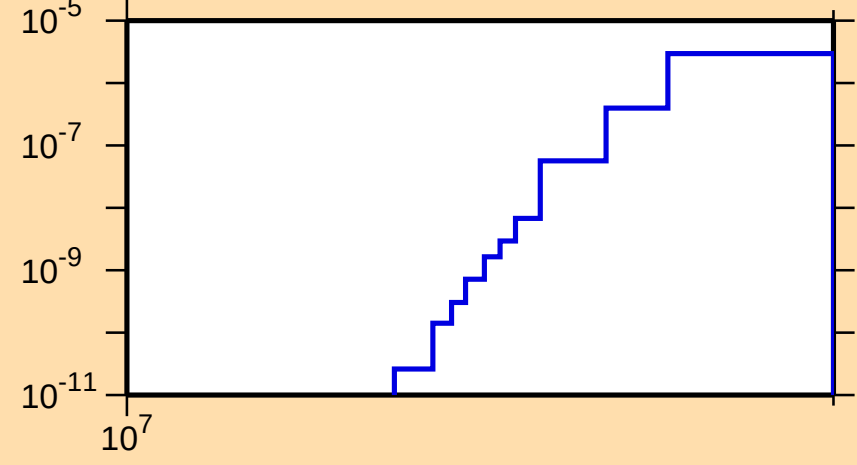
\sigma vs. E for ^{244}\text{Bk}(n,2np)
