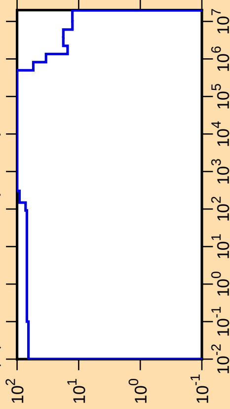
\Delta\mu/\mu vs. E for ^{244}\text{Bk}(\text{mt251})
