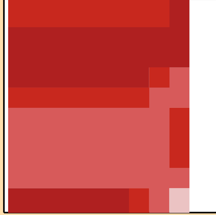
\Delta\sigma/\sigma vs. E for ^{244}\text{Bk}(n,n_1)
