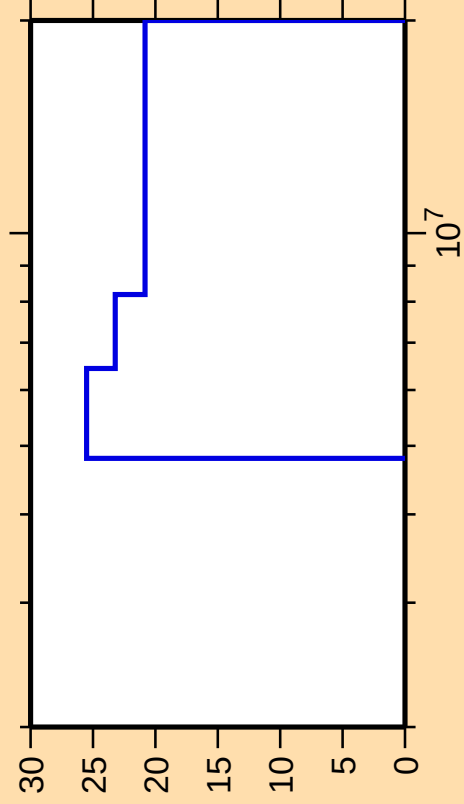
\Delta\sigma/\sigma vs. E for ^{244}\text{Bk}(n,f)
