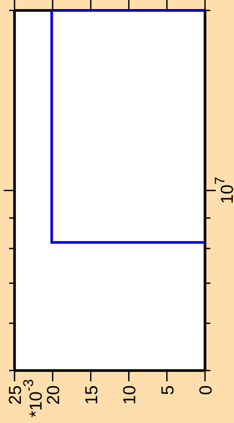
\Delta\sigma/\sigma vs. E for ^{244}\text{Bk}(n,3n\alpha)
