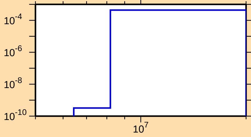
\sigma vs. E for ^{244}\text{Bk}(n,d)
