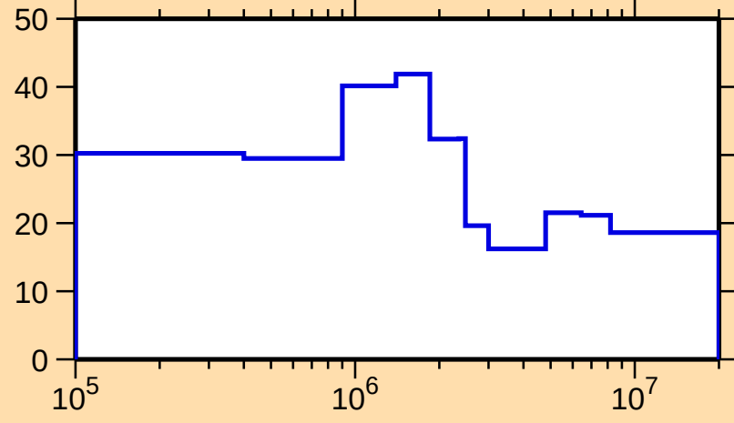
\Delta\sigma/\sigma vs. E for ^{244}\text{Bk}(n,n\text{onel.})
