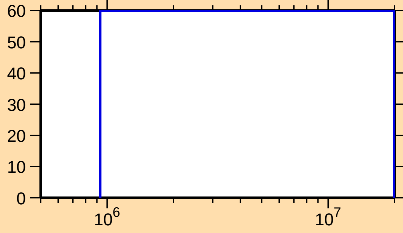
\Delta\sigma/\sigma vs. E for ^{238}\text{Cm}(n,\text{inel.})
