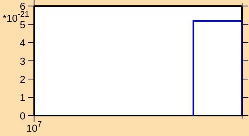
\sigma vs. E for ^{238}\text{Cm}(\text{mt } 42)
