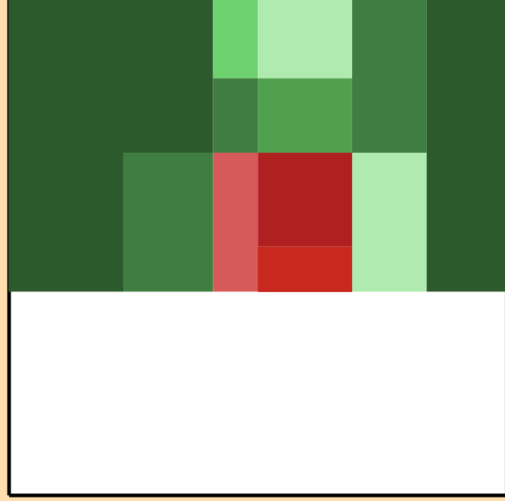
\Delta\sigma/\sigma vs. E for ^{238}\text{Cm}(n,\text{el.})
