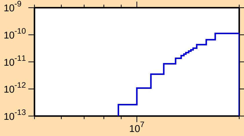
\sigma vs. E for ^{238}\text{Cm}(n,p\alpha)
