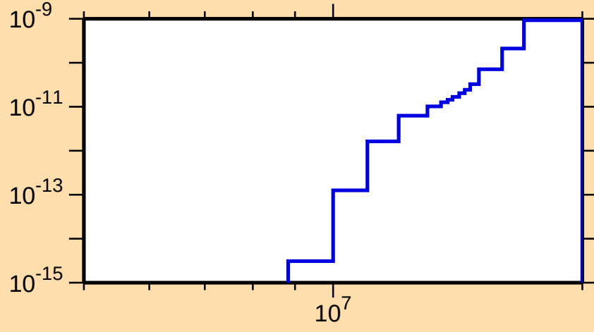
\sigma vs. E for ^{238}\text{Cm}(n,2n\alpha)
