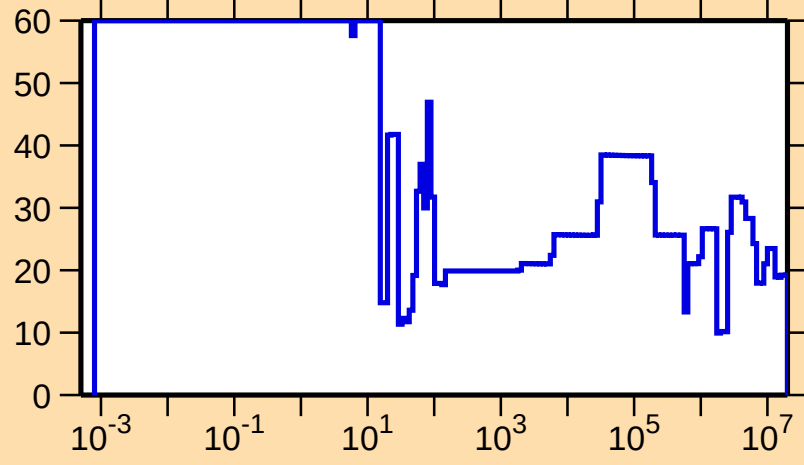
\Delta\sigma/\sigma vs. E for ^{238}\text{Cm}(n,el.)
