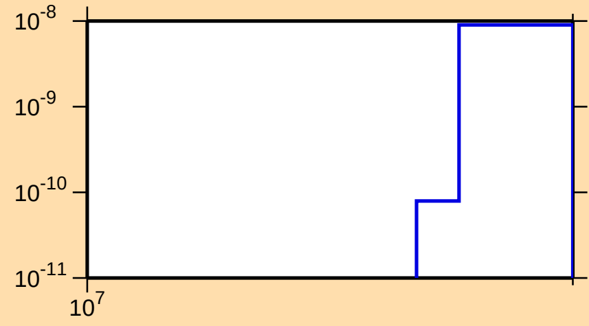
\sigma vs. E for ^{238}\text{Cm}(n,2np)
