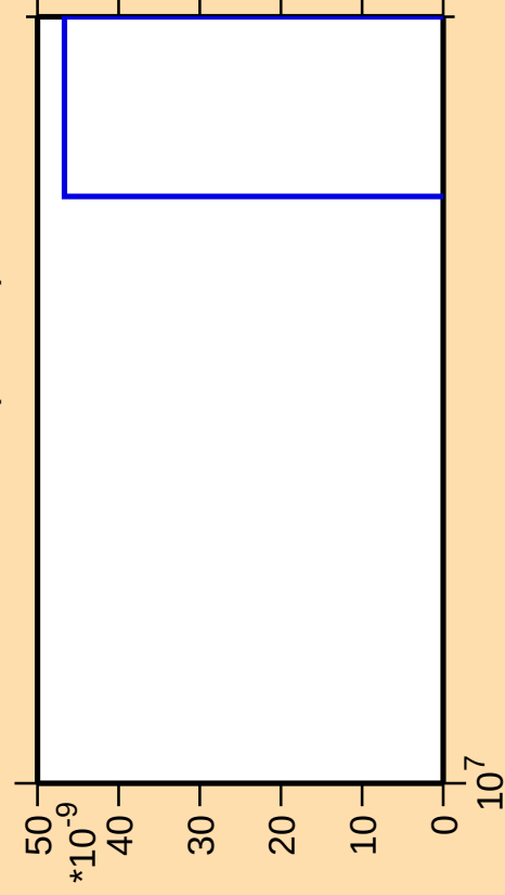
\Delta\sigma/\sigma vs. E for ^{238}\text{Cm}(\text{mt } 42)
