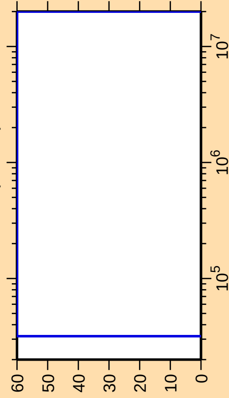
\Delta\sigma/\sigma vs. E for ^{238}\text{Cm}(n,\text{inel.})
