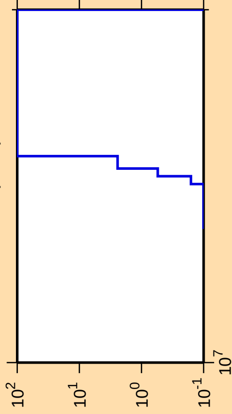
\Delta\sigma/\sigma vs. E for ^{238}\text{Cm}(n,\text{nd})
