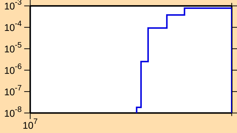
\sigma vs. E for ^{238}\text{Cm}(n,3n)
