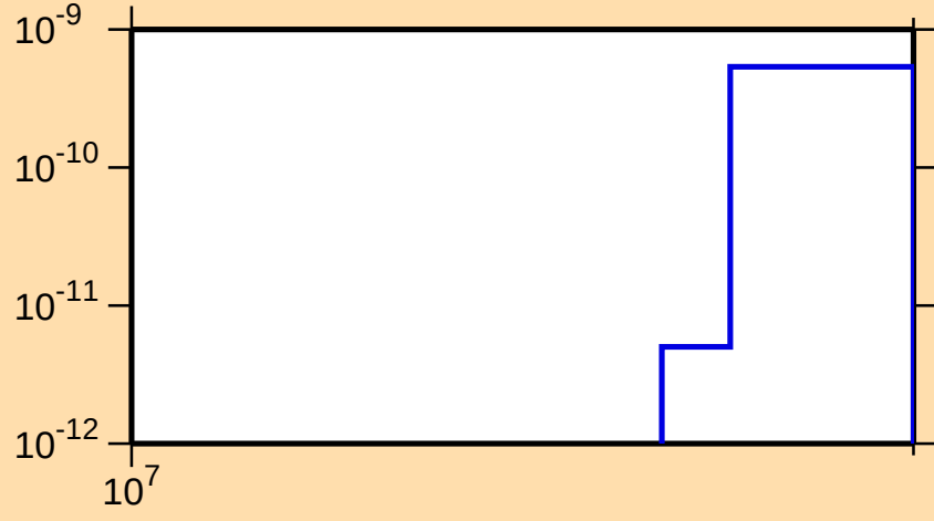
\sigma vs. E for ^{238}\text{Cm}(n,nt)
