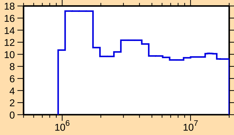
\Delta\sigma/\sigma vs. E for ^{238}\text{Cm}(n,\text{nonel.})
