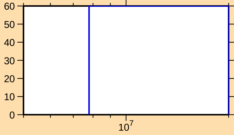
\Delta\sigma/\sigma vs. E for ^{238}\text{Cm}(n,2n)
