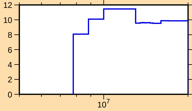
\Delta\sigma/\sigma vs. E for ^{238}\text{Cm}(n,\text{tot.})
