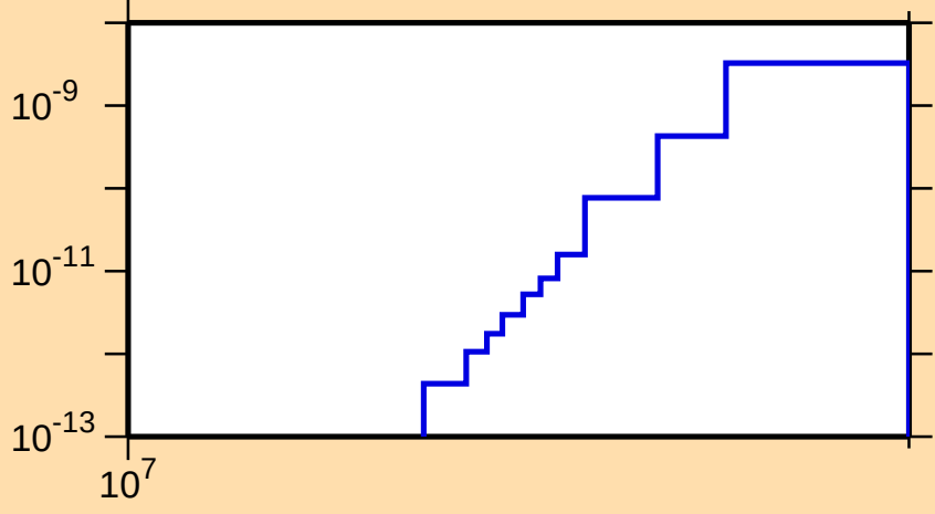
\sigma vs. E for ^{238}\text{Cm}(n,\text{He3})
