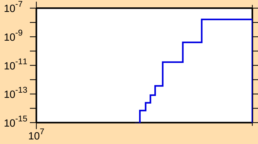
\sigma vs. E for ^{238}\text{Cm}(n,\text{nd})
