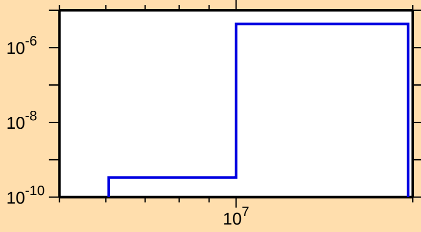
\sigma vs. E for ^{238}\text{Cm}(n,np)
