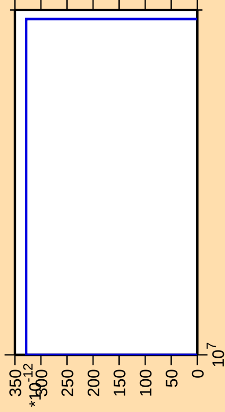
\Delta\sigma/\sigma vs. E for ^{238}\text{Cm}(\text{mt } 42)
