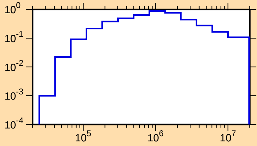
\sigma vs. E for ^{238}\text{Cm}(n,\text{inel.})
