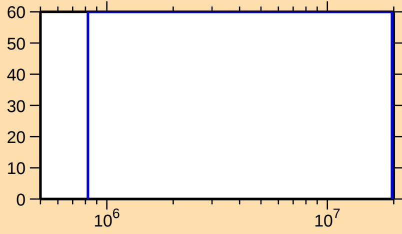
\Delta\sigma/\sigma vs. E for ^{238}\text{Cm}(n,ncont.)
