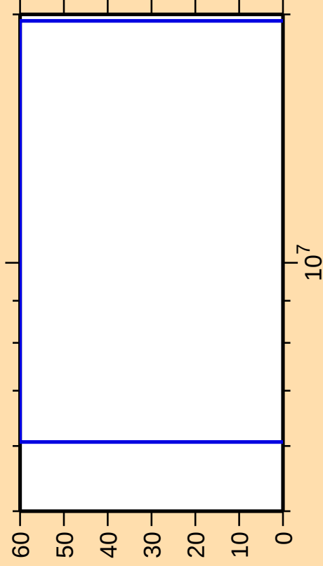
\Delta\sigma/\sigma vs. E for ^{238}\text{Cm}(n,np)
