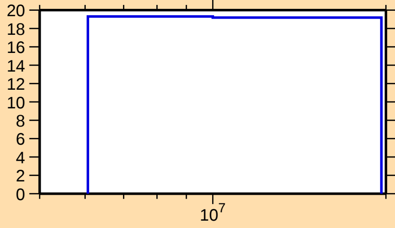
\Delta\sigma/\sigma vs. E for ^{238}\text{Cm}(n,\text{el.})
