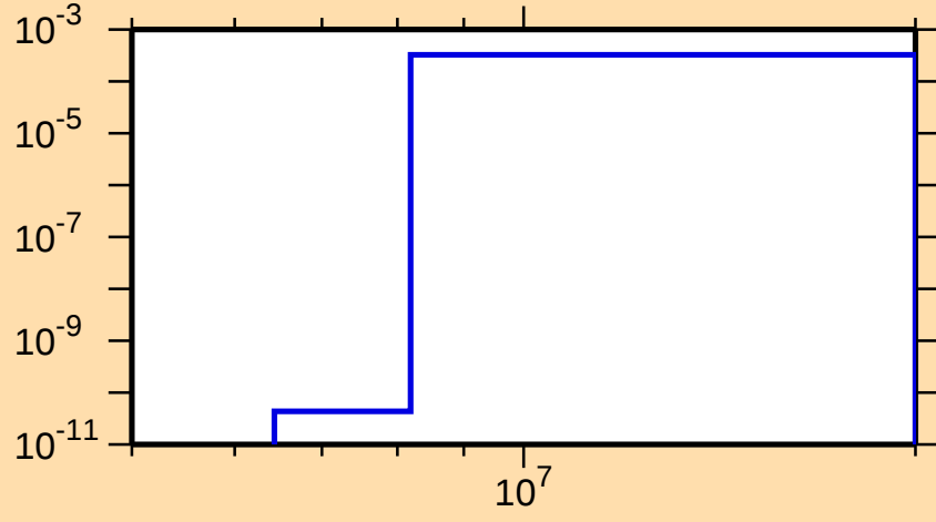
\sigma vs. E for ^{238}\text{Cm}(n,d)
