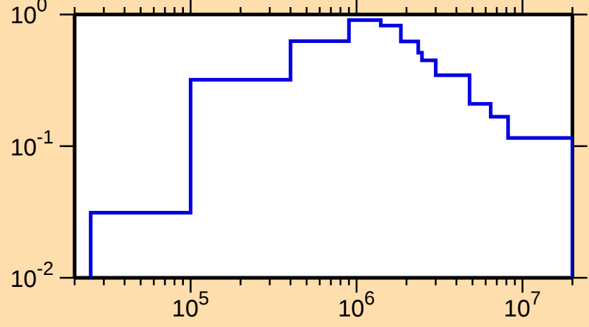
\sigma vs. E for ^{238}\text{Cm}(n,\text{inel.})
