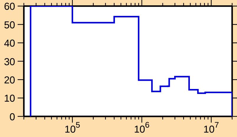
\Delta\sigma/\sigma vs. E for ^{238}\text{Cm}(n,f)
