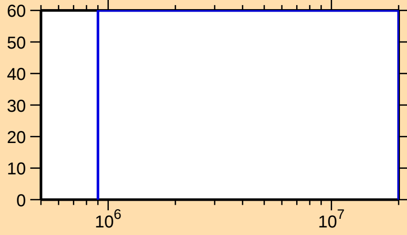
\Delta\sigma/\sigma vs. E for ^{238}\text{Cm}(n,n\text{cont.})
