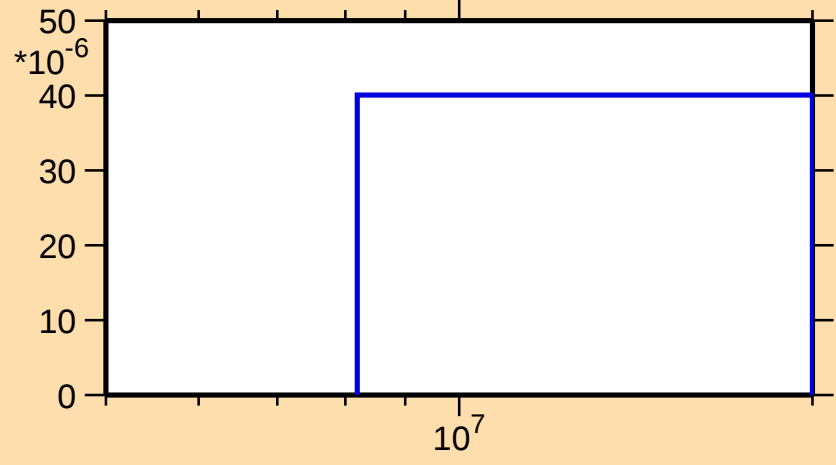
\sigma vs. E for ^{238}\text{Cm}(n,t)
