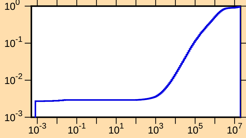
\mu vs. E for ^{249}\text{Cm}(\text{mt251})
