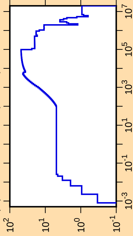
\Delta\mu/\mu vs. E for ^{249}\text{Cm}(\text{mt251})
