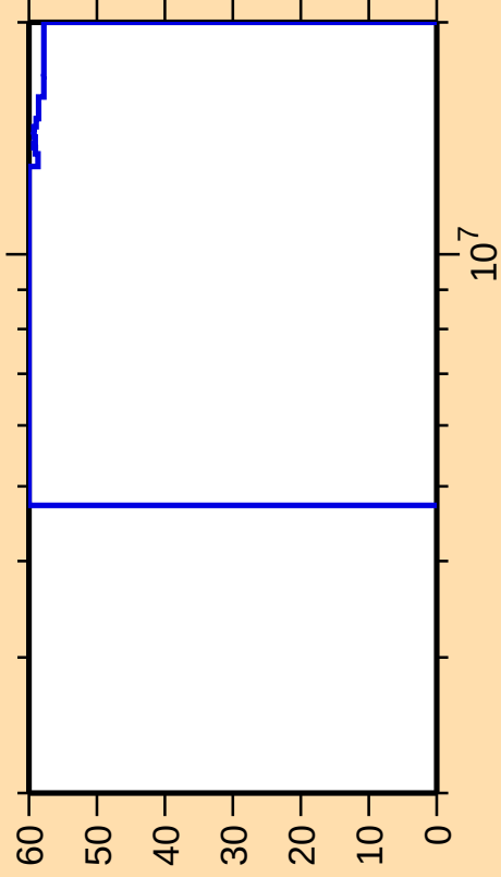
\Delta\sigma/\sigma vs. E for ^{249}\text{Cm}(n,n\text{cont.})
