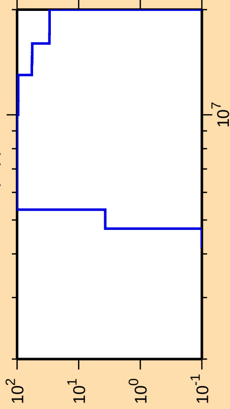
\Delta\sigma/\sigma vs. E for ^{249}\text{Cm}(n,p)
