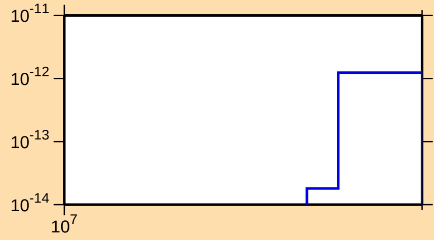
\sigma vs. E for ^{249}\text{Cm}(n,\text{He3})
