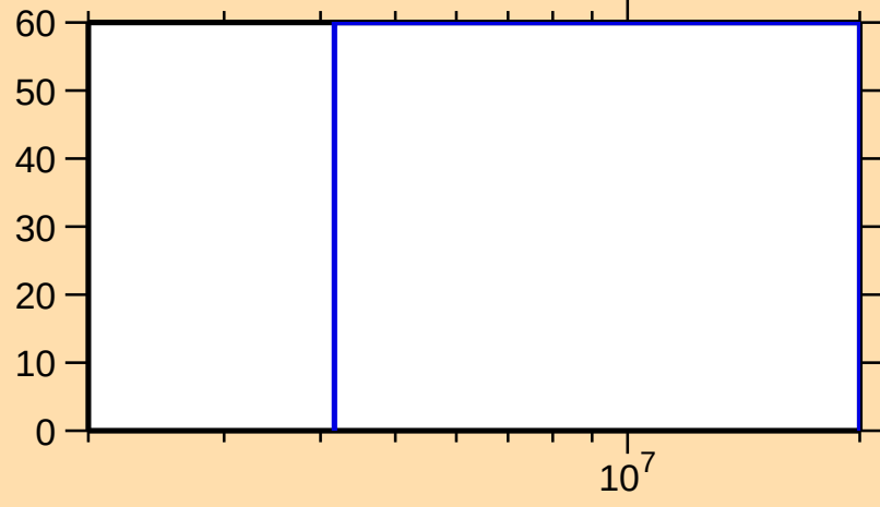
\Delta\sigma/\sigma vs. E for ^{249}\text{Cm}(n,\gamma)
