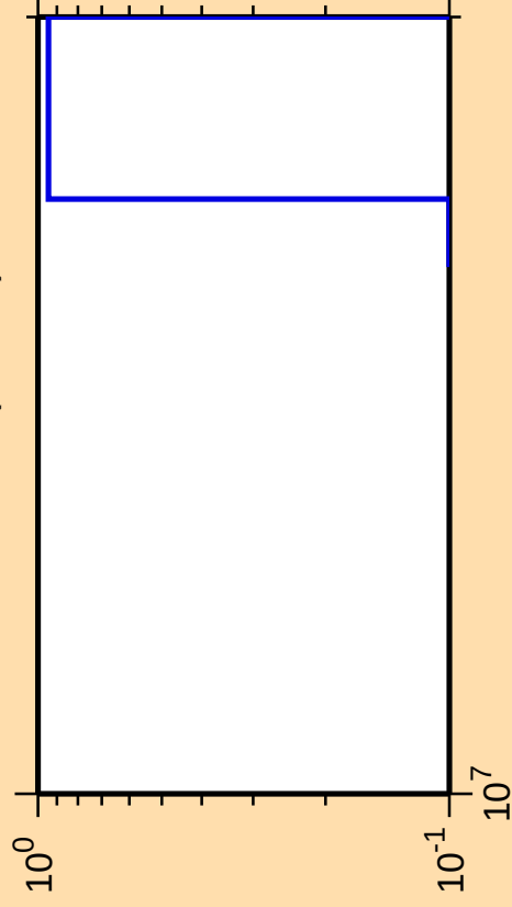
\Delta\sigma/\sigma vs. E for ^{249}\text{Cm}(n,\text{He3})
