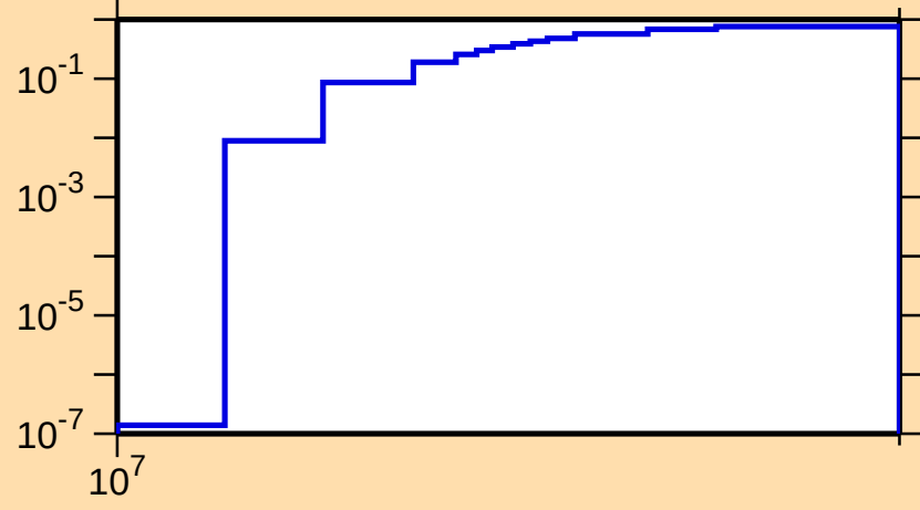
\sigma vs. E for ^{249}\text{Cm}(n,3n)
