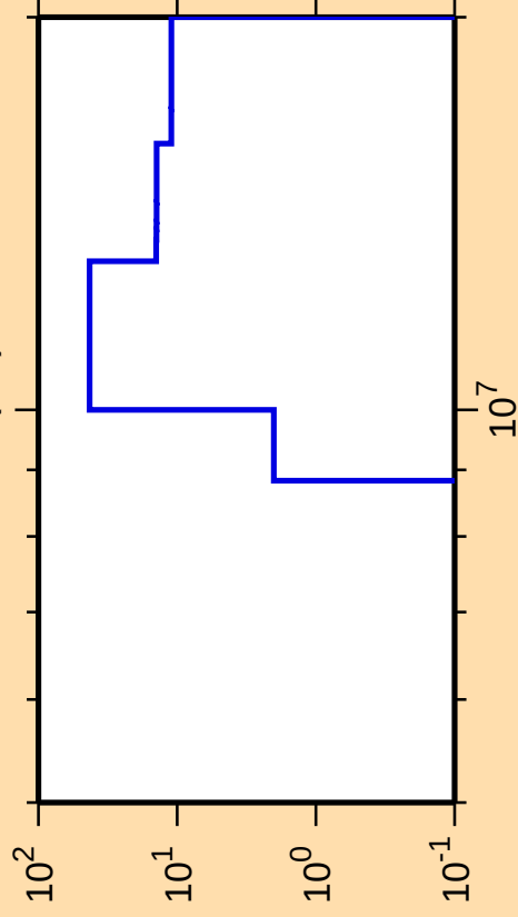
\Delta\sigma/\sigma vs. E for ^{249}\text{Cm}(n,t)
