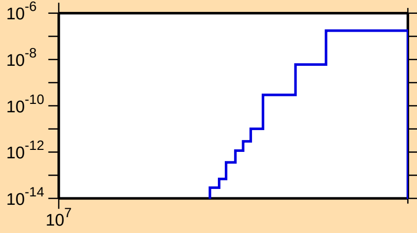
\sigma vs. E for ^{249}\text{Cm}(n,nt)
