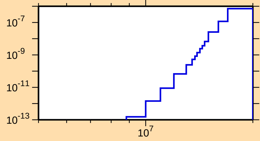
\sigma vs. E for ^{249}\text{Cm}(n,2n\alpha)
