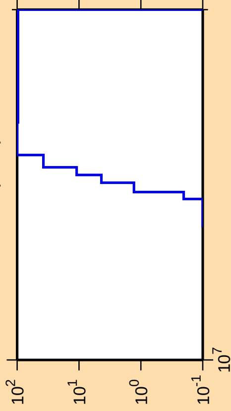
\Delta\sigma/\sigma vs. E for ^{249}\text{Cm}(n,\text{nd})
