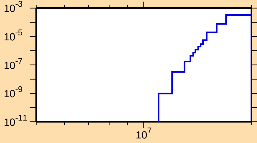
\sigma vs. E for ^{249}\text{Cm}(n,np)
