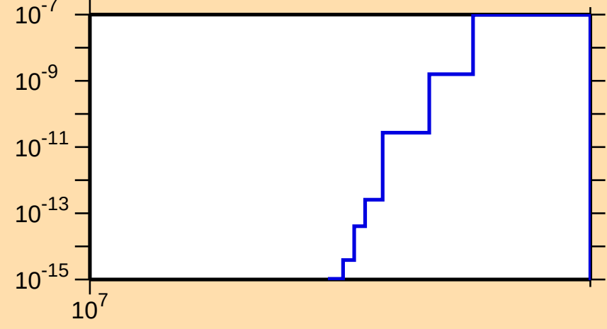
\sigma vs. E for ^{249}\text{Cm}(n,2np)
