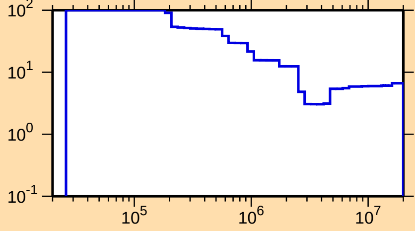
\Delta\sigma/\sigma vs. E for ^{249}\text{Cm}(n,\text{nonel.})
