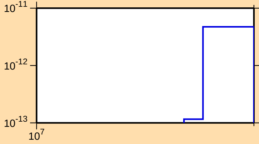
\sigma vs. E for ^{249}\text{Cm}(n,3n\alpha)
