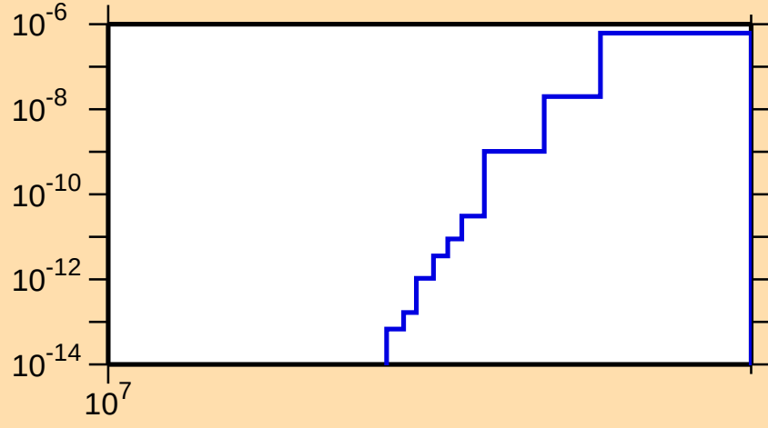
\sigma vs. E for ^{249}\text{Cm}(n,\text{nd})
