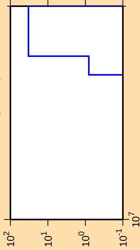
\Delta\sigma/\sigma vs. E for ^{249}\text{Cm}(n,3n\alpha)
