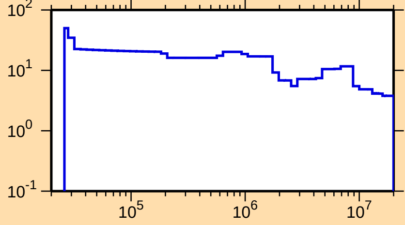
\Delta\sigma/\sigma vs. E for ^{249}\text{Cm}(n,\text{el.})
