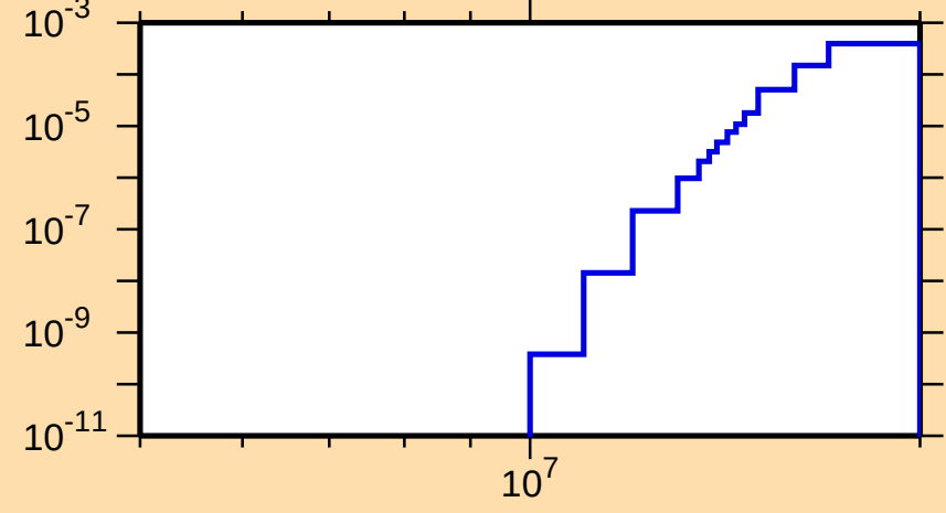
\sigma vs. E for ^{249}\text{Cm}(n,t)
