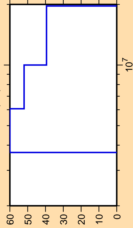
\Delta\sigma/\sigma vs. E for ^{249}\text{Cm}(n,f)
