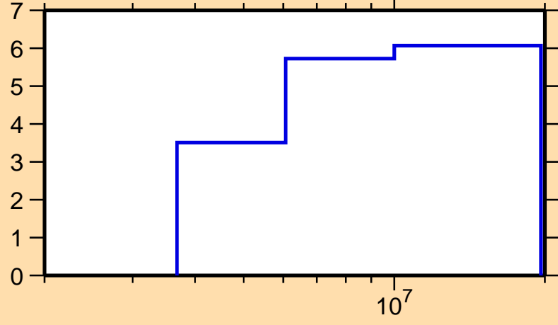
\Delta\sigma/\sigma vs. E for ^{249}\text{Cm}(n,\text{nonel.})
