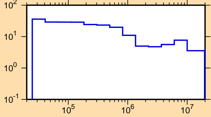
\Delta\sigma/\sigma vs. E for ^{249}\text{Cm}(n,\text{tot.})
