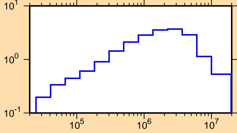
\sigma vs. E for ^{249}\text{Cm}(n,\text{inel.})
