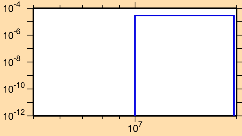
\sigma vs. E for ^{249}\text{Cm}(n,d)
