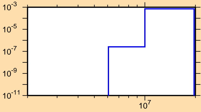
\sigma vs. E for ^{249}\text{Cm}(n,p)
