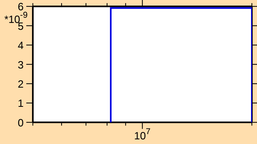
\sigma vs. E for ^{249}\text{Cm}(n,nd)
