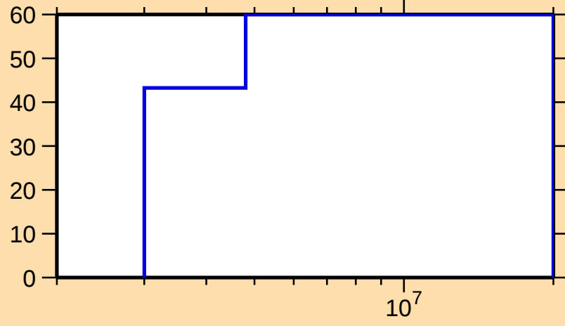
\Delta\sigma/\sigma vs. E for ^{249}\text{Cm}(n,n\text{cont.})
