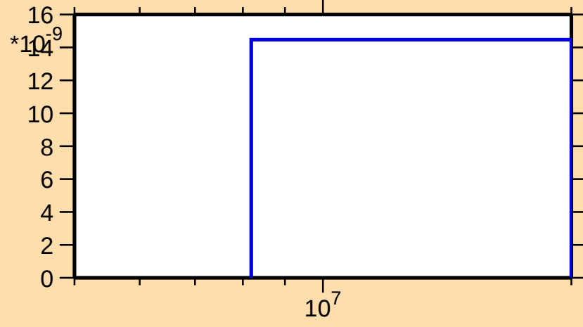
\sigma vs. E for ^{249}\text{Cm}(n,2n\alpha)
