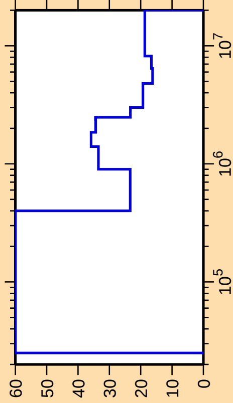
\Delta\sigma/\sigma vs. E for ^{249}\text{Cm}(n,n_1)
