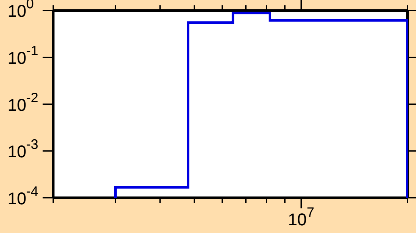
\sigma vs. E for ^{249}\text{Cm}(n,2n)
