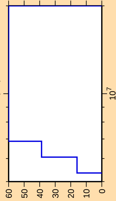
\Delta\sigma/\sigma vs. E for ^{252}\text{Cm}(n,f)
