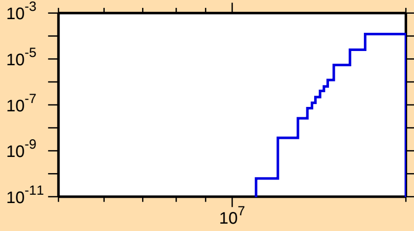
\sigma vs. E for ^{252}\text{Cm}(n,np)
