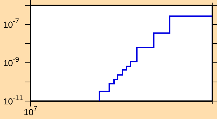
\sigma vs. E for ^{252}\text{Cm}(n,2n\alpha)
