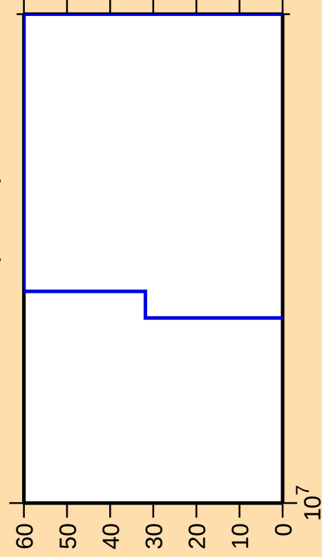
\Delta\sigma/\sigma vs. E for ^{252}\text{Cm}(n,2n\alpha)
