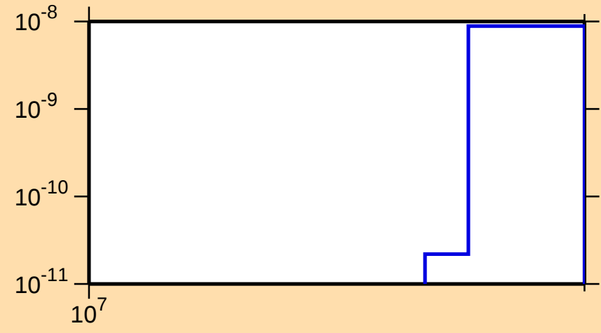
\sigma vs. E for ^{252}\text{Cm}(n,2np)
