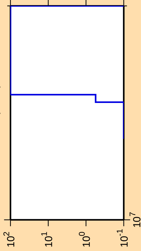
\Delta\sigma/\sigma vs. E for ^{252}\text{Cm}(n,\text{nd})
