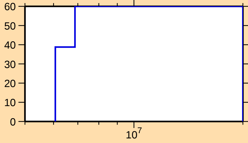
\Delta\sigma/\sigma vs. E for ^{252}\text{Cm}(n,f)
