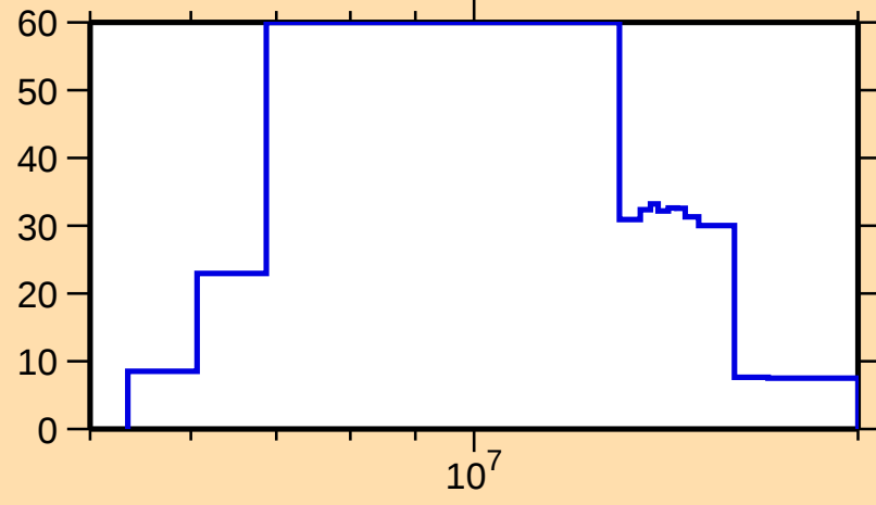
\Delta\sigma/\sigma vs. E for ^{252}\text{Cm}(n,\text{el.})
