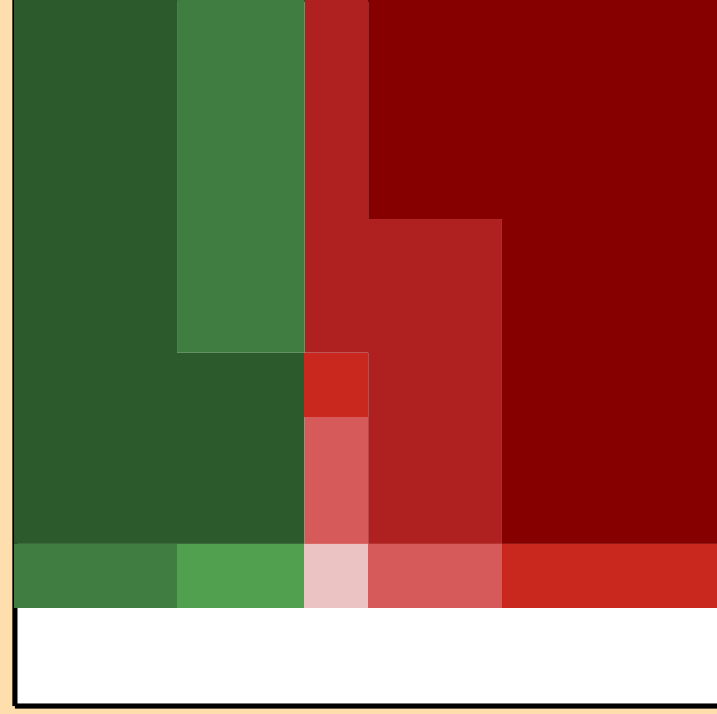
\Delta\sigma/\sigma vs. E for ^{252}\text{Cm}(n,\text{nonel.})
