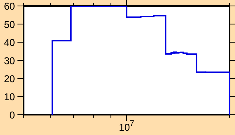
\Delta\sigma/\sigma vs. E for ^{252}\text{Cm}(n,\text{inel.})
