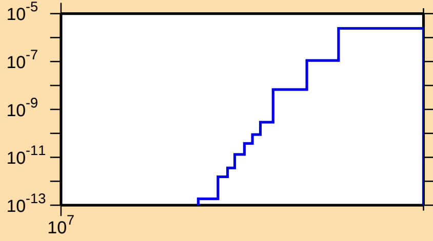
\sigma vs. E for ^{252}\text{Cm}(n,nt)
