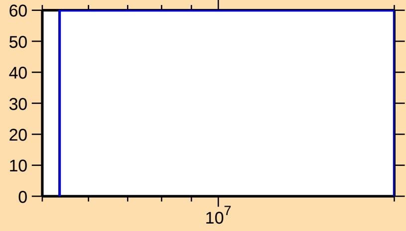
\Delta\sigma/\sigma vs. E for ^{252}\text{Cm}(n,2n)
