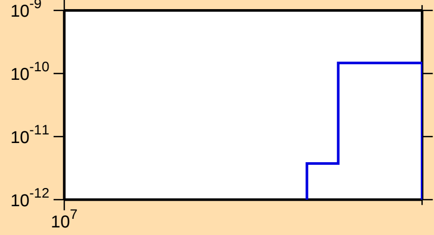
\sigma vs. E for ^{252}\text{Cm}(n,3n\alpha)
