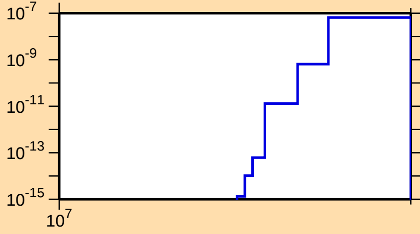
\sigma vs. E for ^{252}\text{Cm}(n,\text{nd})
