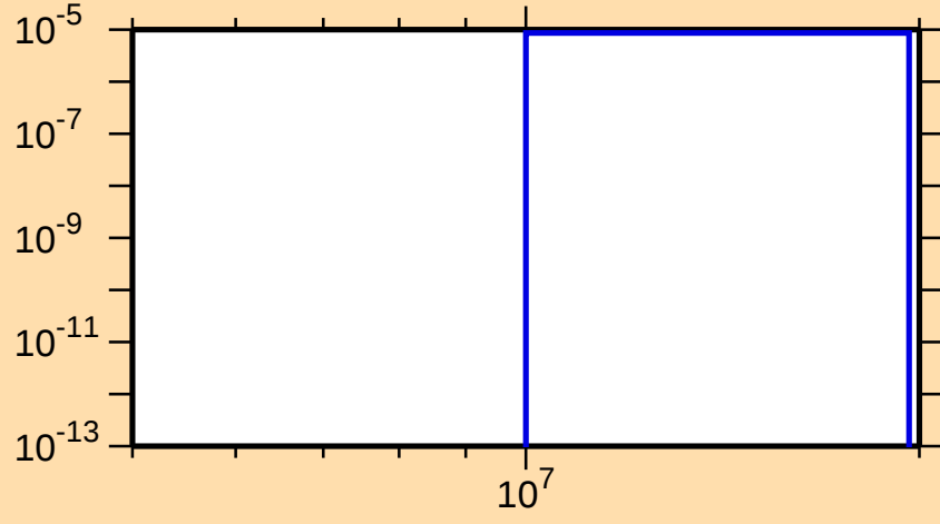
\sigma vs. E for ^{252}\text{Cm}(n,d)
