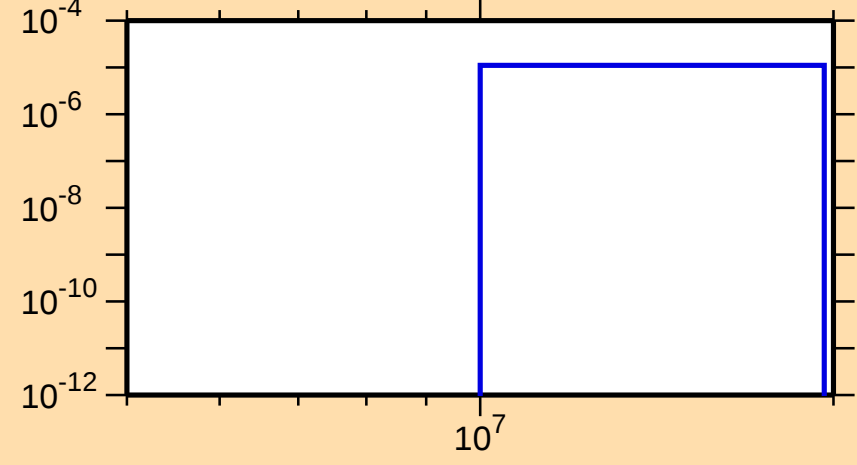
\sigma vs. E for ^{252}\text{Cm}(n,t)
