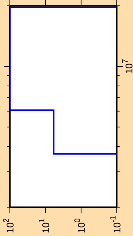
\Delta\sigma/\sigma vs. E for ^{252}\text{Cm}(n,n\alpha)
