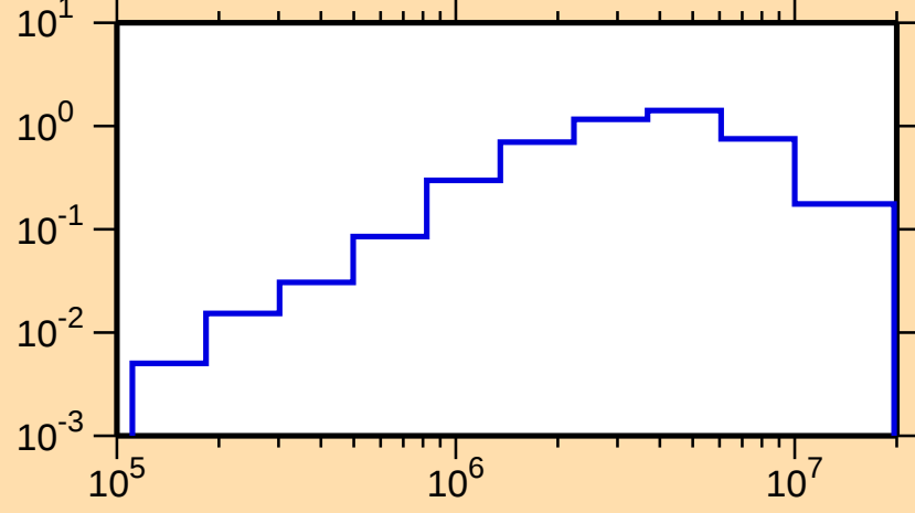
\sigma vs. E for ^{252}\text{Cm}(n,n\text{cont.})
