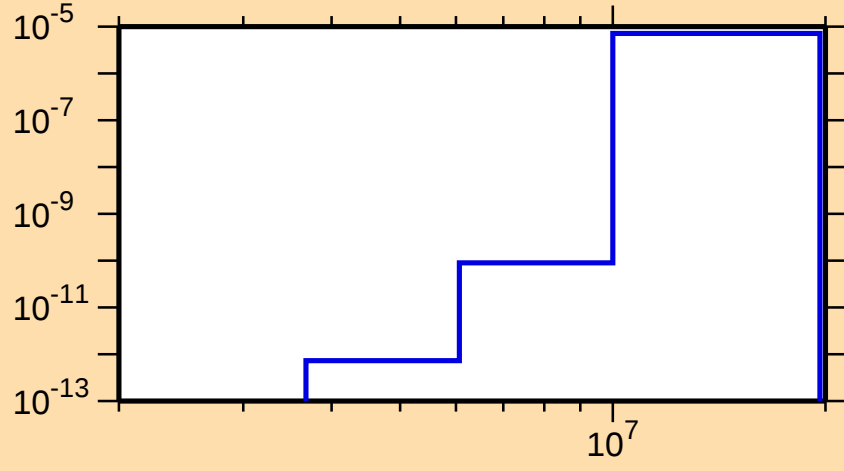
\sigma vs. E for ^{252}\text{Cm}(n,n\alpha)
