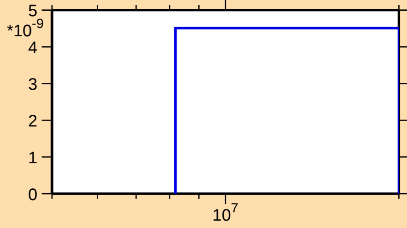
\sigma vs. E for ^{252}\text{Cm}(n,2n\alpha)
