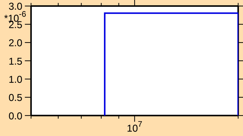
\sigma vs. E for ^{252}\text{Cm}(n,np)
