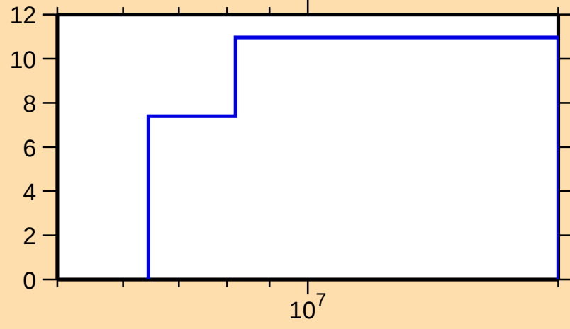
\Delta\sigma/\sigma vs. E for ^{252}\text{Cm}(n,\text{nonel.})
