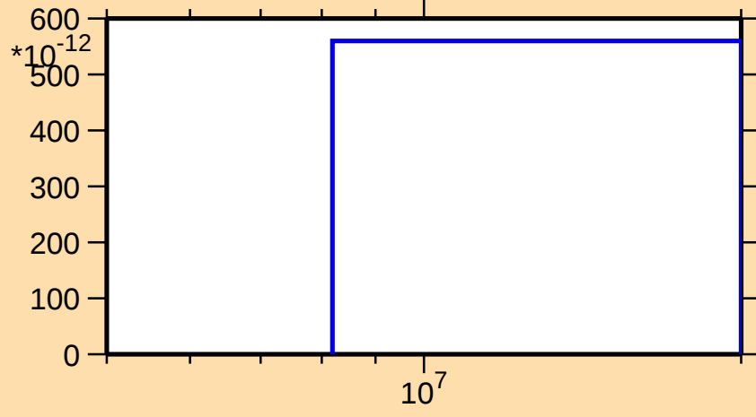
\sigma vs. E for ^{252}\text{Cm}(n,nd)
