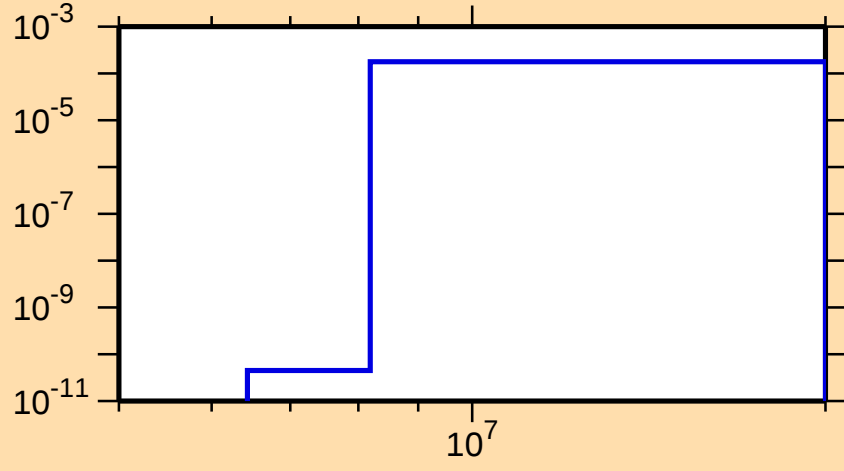
\sigma vs. E for ^{252}\text{Cm}(n,p)
