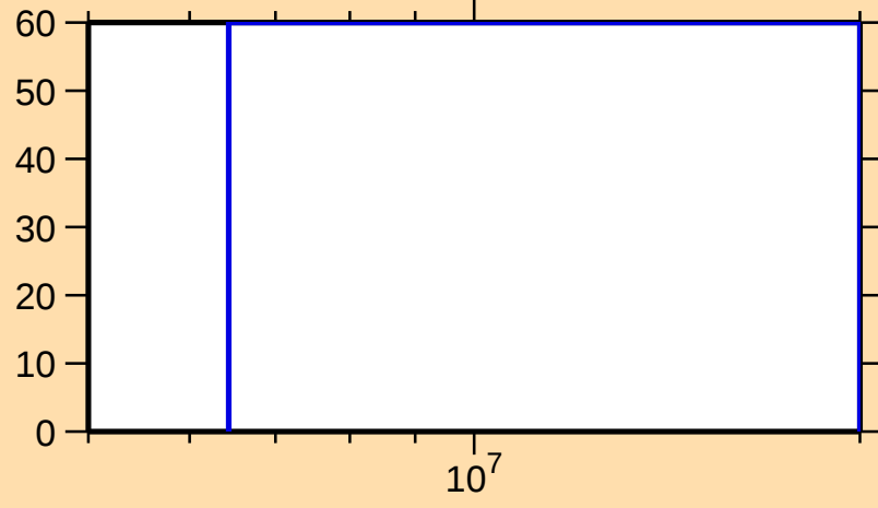
\Delta\sigma/\sigma vs. E for ^{252}\text{Cm}(n,p)
