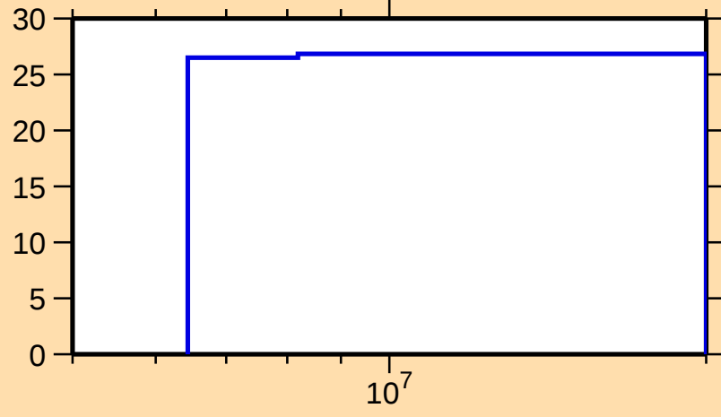
\Delta\sigma/\sigma vs. E for ^{252}\text{Cm}(n,\text{tot.})
