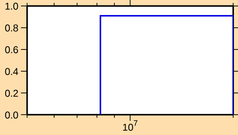
\sigma vs. E for ^{252}\text{Cm}(n,3n)
