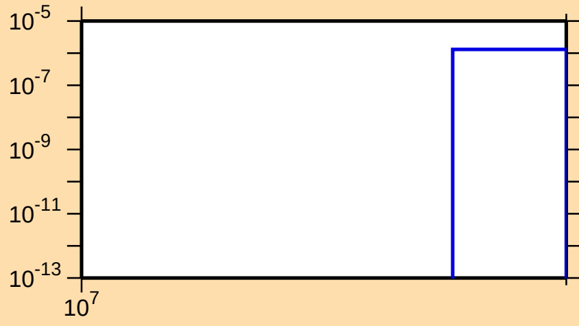
\sigma vs. E for ^{144}\text{Dy}(n,2np)
