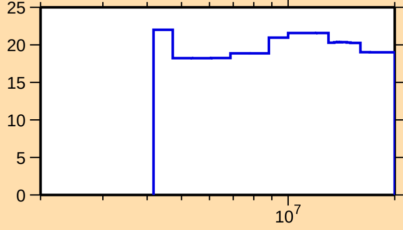
\Delta\sigma/\sigma vs. E for ^{144}\text{Dy}(n,n\text{nonel.})
