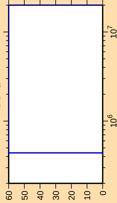
\Delta\sigma/\sigma vs. E for ^{144}\text{Dy}(n,\gamma)
