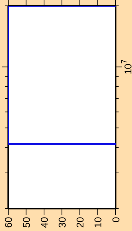
\Delta\sigma/\sigma vs. E for ^{144}\text{Dy}(n,\text{ncont.})
