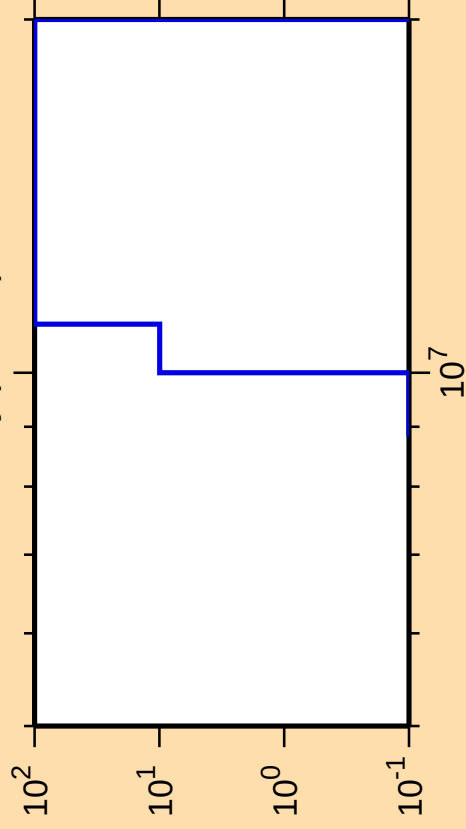
\Delta\sigma/\sigma vs. E for ^{144}\text{Dy}(\text{mt } 45)
