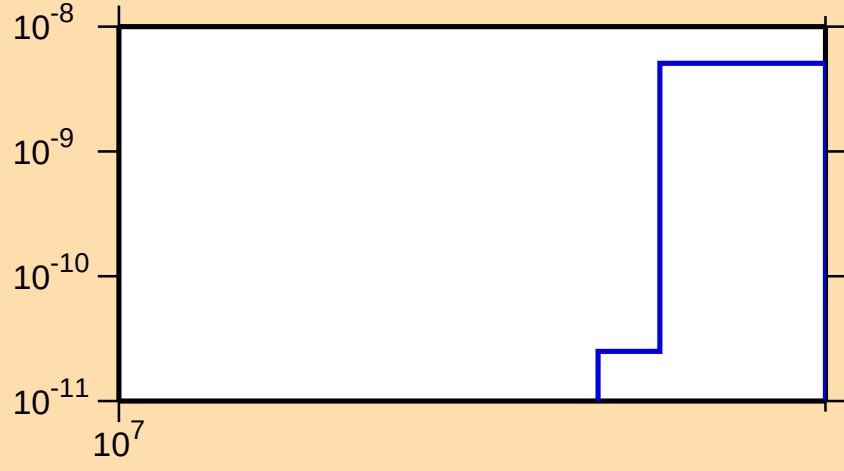
\sigma vs. E for ^{144}\text{Dy}(n,2n\alpha)
