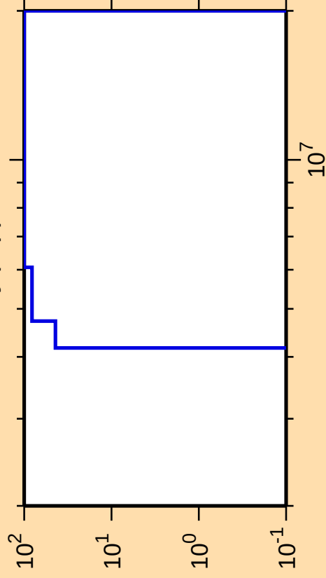
\Delta\sigma/\sigma vs. E for ^{144}\text{Dy}(n,p)
