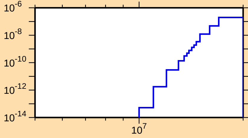
\sigma vs. E for ^{144}\text{Dy}(\text{mt117})
