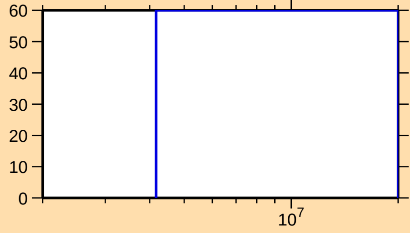
\Delta\sigma/\sigma vs. E for ^{144}\text{Dy}(n,n\text{cont.})
