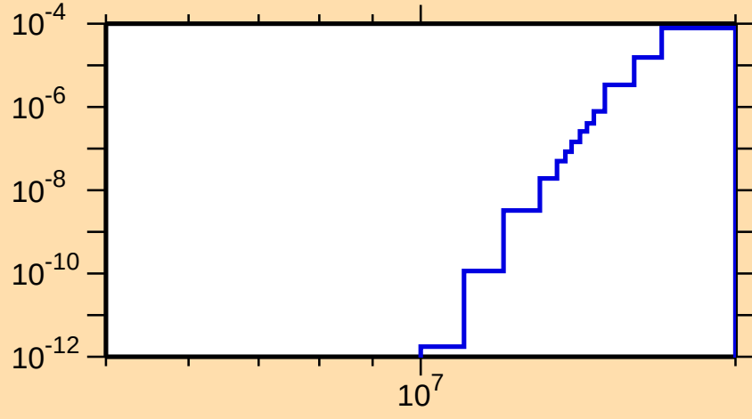
\sigma vs. E for ^{144}\text{Dy}(\text{mt } 45)
