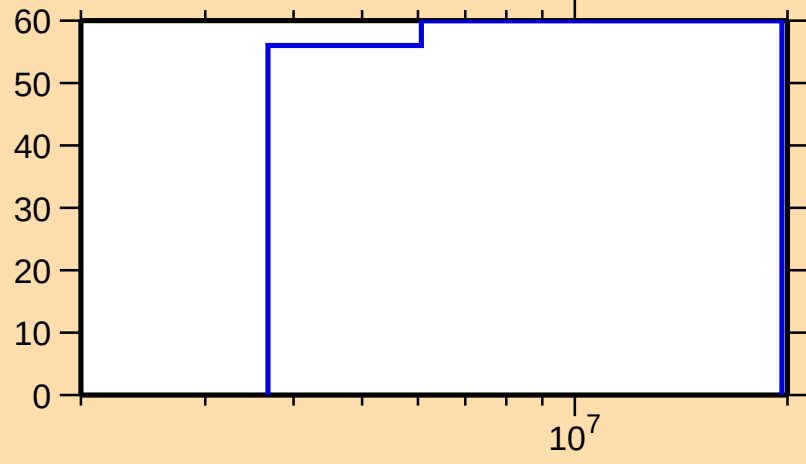
\Delta\sigma/\sigma vs. E for ^{144}\text{Dy}(\text{n},\text{el.})
