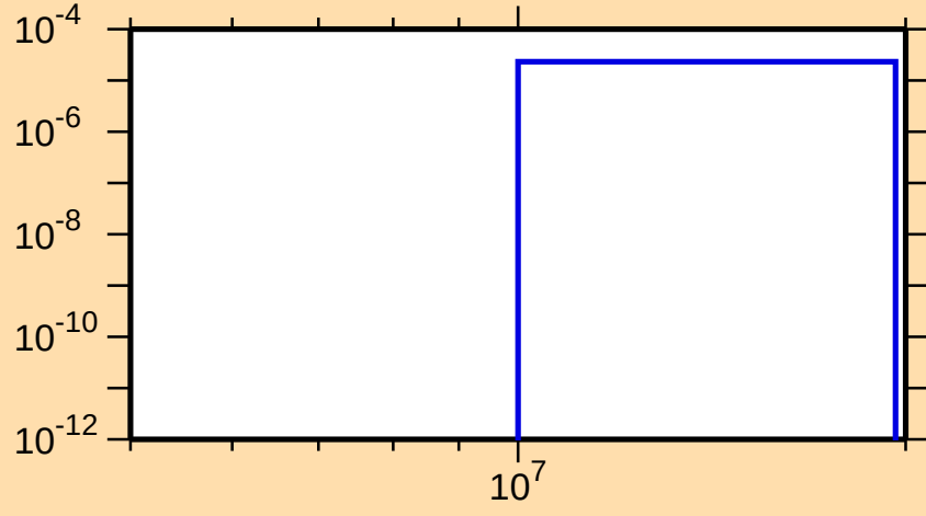
\sigma vs. E for ^{144}\text{Dy}(n,t)
