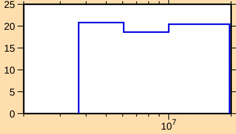
\Delta\sigma/\sigma vs. E for ^{144}\text{Dy}(\text{n},\text{nonel.})
