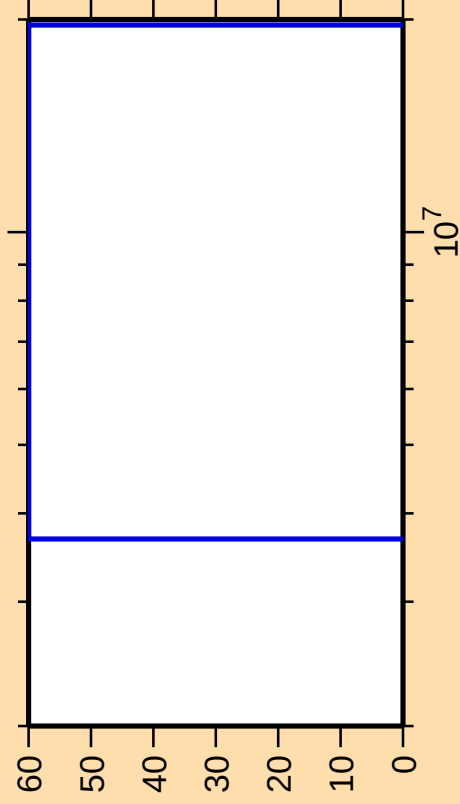
\Delta\sigma/\sigma vs. E for ^{144}\text{Dy}(\text{n},\text{ncont.})
