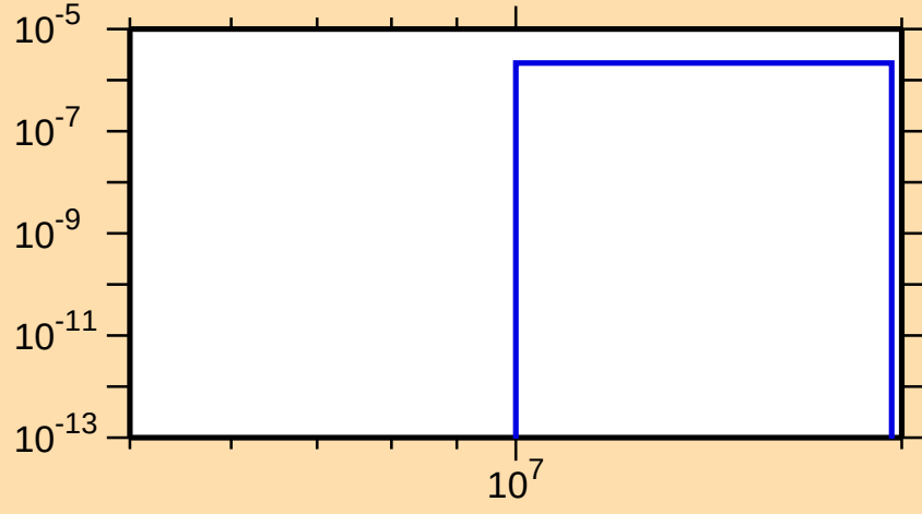
\sigma vs. E for ^{144}\text{Dy} (mt 45)
