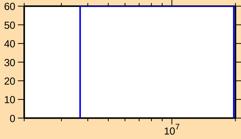
\Delta\sigma/\sigma vs. E for ^{144}\text{Dy}(\text{n},\text{inel.})
