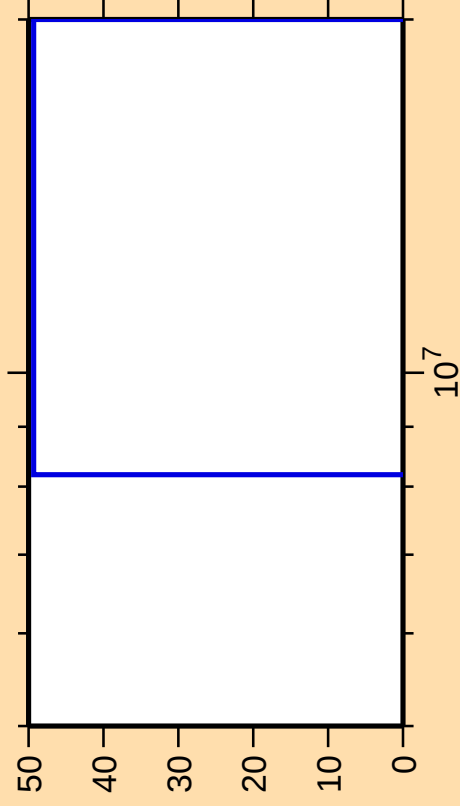
\Delta\sigma/\sigma vs. E for ^{144}\text{Dy}(\text{mt } 34)
