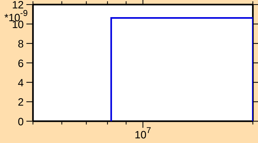
\sigma vs. E for ^{144}\text{Dy}(n,2np)
