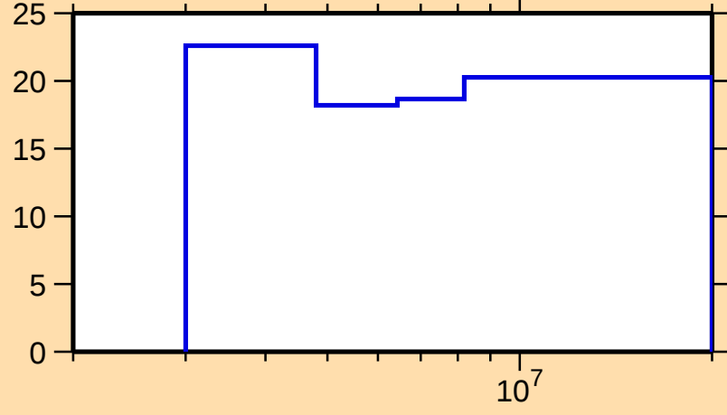
\Delta\sigma/\sigma vs. E for ^{144}\text{Dy}(n,n\text{onel.})
