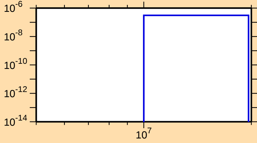
\sigma vs. E for ^{145}\text{Dy}(\text{mt } 45)
