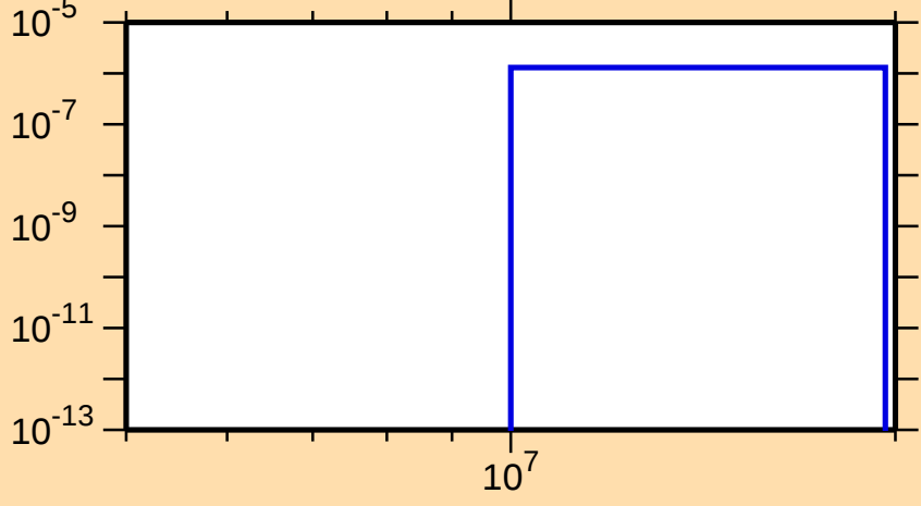
\sigma vs. E for ^{145}\text{Dy}(n,\text{pt})
