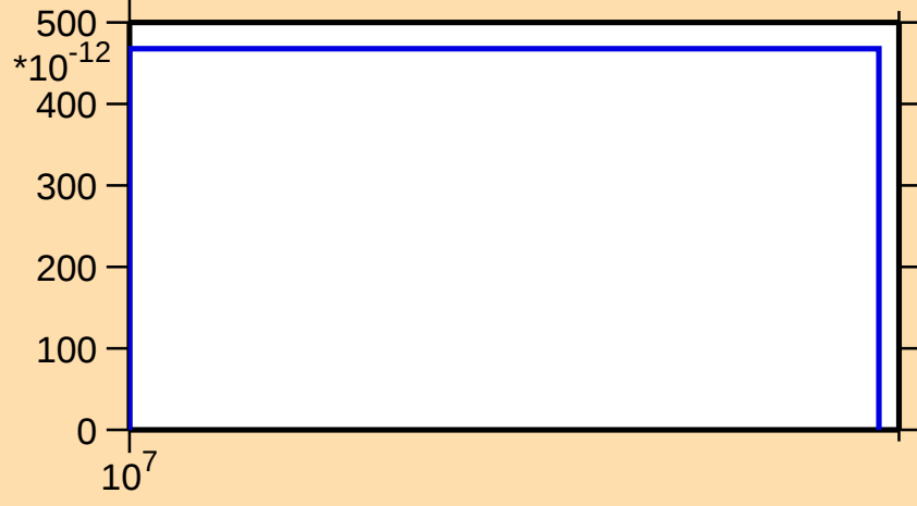
\sigma vs. E for ^{145}\text{Dy}(\text{mt } 34)
