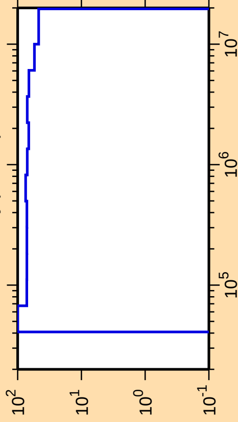
\Delta\sigma/\sigma vs. E for ^{145}\text{Dy}(n,\text{inel.})
