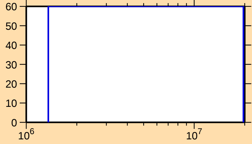
\Delta\sigma/\sigma vs. E for ^{145}\text{Dy}(n,n\text{cont.})
