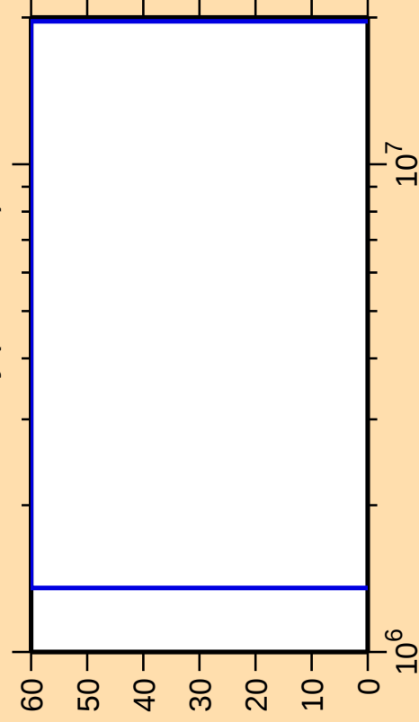
\Delta\sigma/\sigma vs. E for ^{145}\text{Dy}(n,\text{ncont.})
