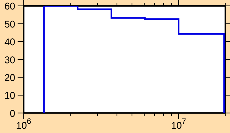
\Delta\sigma/\sigma vs. E for ^{145}\text{Dy}(n,n_1)
