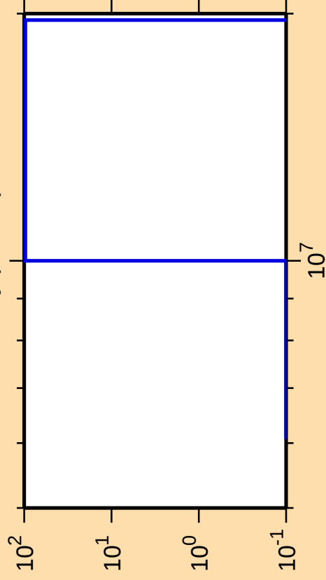
\Delta\sigma/\sigma vs. E for ^{145}\text{Dy}(\text{mt } 45)
