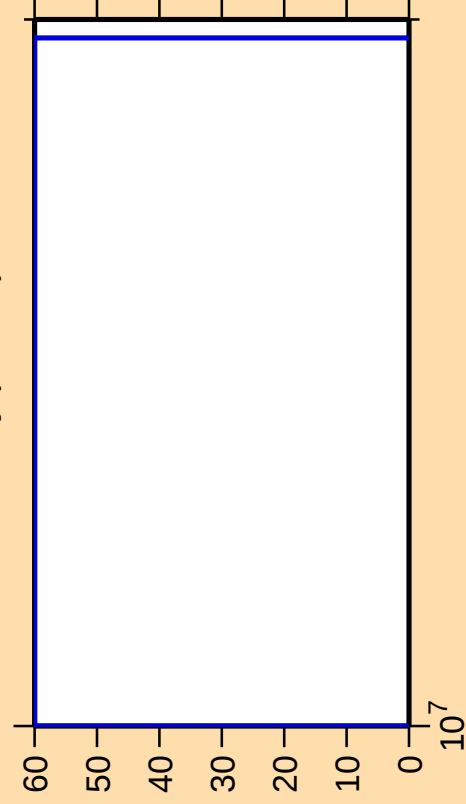
\Delta\sigma/\sigma vs. E for ^{145}\text{Dy}(\text{mt } 34)
