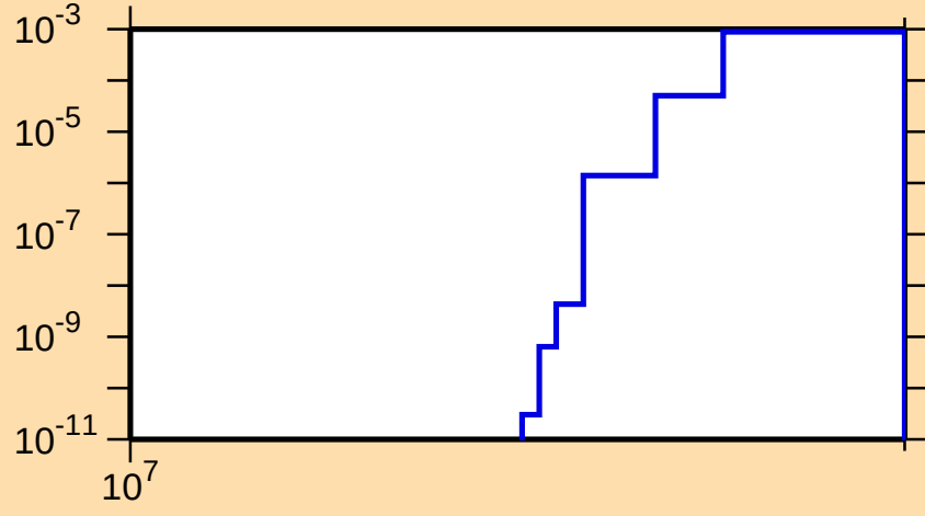
\sigma vs. E for ^{151}\text{Dy}(n,2np)
