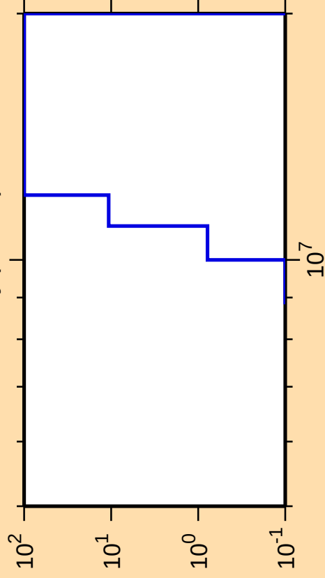
\Delta\sigma/\sigma vs. E for ^{151}\text{Dy}(\text{mt } 45)
