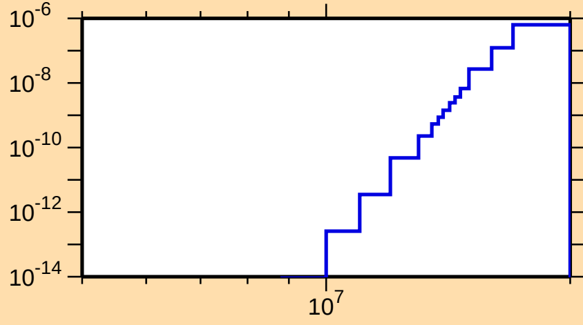
\sigma vs. E for ^{151}\text{Dy}(\text{mt } 45)
