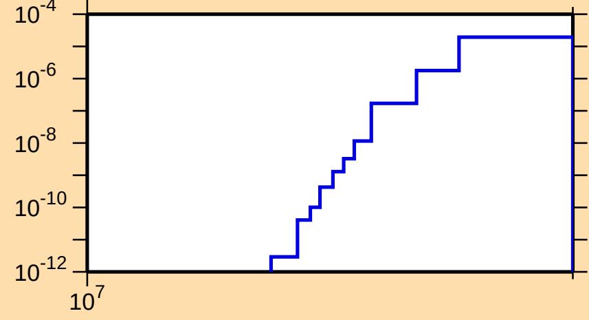
\sigma vs. E for ^{151}\text{Dy}(n,nd)
