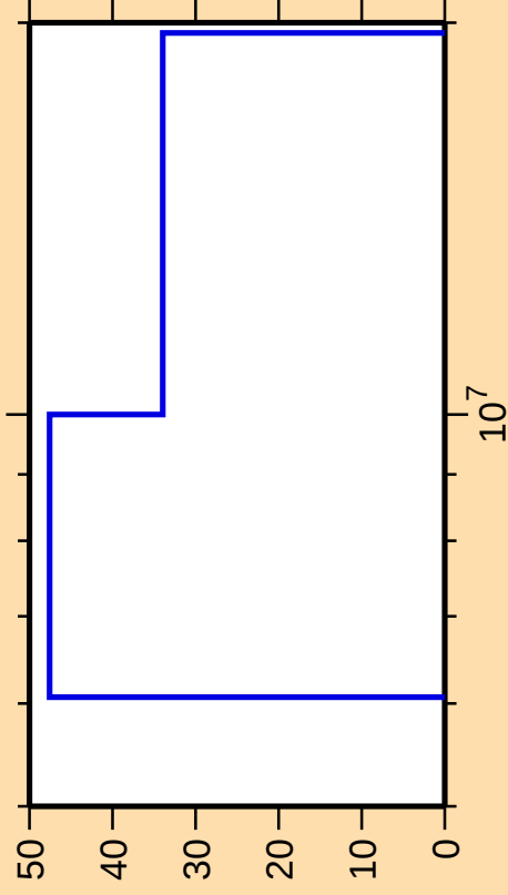
\Delta\sigma/\sigma vs. E for ^{151}\text{Dy}(n,2n)
