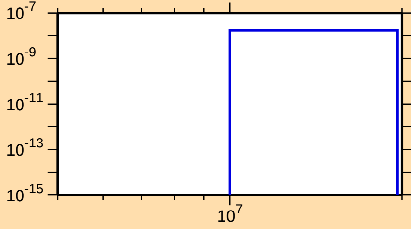
\sigma vs. E for ^{151}\text{Dy} (mt 45)
