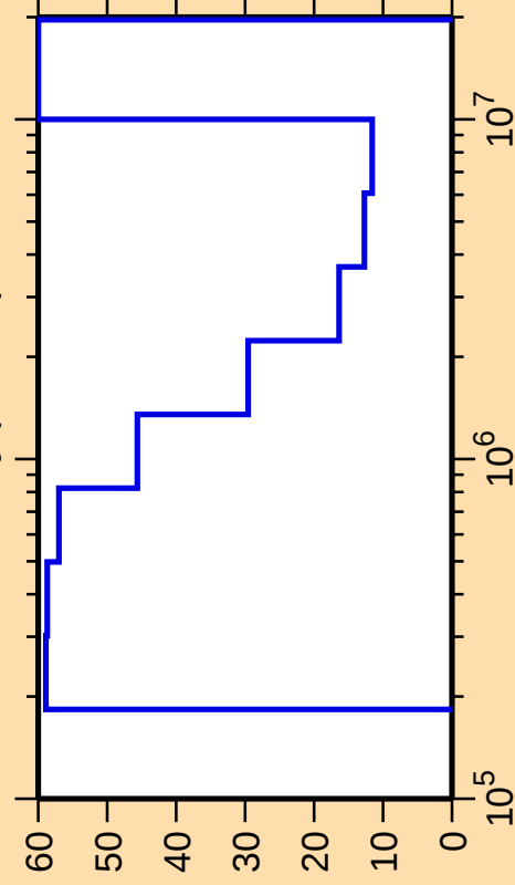
\Delta\sigma/\sigma vs. E for ^{151}\text{Dy}(n,\text{inel.})
