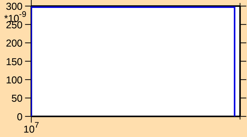
\sigma vs. E for ^{151}\text{Dy}(n,\text{nd})
