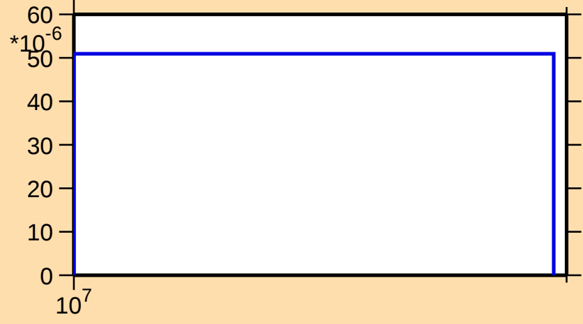
\sigma vs. E for ^{151}\text{Dy}(n,3n)
