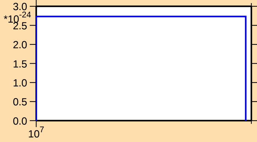
\sigma vs. E for ^{151}\text{Dy} (mt 11)
