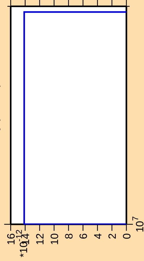
\Delta\sigma/\sigma vs. E for ^{151}\text{Dy} (mt 11)
