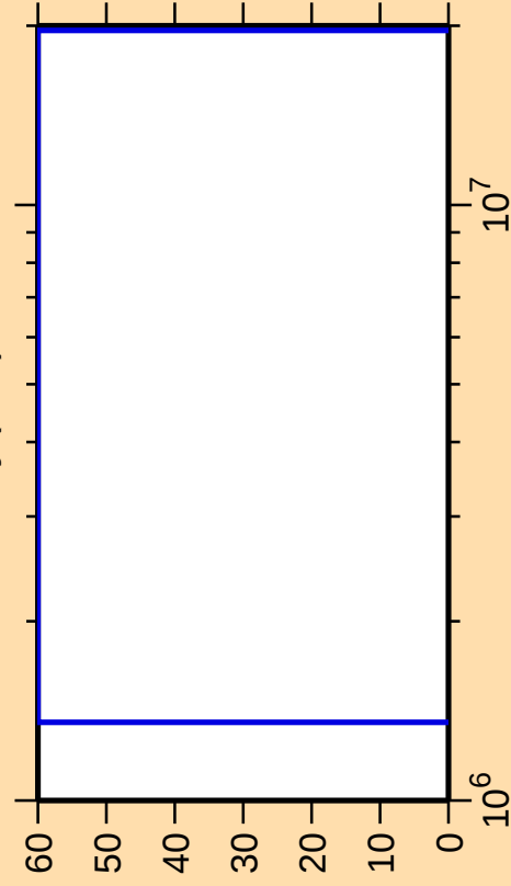
\Delta\sigma/\sigma vs. E for ^{151}\text{Dy}(n,\alpha)
