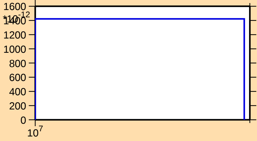
\sigma vs. E for ^{151}\text{Dy}(n,\text{pt})
