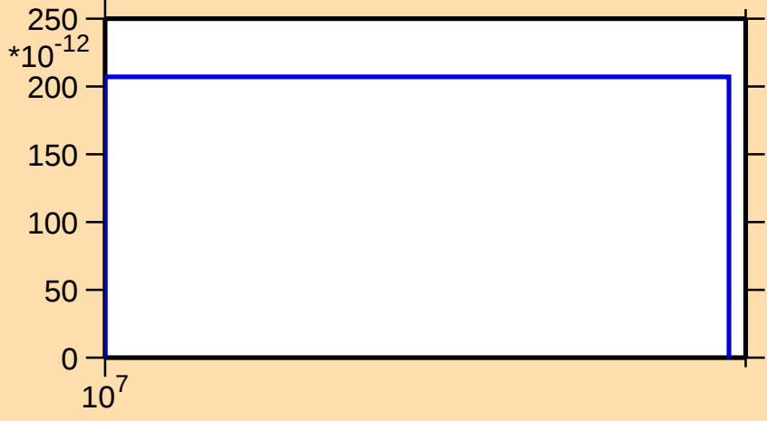
\sigma vs. E for ^{151}\text{Dy}(n,nt)
