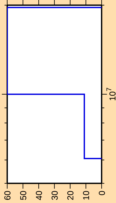
\Delta\sigma/\sigma vs. E for ^{151}\text{Dy}(n,n\text{cont.})
