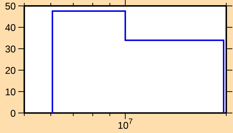
\Delta\sigma/\sigma vs. E for ^{151}\text{Dy}(n,2n)
