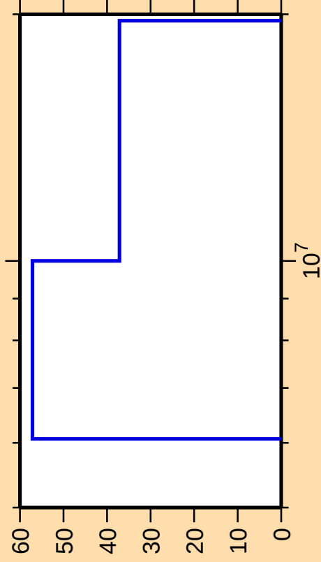
\Delta\sigma/\sigma vs. E for ^{151}\text{Dy}(n,p)
