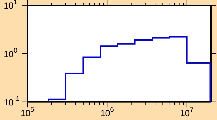
\sigma vs. E for ^{151}\text{Dy}(n,\text{inel.})
