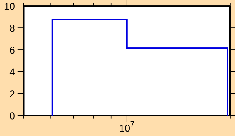
\Delta\sigma/\sigma vs. E for ^{151}\text{Dy}(n,\text{tot.})
