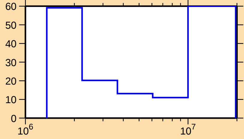
\Delta\sigma/\sigma vs. E for ^{151}\text{Dy}(n,n\text{cont.})
