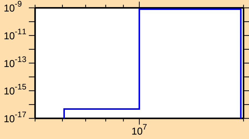
\sigma vs. E for ^{151}\text{Dy}(\text{mt117})
