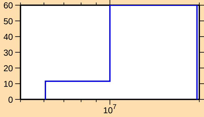
\Delta\sigma/\sigma vs. E for ^{151}\text{Dy}(n,\text{inel.})
