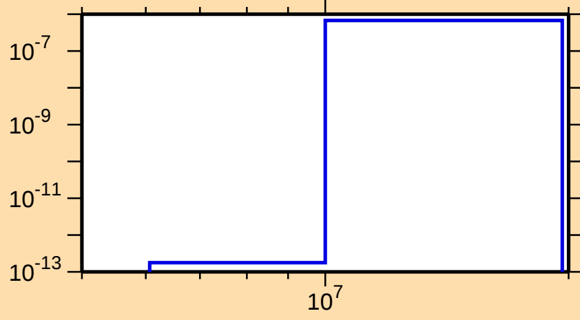
\sigma vs. E for ^{151}\text{Dy}(n,\text{He}3)
