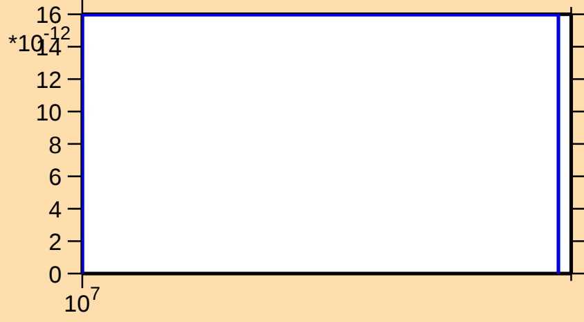
\sigma vs. E for ^{151}\text{Dy}(\text{mt } 34)
