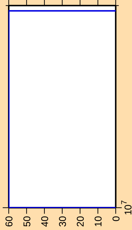
\Delta\sigma/\sigma vs. E for ^{151}\text{Dy}(\text{mt } 34)
