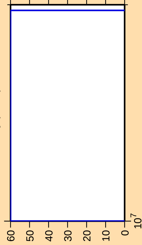
\Delta\sigma/\sigma vs. E for ^{151}\text{Dy}(n,\text{nd})
