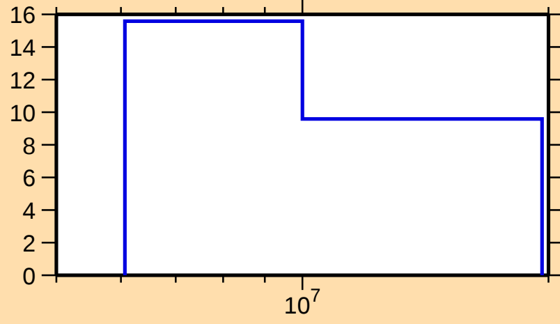
\Delta\sigma/\sigma vs. E for ^{151}\text{Dy}(n,\text{el.})
