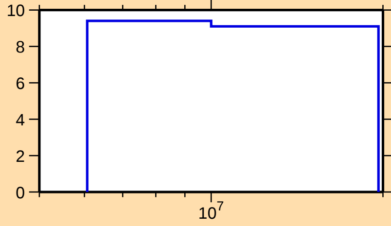
\Delta\sigma/\sigma vs. E for ^{151}\text{Dy}(n,\text{nonel.})
