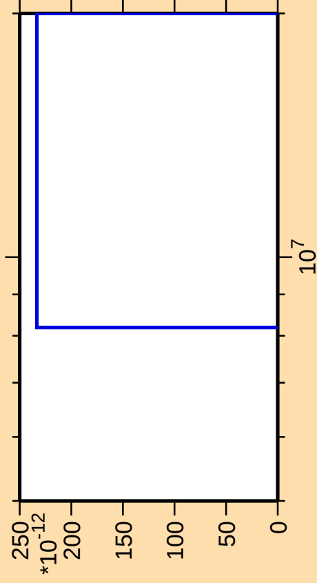
\Delta\sigma/\sigma vs. E for ^{151}\text{Dy}(\text{mt } 11)
