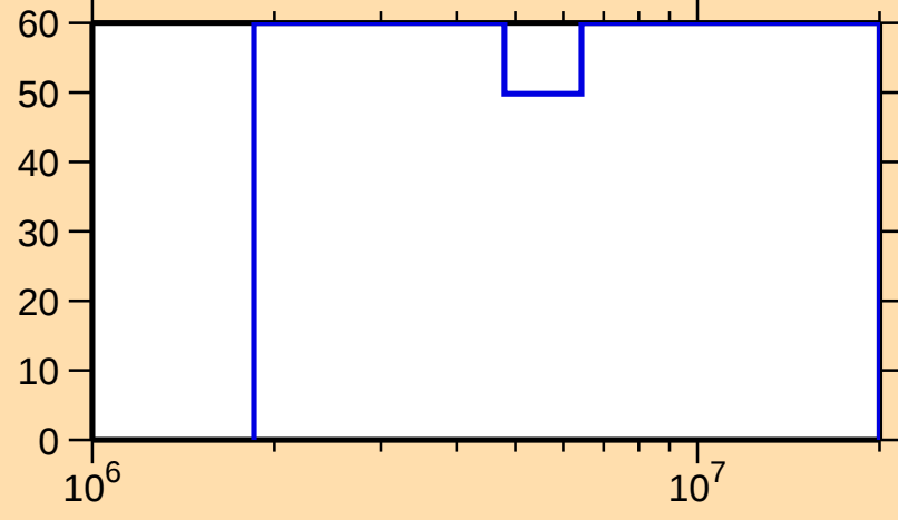
\Delta\sigma/\sigma vs. E for ^{151}\text{Dy}(n,n_1)
