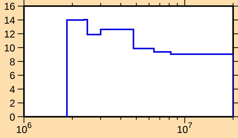
\Delta\sigma/\sigma vs. E for ^{151}\text{Dy}(n,n\text{nonel.})
