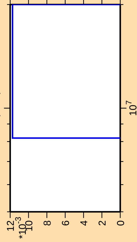
\Delta\sigma/\sigma vs. E for ^{151}\text{Er}(n,\text{nt})
