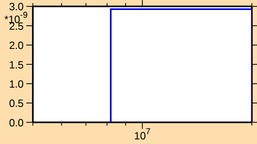
\sigma vs. E for ^{151}\text{Er}(\text{mt117})
