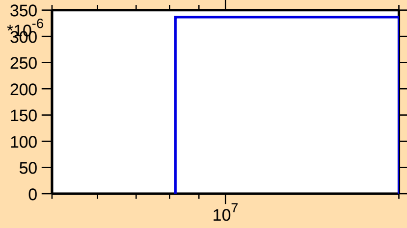
\sigma vs. E for ^{151}\text{Er}(n,2np)
