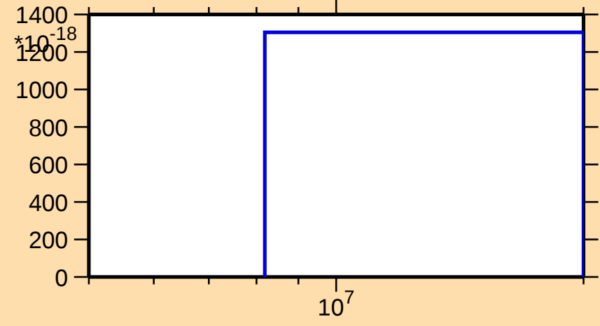
\sigma vs. E for ^{151}\text{Er}(n,\text{nt})
