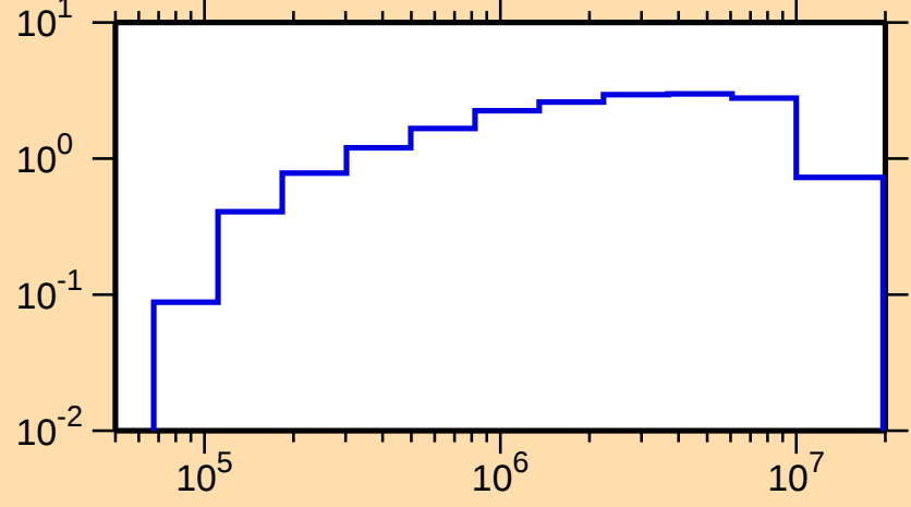
\sigma vs. E for ^{166}\text{Er}(n,\text{inel.})
