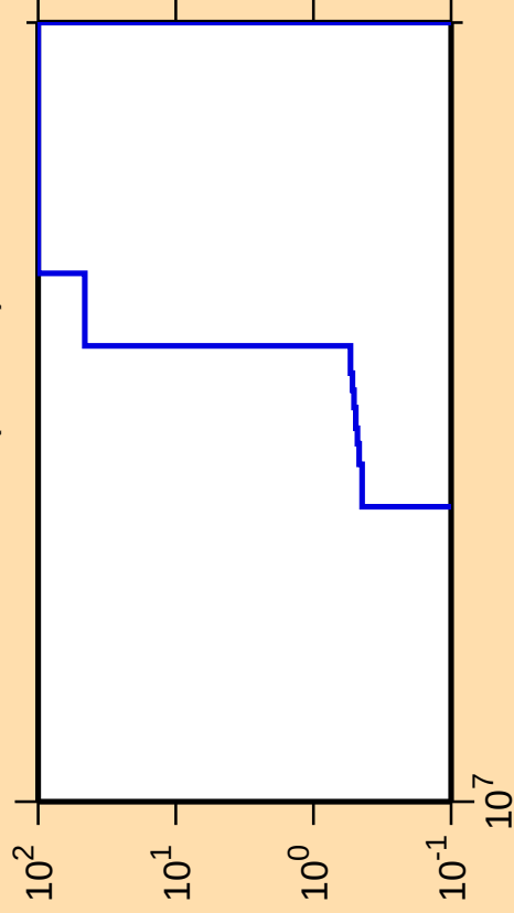
\Delta\sigma/\sigma vs. E for ^{248}\text{Es}(n,3n\alpha)
