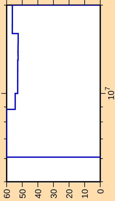
\Delta\sigma/\sigma vs. E for ^{248}\text{Es}(n,p)
