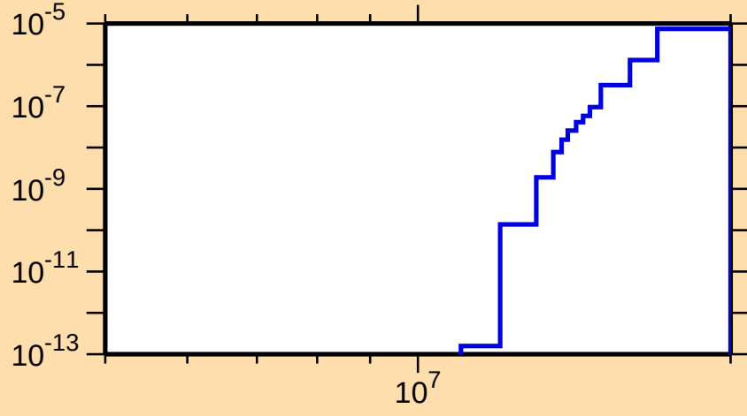
\sigma vs. E for ^{248}\text{Es}(n,2np)
