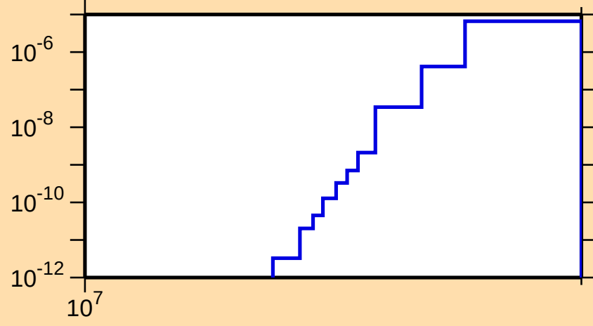
\sigma vs. E for ^{248}\text{Es}(n,nt)
