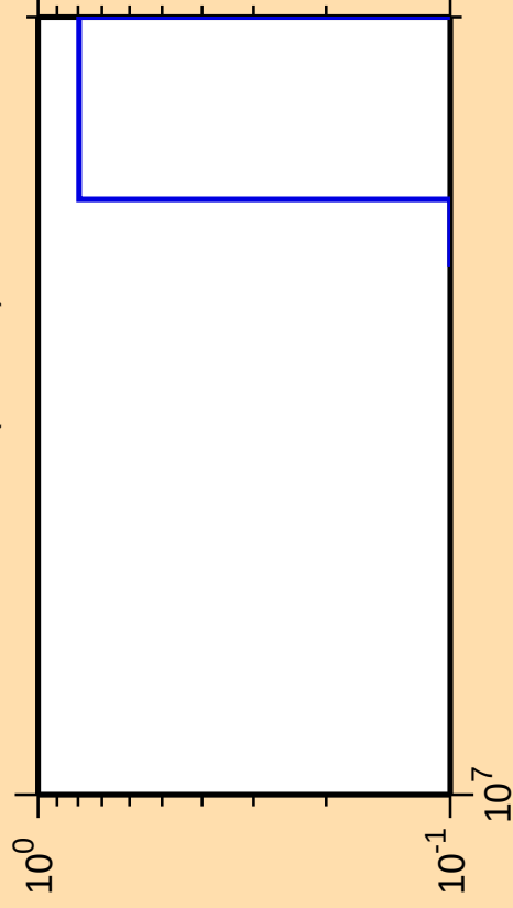
\Delta\sigma/\sigma vs. E for ^{248}\text{Es} (mt 11)
