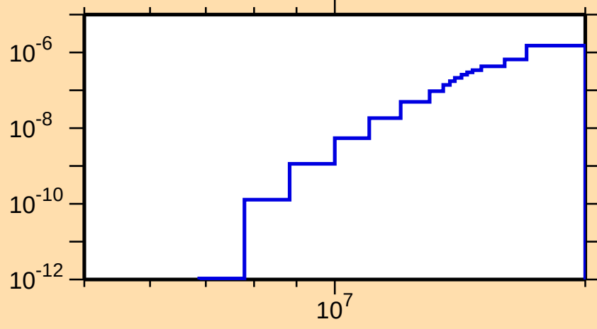
\sigma vs. E for ^{248}\text{Es}(n,2n\alpha)
