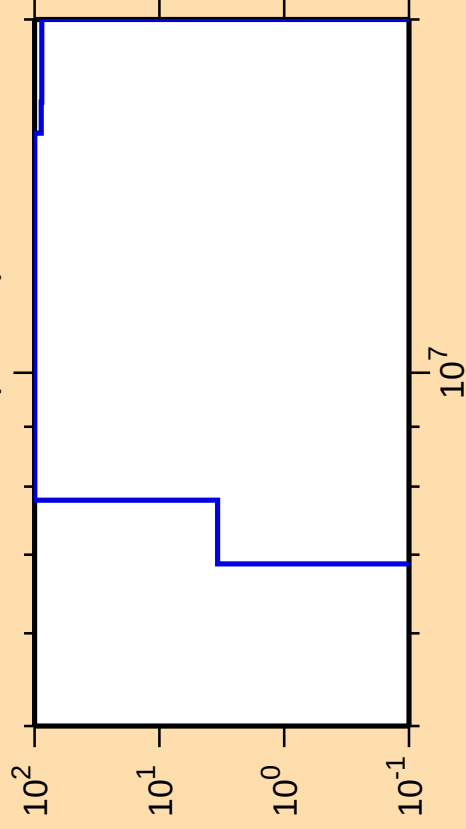
\Delta\sigma/\sigma vs. E for ^{248}\text{Es}(n,2n\alpha)
