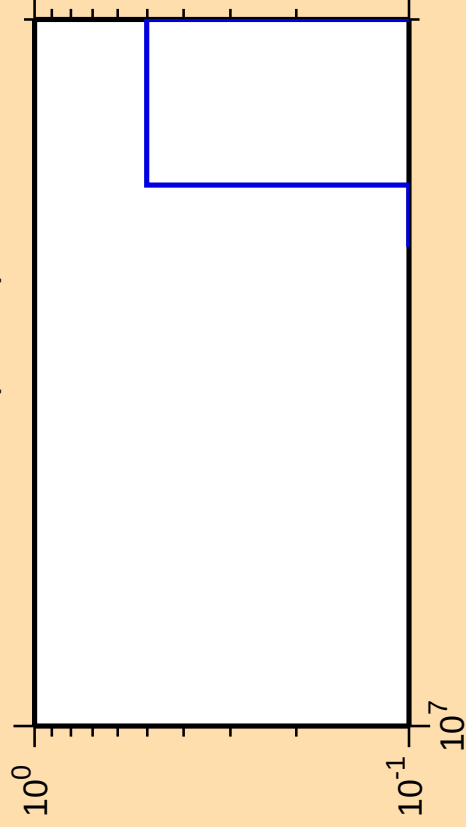
\Delta\sigma/\sigma vs. E for ^{248}\text{Es} (mt 42)
