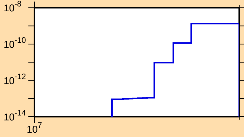
\sigma vs. E for ^{248}\text{Es}(n,3n\alpha)
