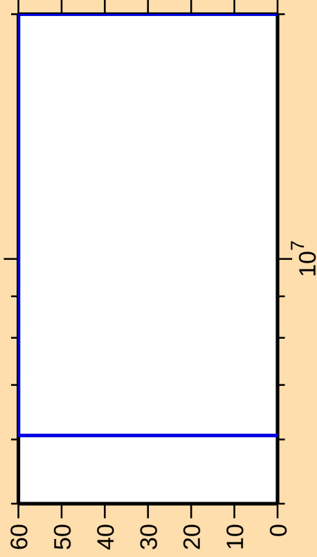
\Delta\sigma/\sigma vs. E for ^{248}\text{Es}(n,\alpha)
