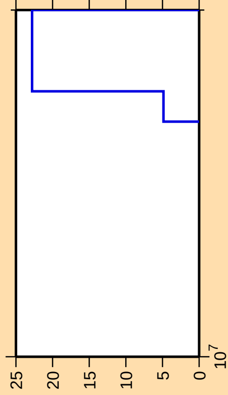
\Delta\sigma/\sigma vs. E for ^{248}\text{Es}(\text{mt117})
