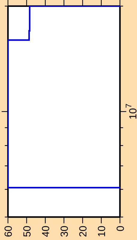
\Delta\sigma/\sigma vs. E for ^{248}\text{Es}(n,f)
