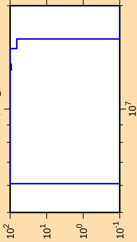
\Delta\sigma/\sigma vs. E for ^{248}\text{Es}(n,n_1)
