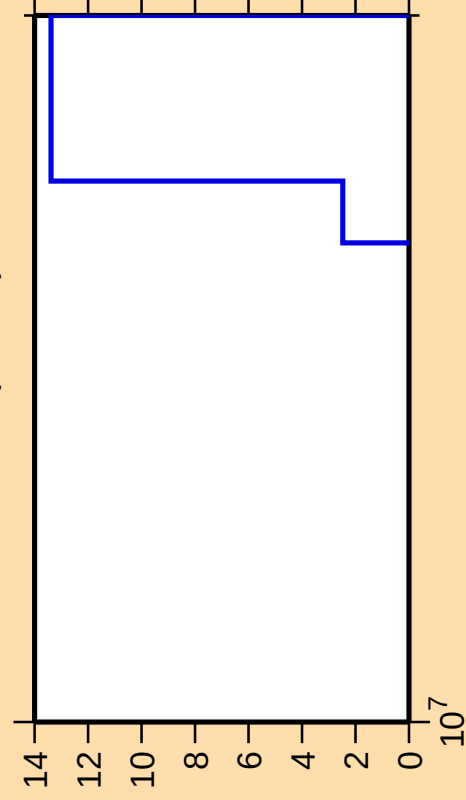
\Delta\sigma/\sigma vs. E for ^{248}\text{Es}(\text{mt } 45)
