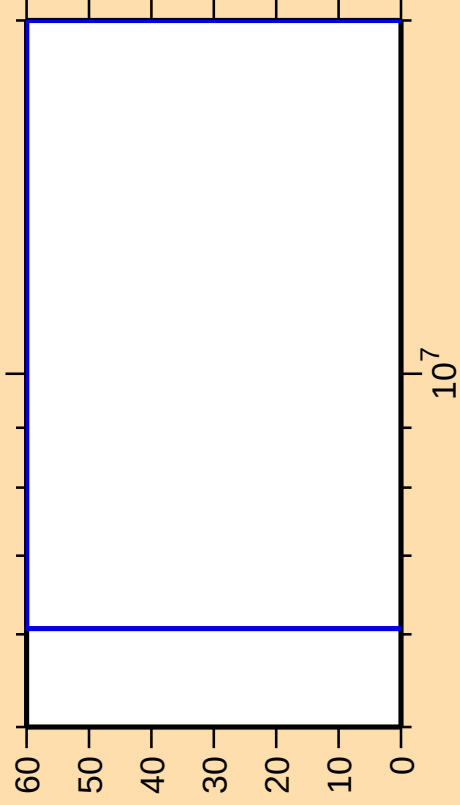
\Delta\sigma/\sigma vs. E for ^{248}\text{Es}(n,\gamma)
