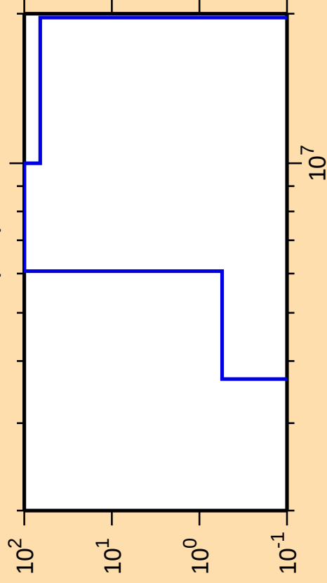
\Delta\sigma/\sigma vs. E for ^{248}\text{Es}(n,d)
