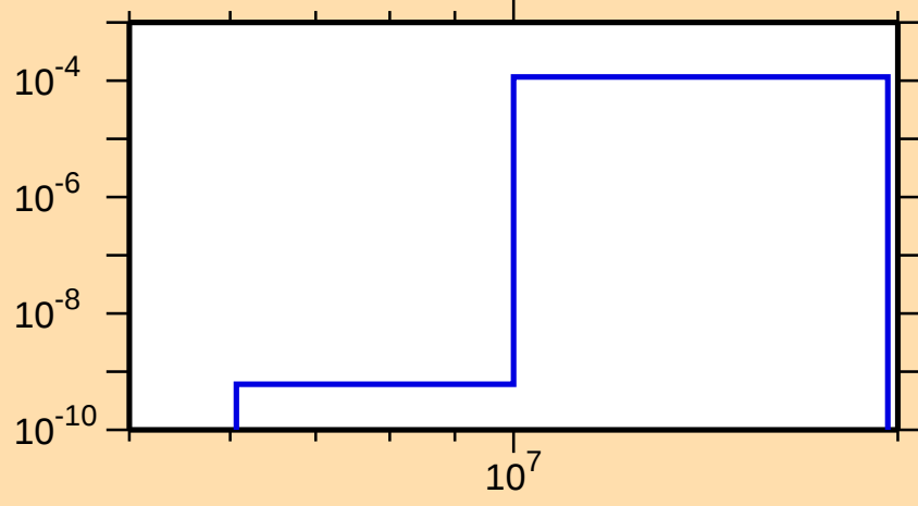
\sigma vs. E for ^{248}\text{Es}(n,t)
