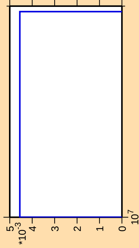
\Delta\sigma/\sigma vs. E for ^{248}\text{Es}(\text{mt 11})
