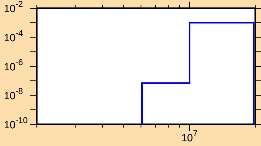
\sigma vs. E for ^{248}\text{Es}(n,d)
