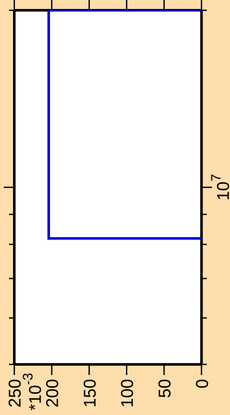
\Delta\sigma/\sigma vs. E for ^{248}\text{Es}(\text{mt } 45)
