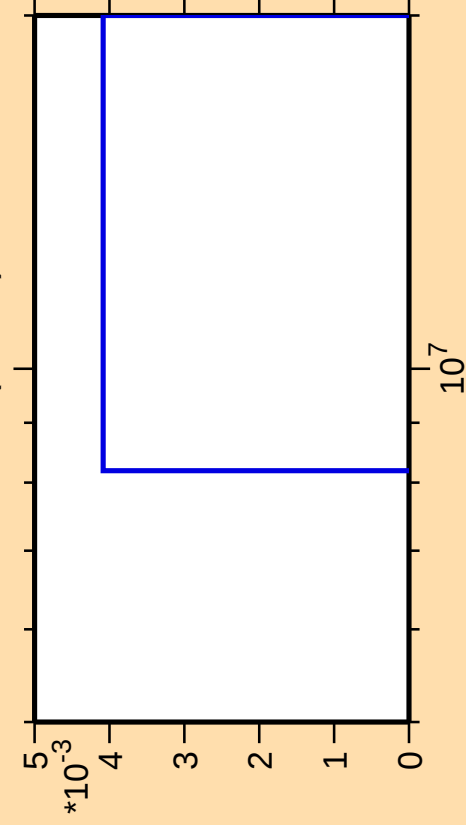
\Delta\sigma/\sigma vs. E for ^{248}\text{Es}(\text{mt } 42)
