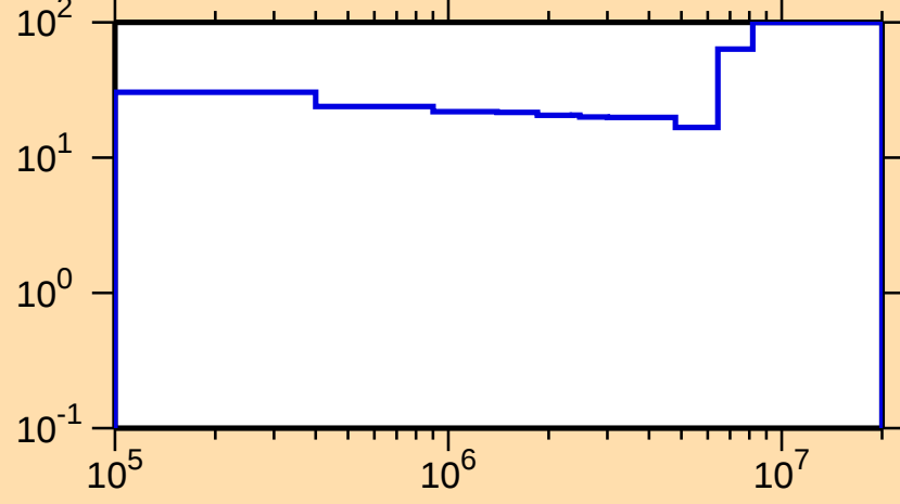
\Delta\sigma/\sigma vs. E for ^{248}\text{Es}(n,\text{inel.})
