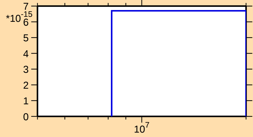
\sigma vs. E for ^{248}\text{Es}(\text{mt 11})
