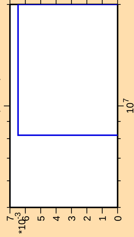
\Delta\sigma/\sigma vs. E for ^{248}\text{Es}(\text{mt 11})
