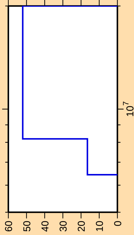
\Delta\sigma/\sigma vs. E for ^{248}\text{Es}(n,t)
