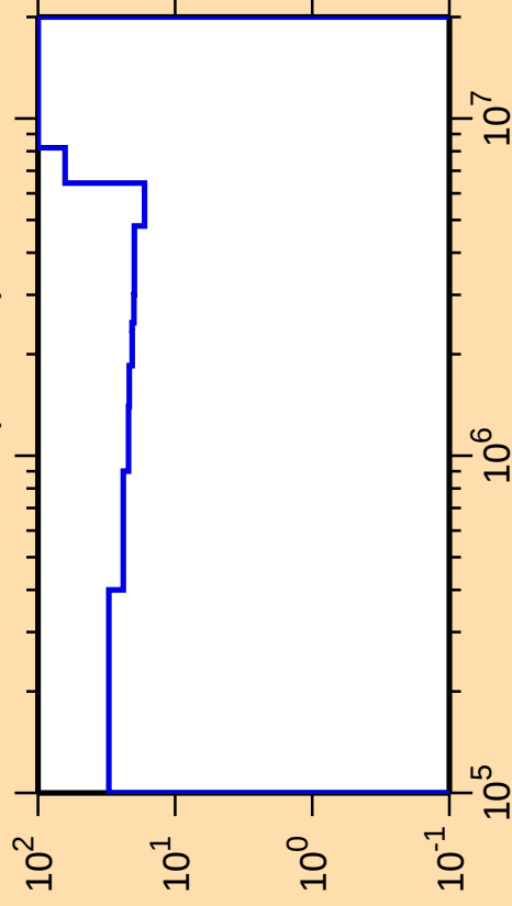
\Delta\sigma/\sigma vs. E for ^{248}\text{Es}(n,\text{inel.})
