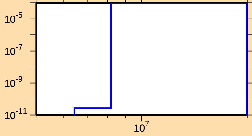
\sigma vs. E for ^{248}\text{Es}(n,t)
