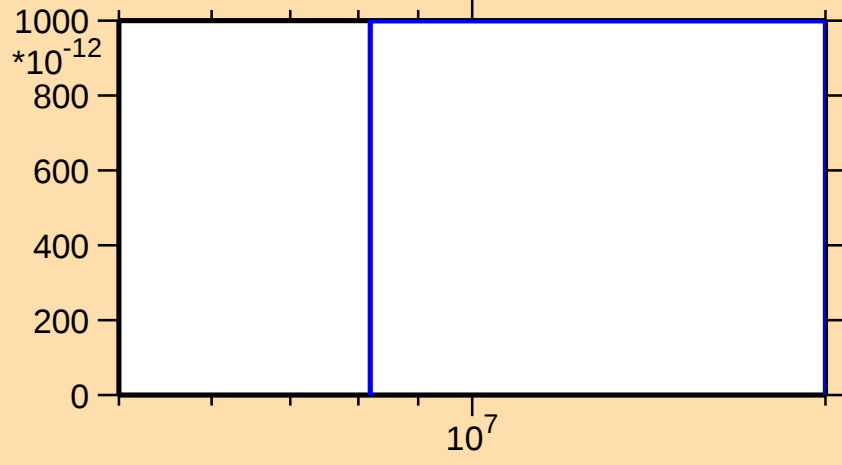
\sigma vs. E for ^{136}\text{Eu}(n,2n\alpha)
