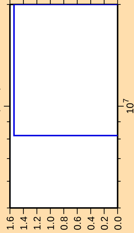
\Delta\sigma/\sigma vs. E for ^{136}\text{Eu}(n,nt)
