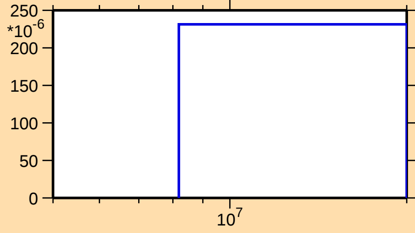
\sigma vs. E for ^{136}\text{Eu}(n,2np)
