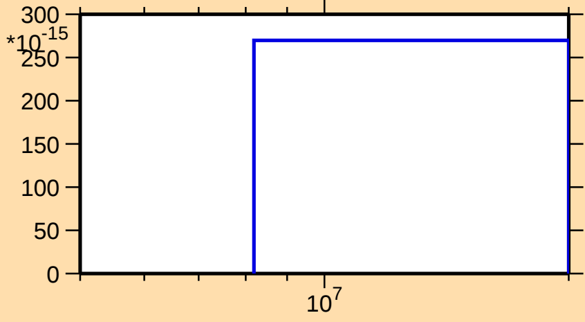
\sigma vs. E for ^{136}\text{Eu}(n,nt)
