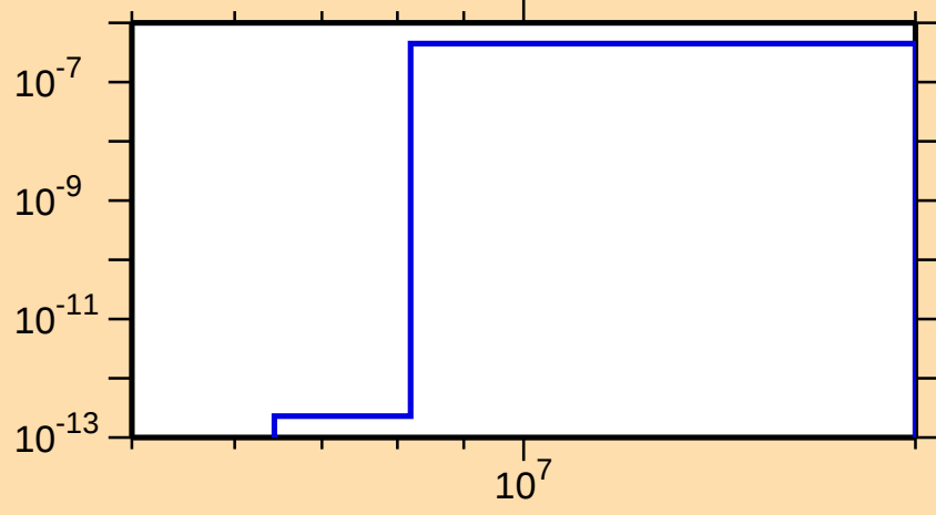
\sigma vs. E for ^{136}\text{Eu}(\text{mt117})
