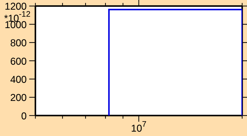
\sigma vs. E for ^{136}\text{Eu}(\text{mt } 34)
