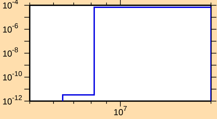
\sigma vs. E for ^{136}\text{Eu}(\text{mt } 45)
